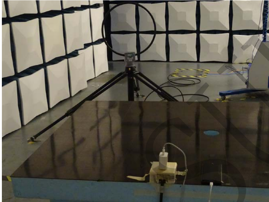
Radiated Disturbance Emissions (9Khz-30Mhz)
