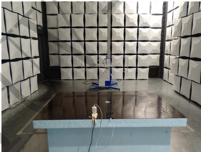
Radiated Disturbance Emissions (30Mhz-1GHz)
