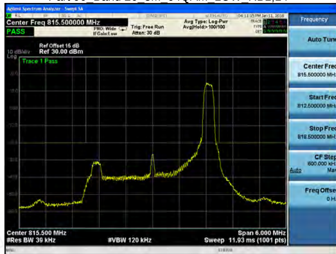
Part 90 Band 26 3M 64QAM LOW RB15,0
