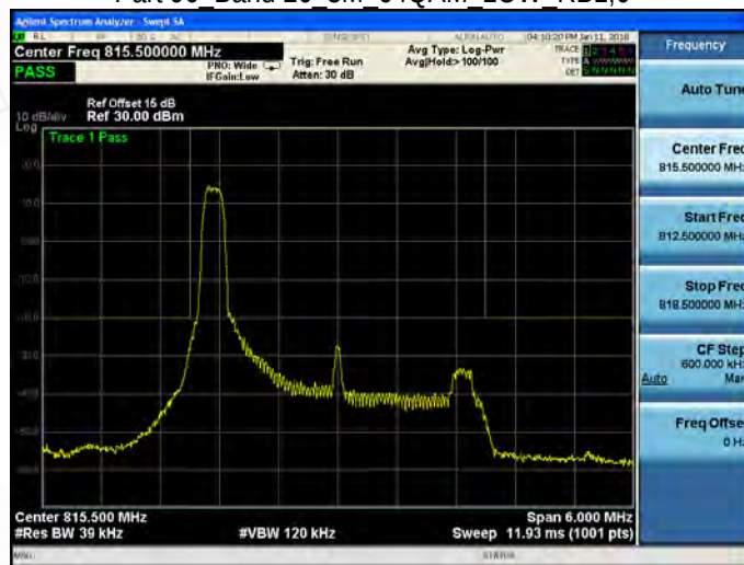
Part 90 Band 26 3M 64QAM LOW RB1,14
