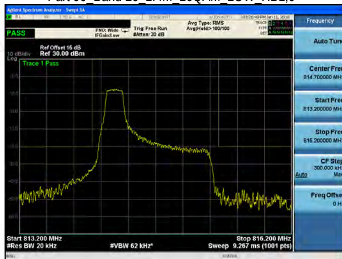
Part 90 Band 26 1.4M 16QAM LOW RB1,5
