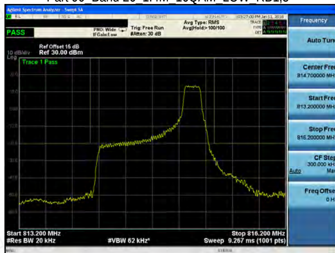
Part 90 Band 26 1.4M 16QAM LOW RB6,0
