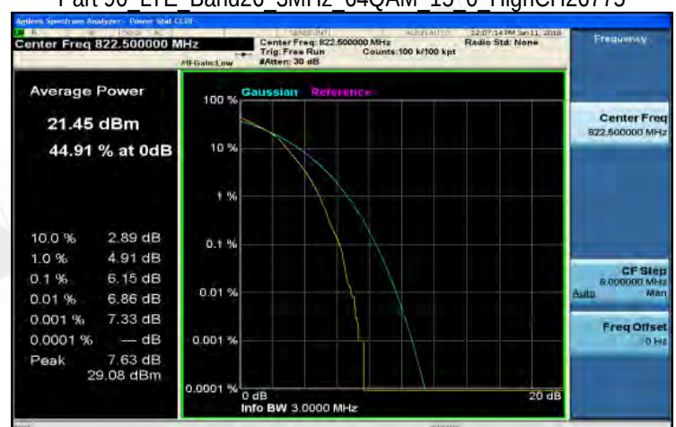
Part 90 LTE Band26 3MHz 64QAM 15 0 HighCH26775
