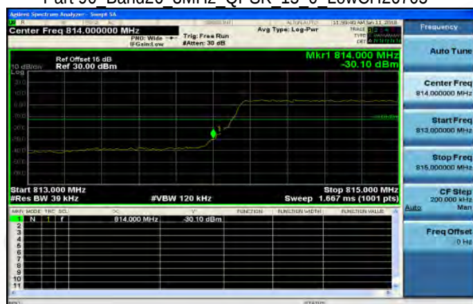
Part 90 Band26 3MHz QPSK 15 0 LowCH26705
