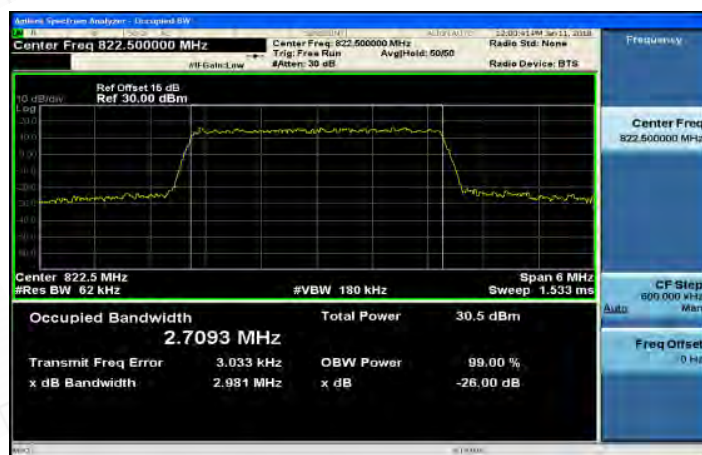
Part 90_Band26_3MHz_QPSK_15_0_HighCH26775
