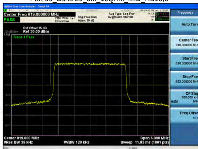
Part 90 Band 26 3M 16QAM MID RB15,0
