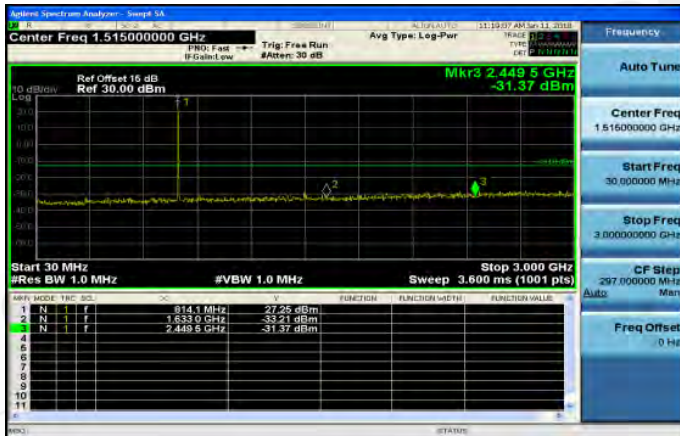
30MHz~3GHz_Band26_5MHz_QPSK_1_0_LowCH26715
