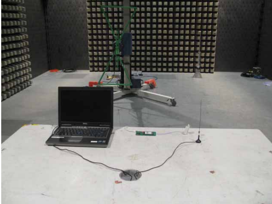
Radiated Disturbance
