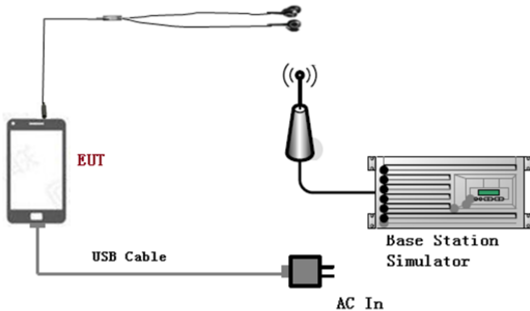
Connection Diagram (Mode 2~3)
