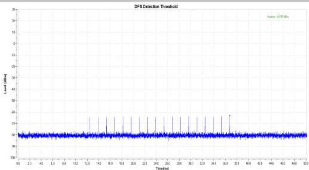
11AC160MIMO_5570_Type0
