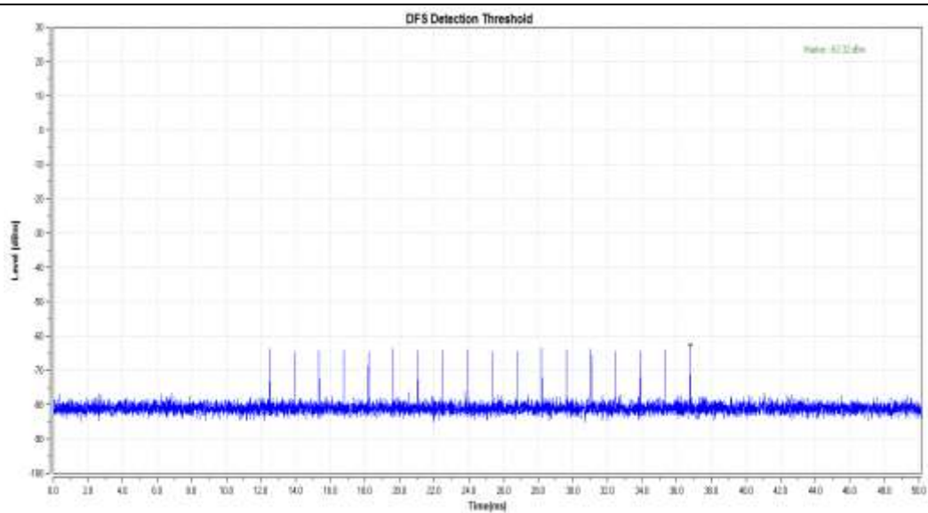
11A CDD_5640_Type0
