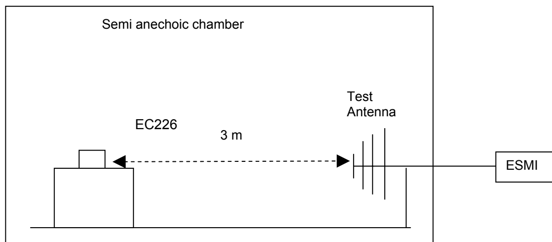
Figure 14. Test set up
