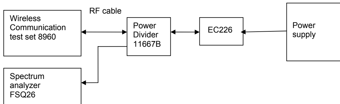
Figure 6. Test Set-up
