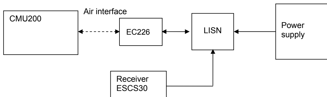
Figure 13. Test Set-up
