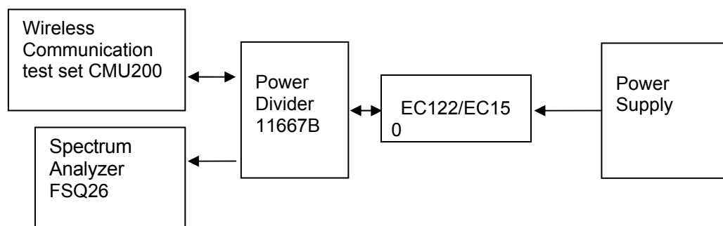
Figure 4. Test Set-up
