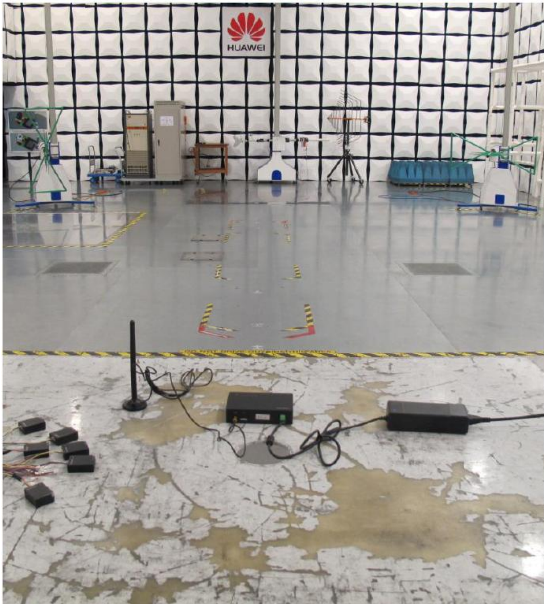
Radiated emission for 30 MHz-1 GHz
