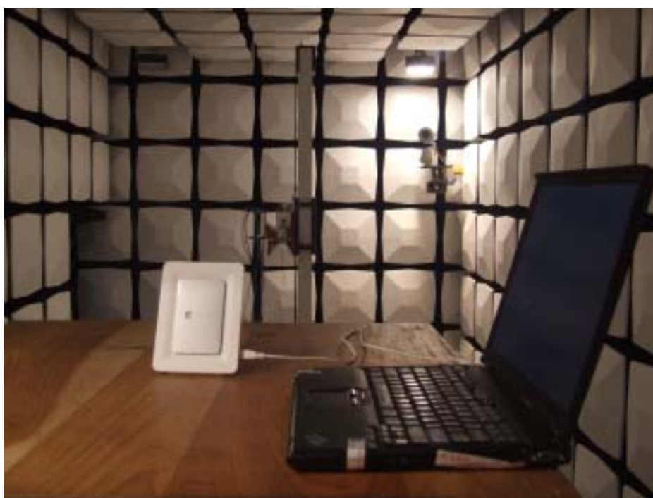
Radiated Spurious Emission (2GHz~18GHz, Modem mode)
