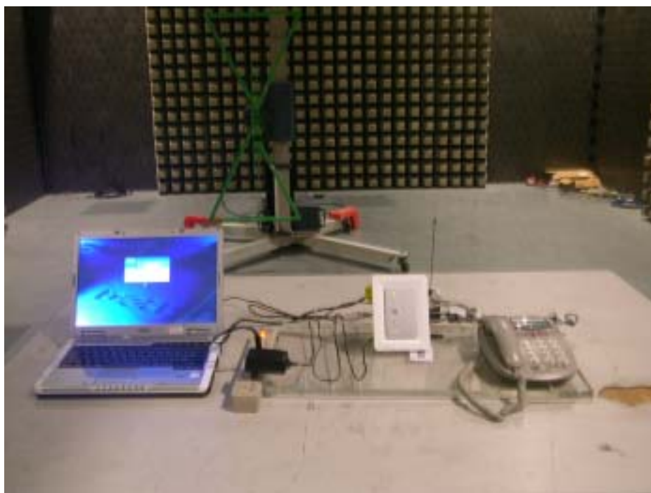
Radiated Disturbance ( gateway mode )
