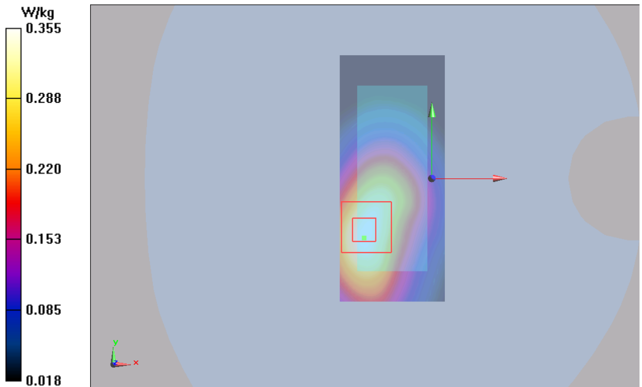
Figure 85 LTE Band 5 with Test Position 1 Channel 20600
