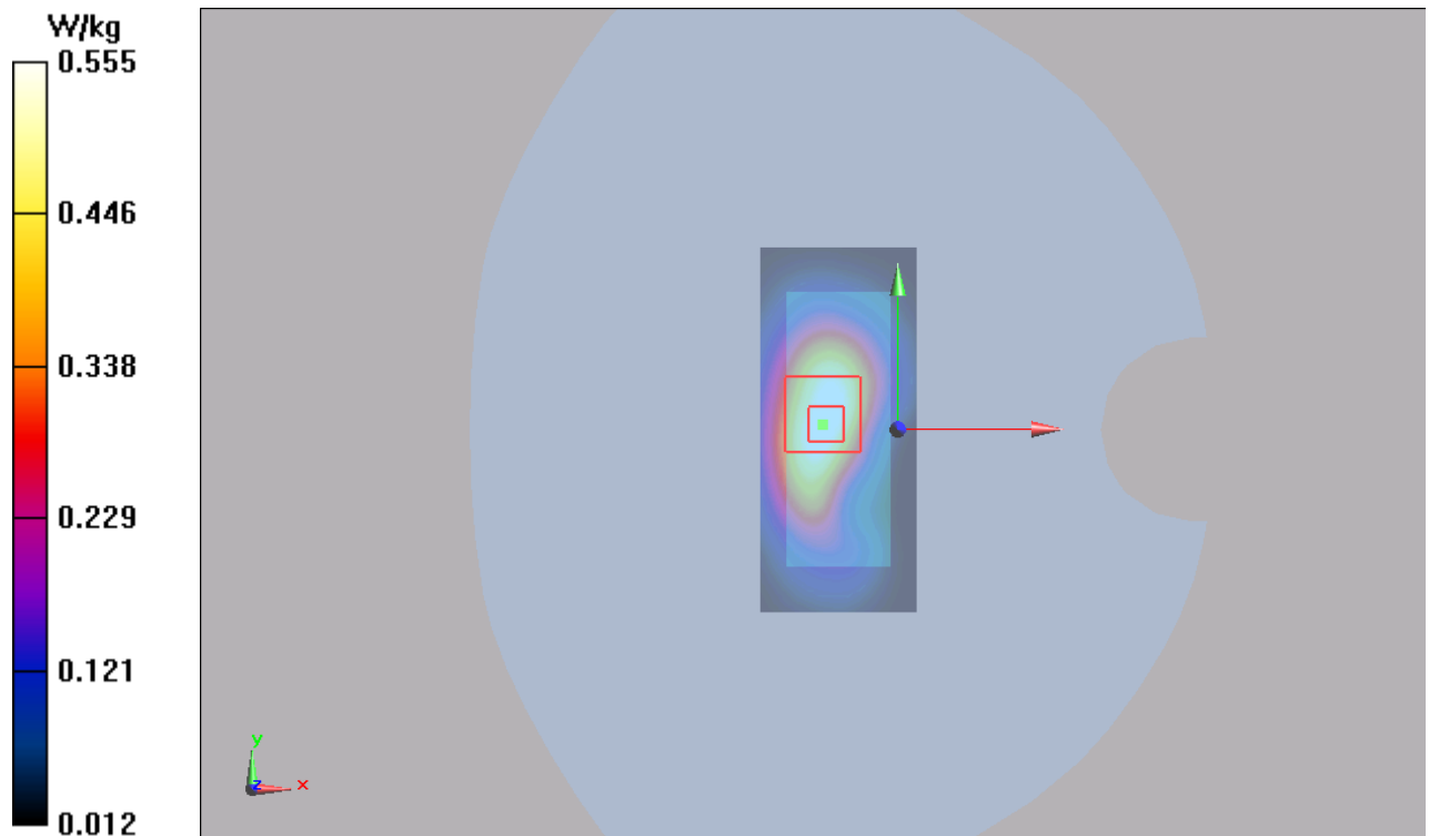
Figure 48 LTE Band 2 with Test Position 1 Channel 18700
