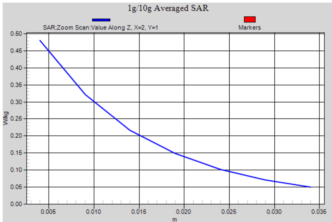
Figure 95 UMTS Band V with Test Position 1 Channel 4233
