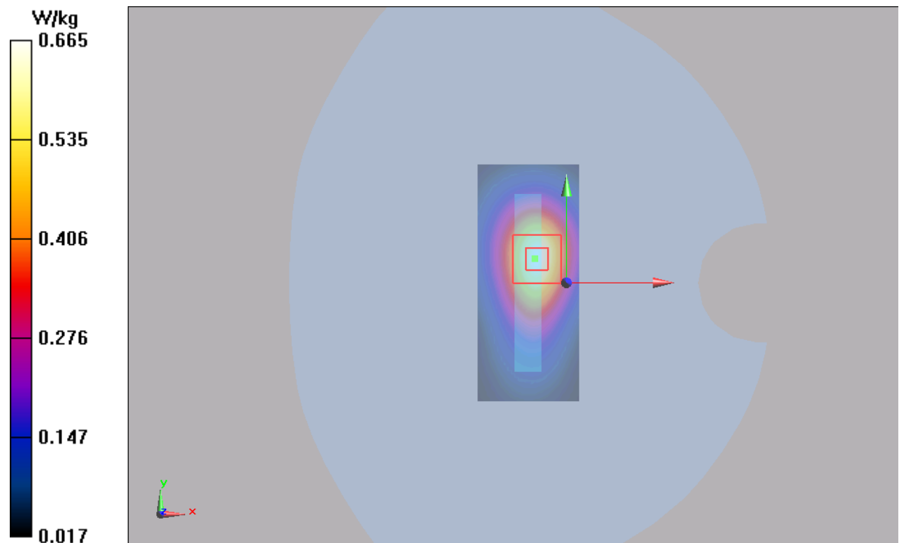
Figure 64 LTE Band 2 with Test Position 3 Channel 18900
