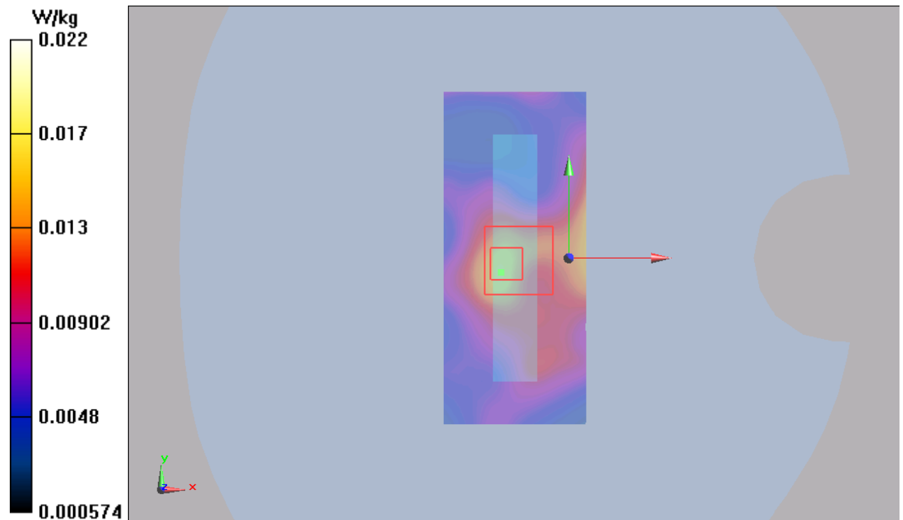
Figure 127 802.11b Test Position 3 Channel 6
