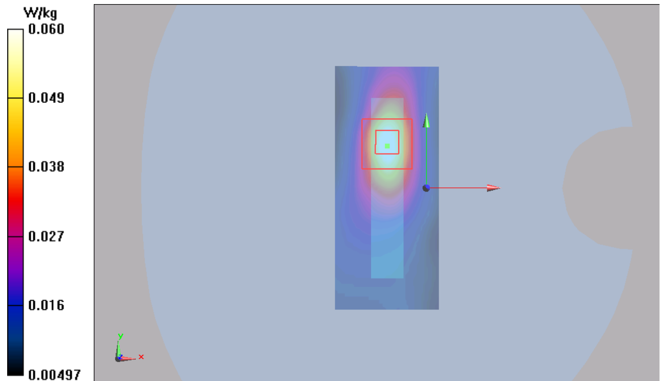
Figure 110 LTE Band 12 with Test Position 4 Channel 23060
