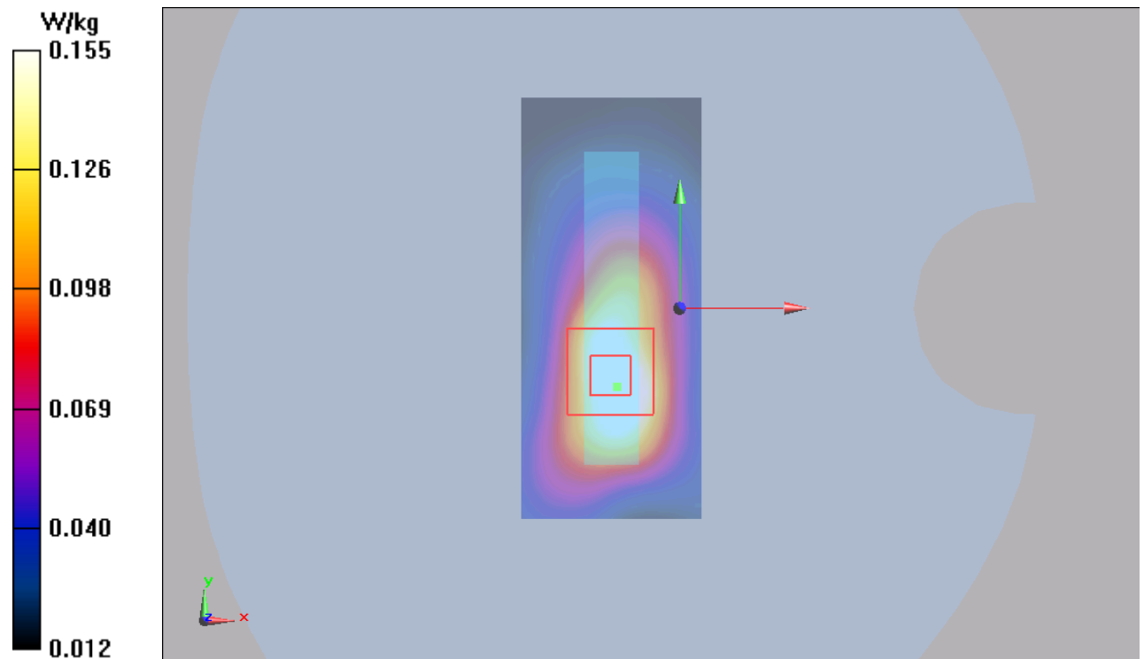
Figure 103 LTE Band 12 with Test Position 3 Channel 23060
