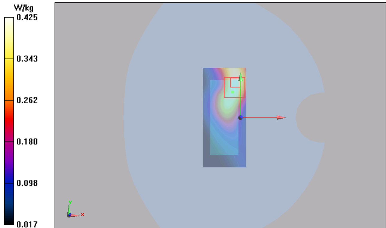
Figure 80 LTE Band 5 with Test Position 1 Channel 20525
