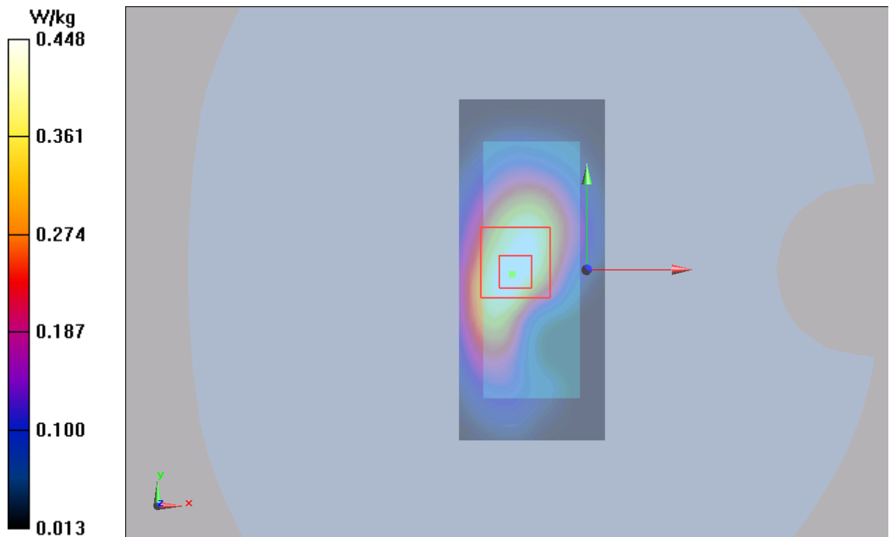
Figure 36 UMTS Band IV with Test Position 1 Channel 1312
