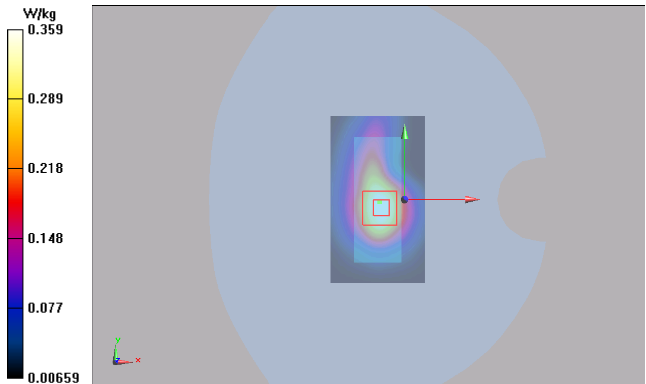
Figure 75 LTE Band 4 with Test Position 2 Channel 20175
