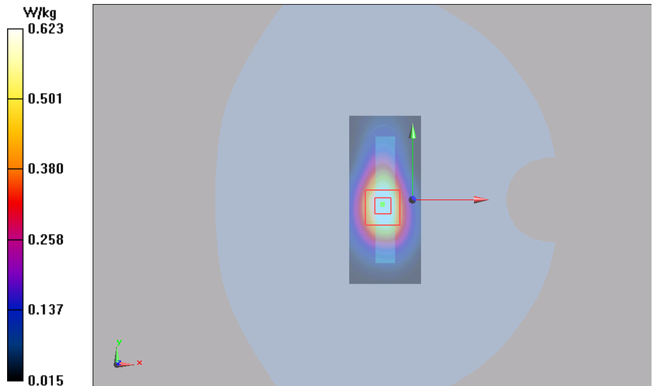
Figure 70 LTE Band 4 with Test Position 3 Channel 20050
