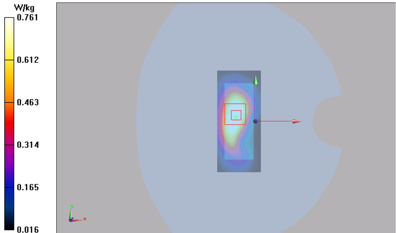
Figure 57 LTE Band 2 with Test Position 1 Channel 18900
