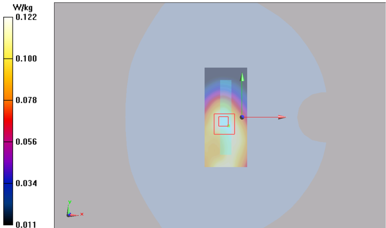
Figure 84 LTE Band 5 with Test Position 4 Channel 20525
