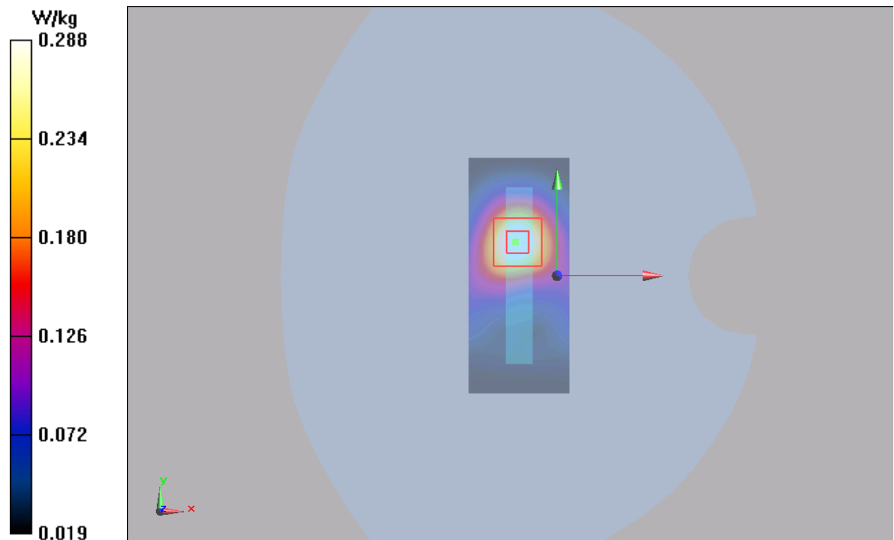
Figure 55 LTE Band 2 with Test Position 4 Channel 18900
