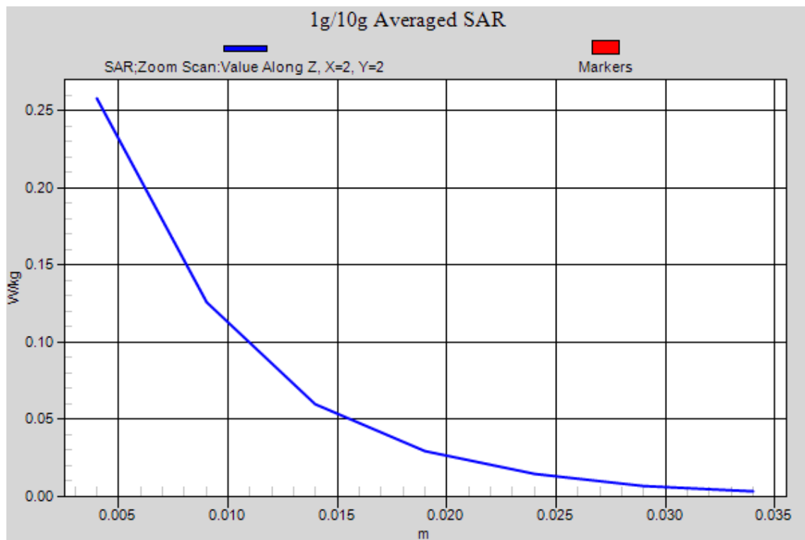
Figure 132 802.11b Test Position 3 Channel 6
