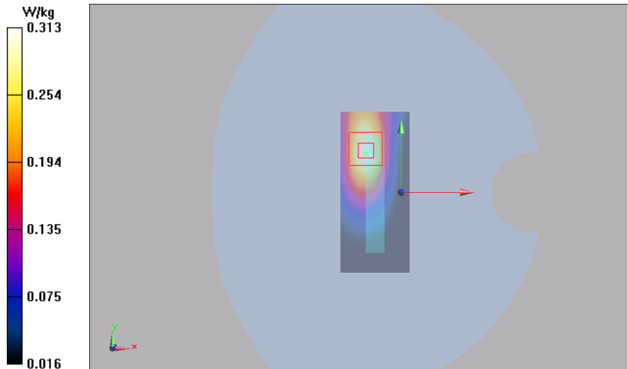
Figure 83 LTE Band 5 with Test Position 3 Channel 20525
