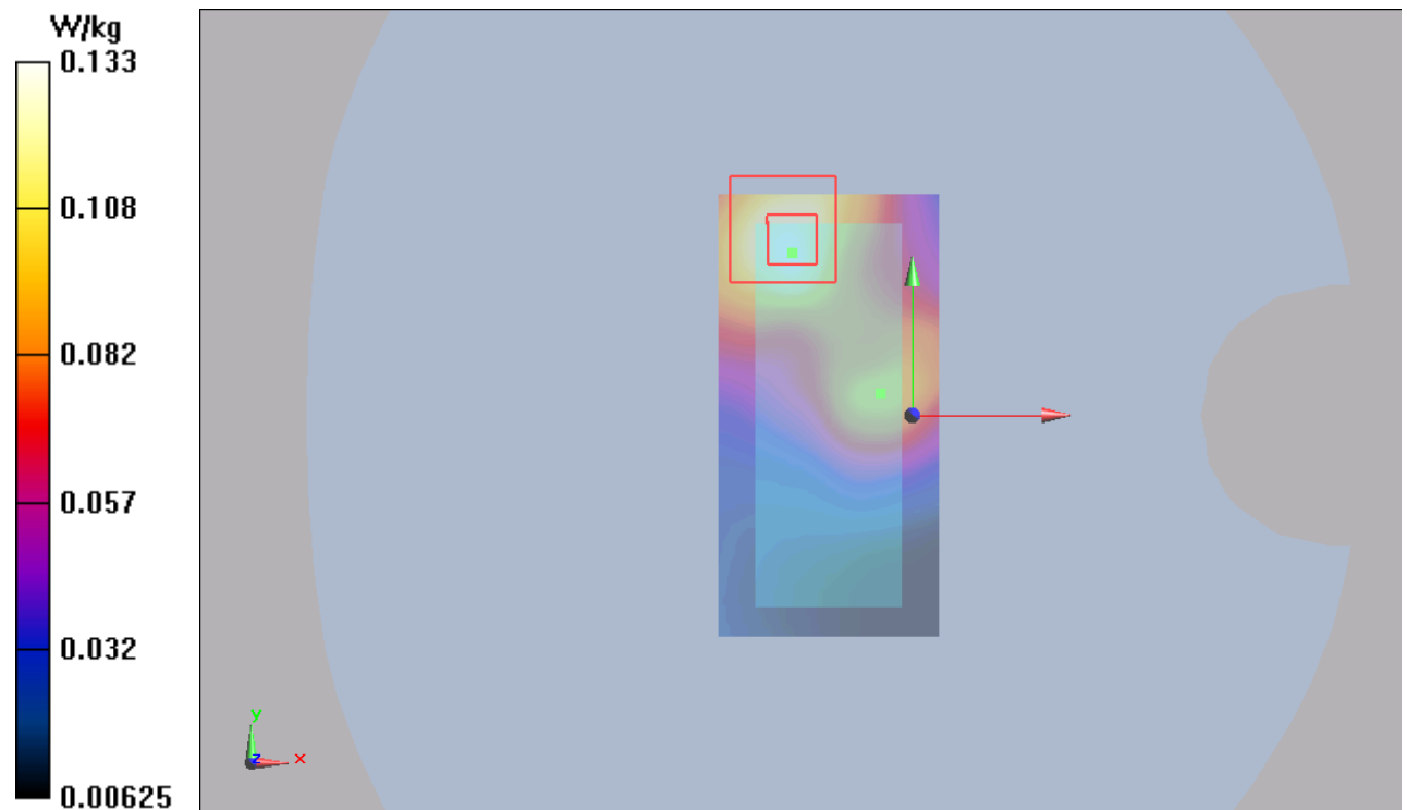
Figure 108 LTE Band 12 with Test Position 2 Channel 23060
