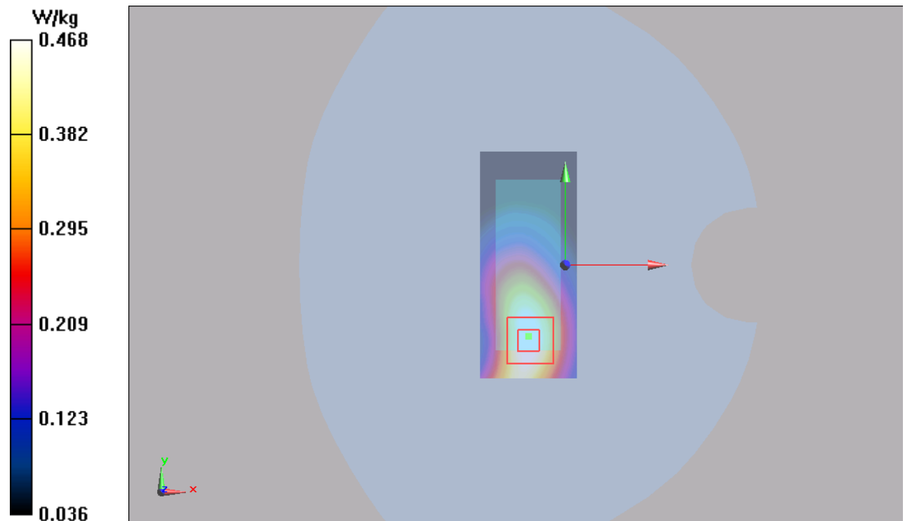
Figure 43 UMTS Band V with Test Position 2 Channel 4182
