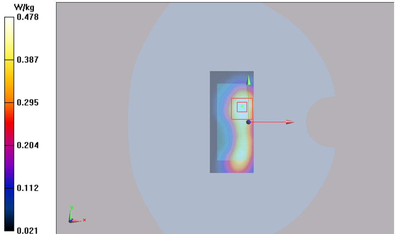
Figure 49 LTE Band 2 with Test Position 2 Channel 19100
