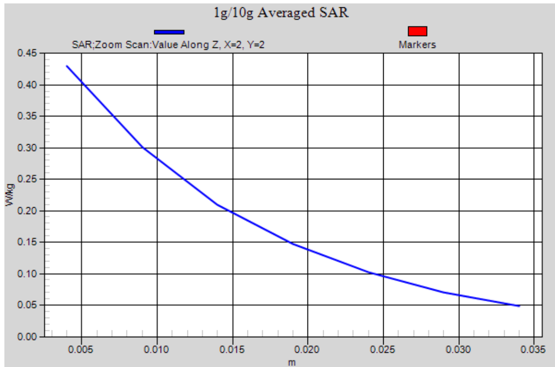
Figure 81 LTE Band 5 with Test Position 1 Channel 20450
