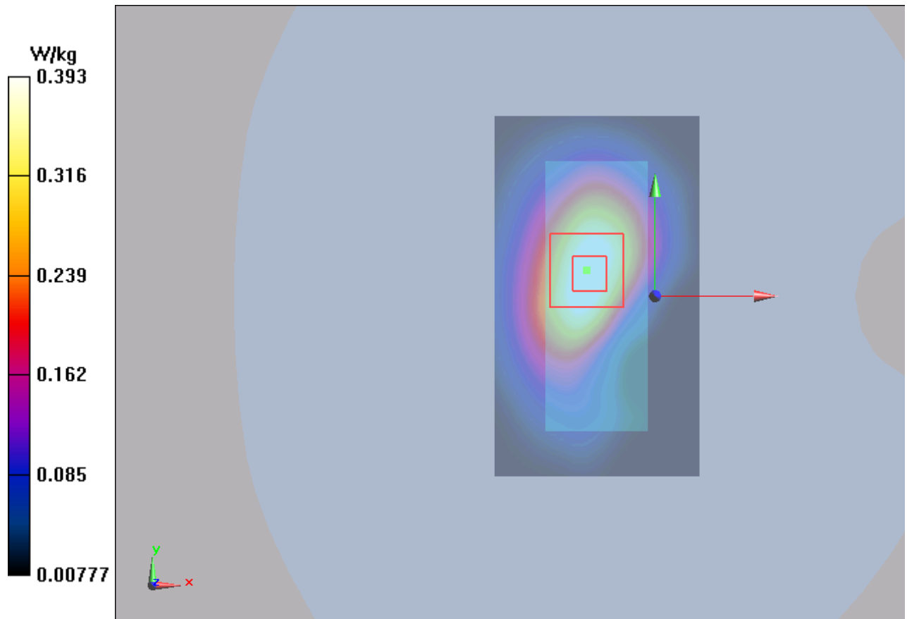
Figure 72 LTE Band 4 with Test Position 1 Channel 20300
