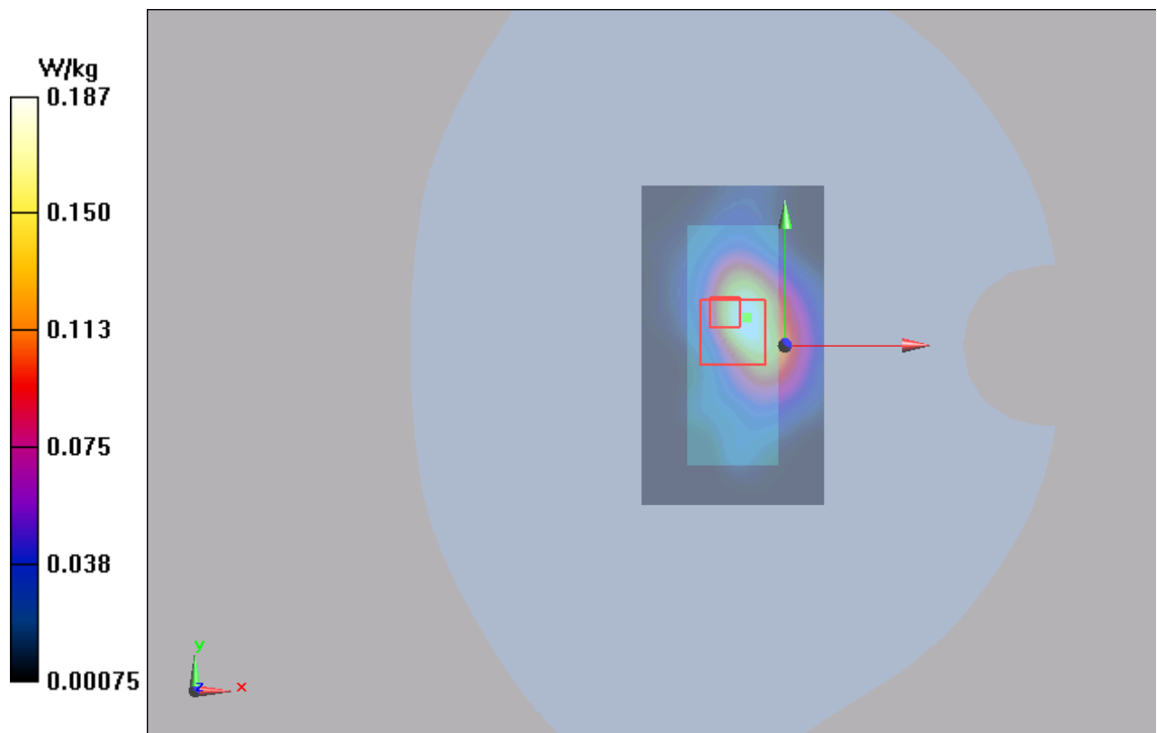
Figure 124 802.11b Test Position 2 Channel 11
