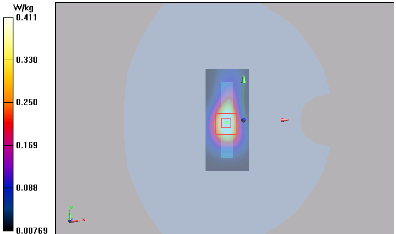
Figure 76 LTE Band 4 with Test Position 3 Channel 20175
