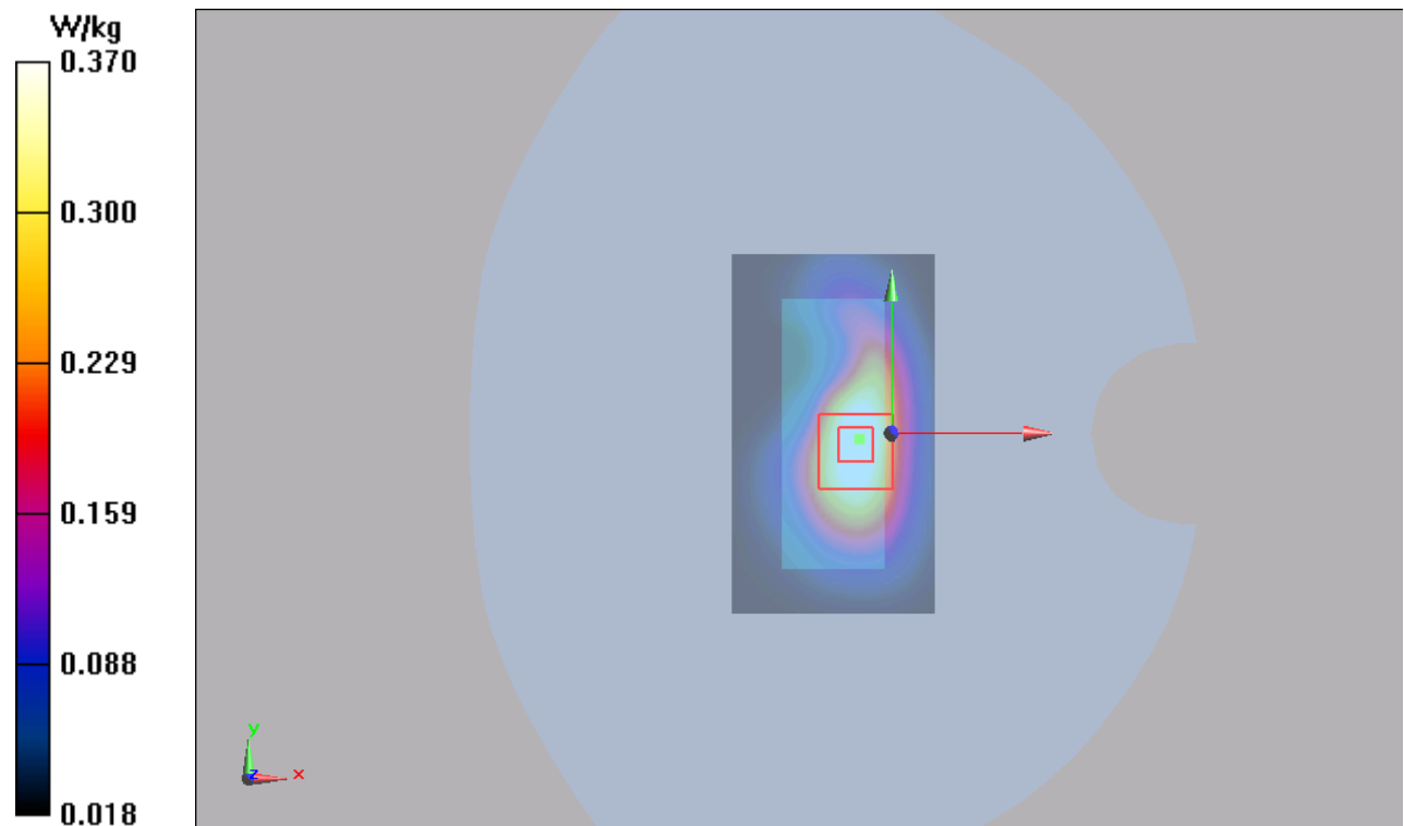
Figure 82 LTE Band 5 with Test Position 2 Channel 20525
