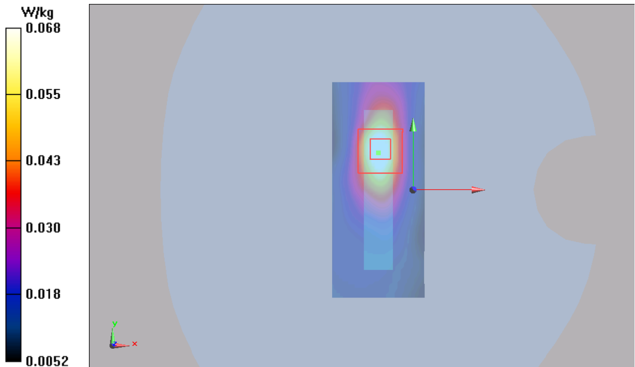
Figure 122 LTE Band 17 with Test Position 4 Channel 23780
