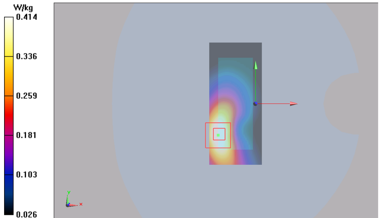
Figure 20 GSM 850 EGPRS (2TXslots) with Test Position 1 Channel 128
