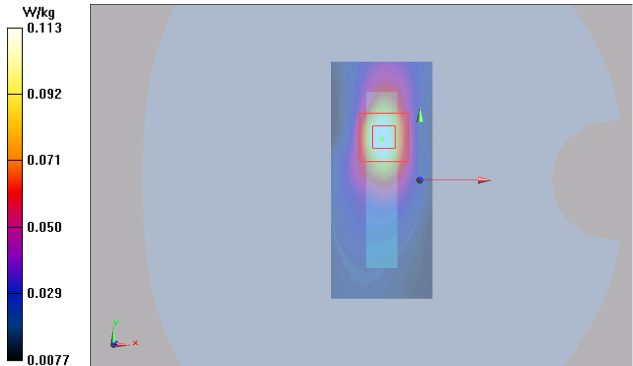
Figure 116 LTE Band 17 with Test Position 4 Channel 23780
