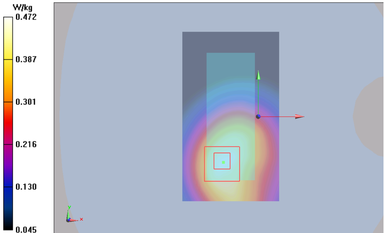
Figure 101 LTE Band 12 with Test Position 1 Channel 23060
