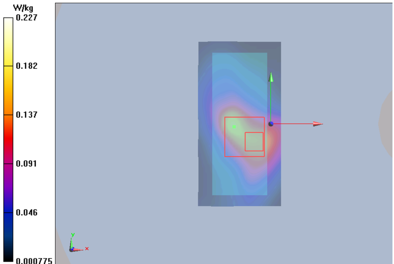
Figure 129 802.11b Test Position 1 Channel 1
