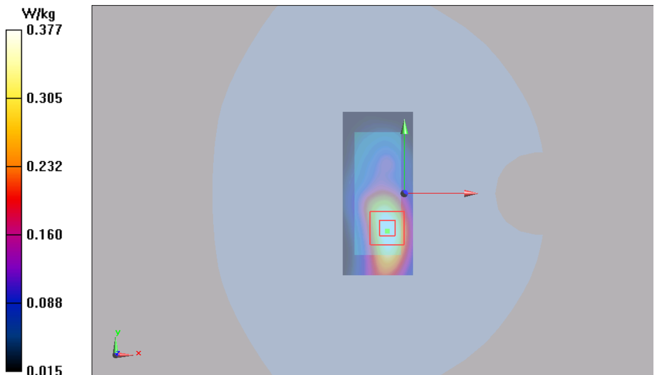
Figure 24 GSM 1900 GPRS (2TXslots) with Test Position 2 Channel 661
