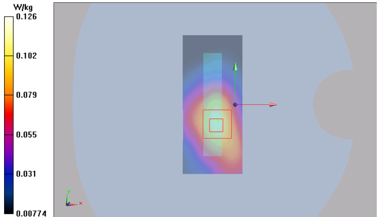
Figure 115 LTE Band 17 with Test Position 3 Channel 23780
