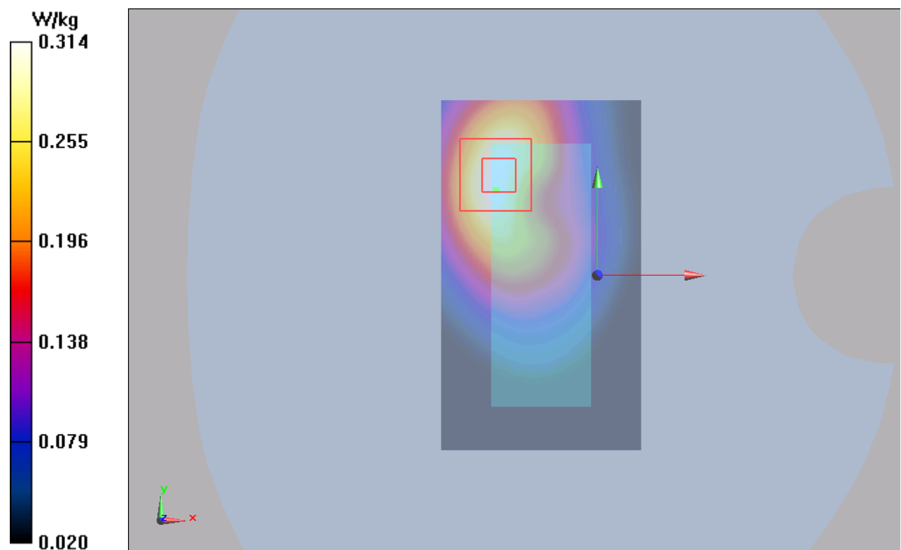
Figure 119 LTE Band 17 with Test Position 2 Channel 23790
