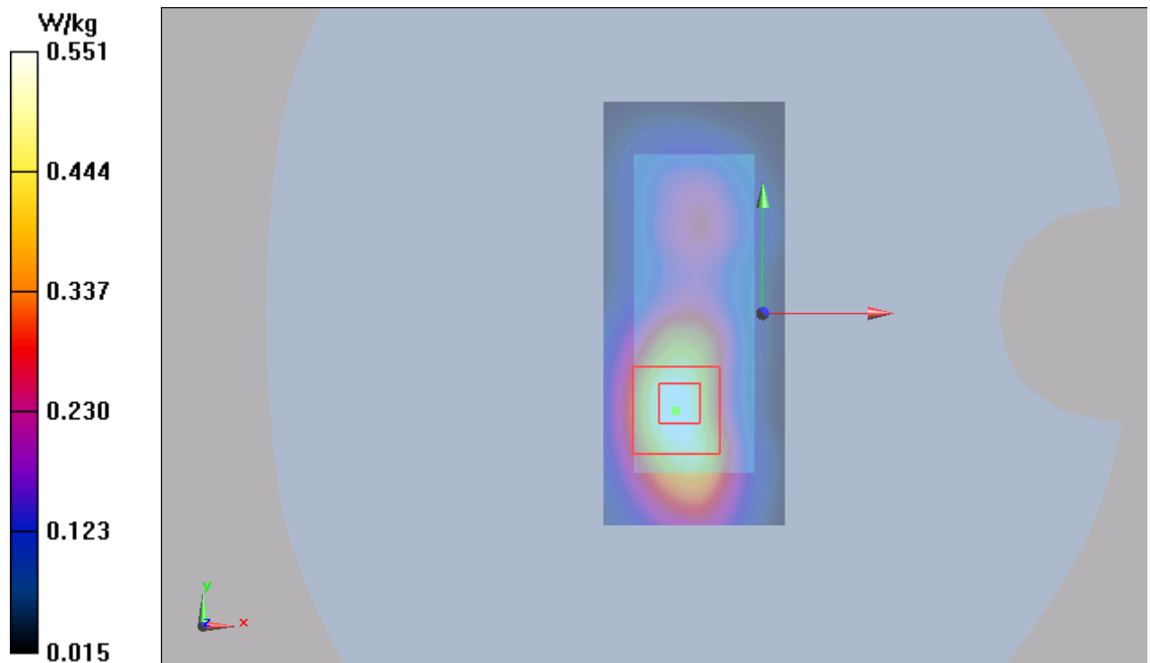
Figure 27 GSM 1900 EGPRS (2TXslots) with Test Position 1 Channel 512
