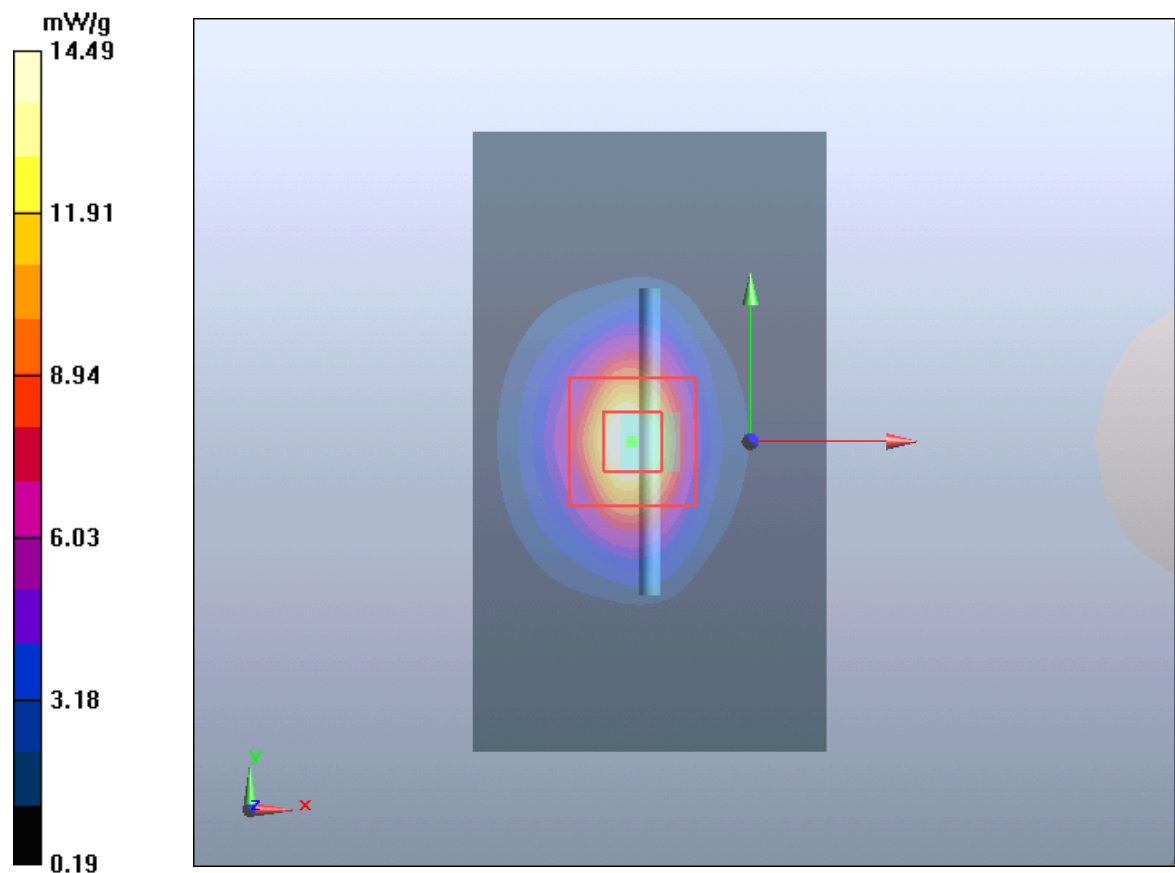
Figure 13 System Performance Check 2450MHz 250mW
