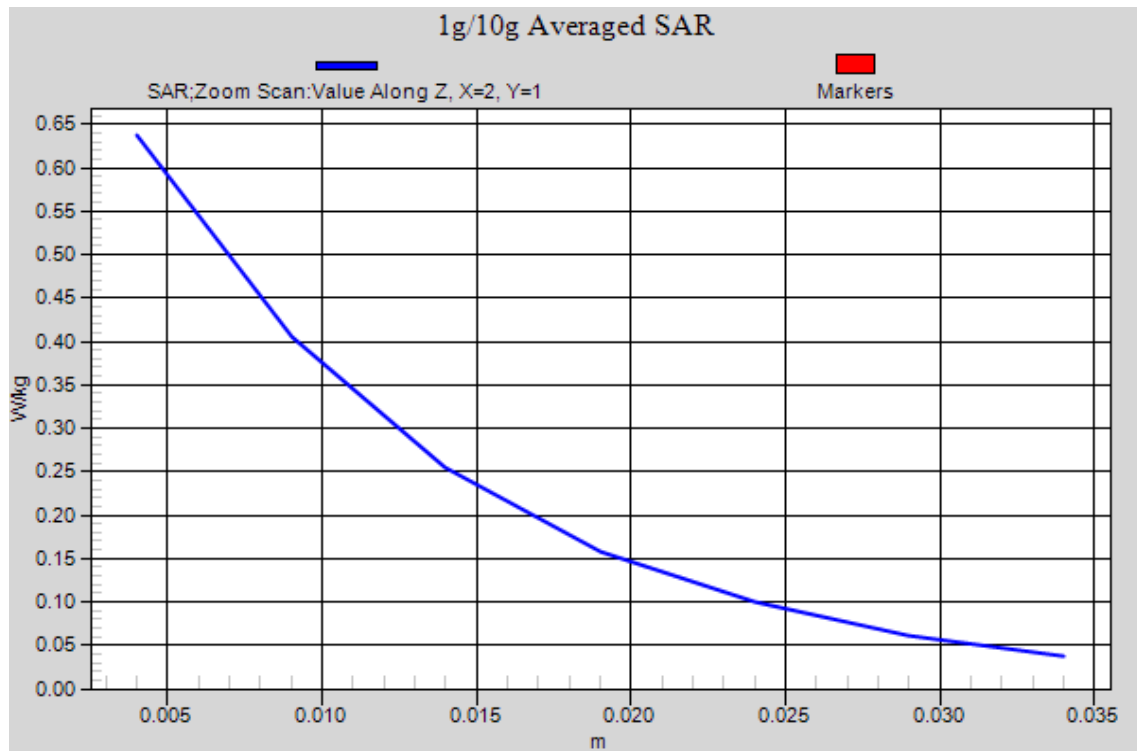
Figure 23 GSM 1900 GPRS (2TXslots) with Test Position 1 Channel 512
