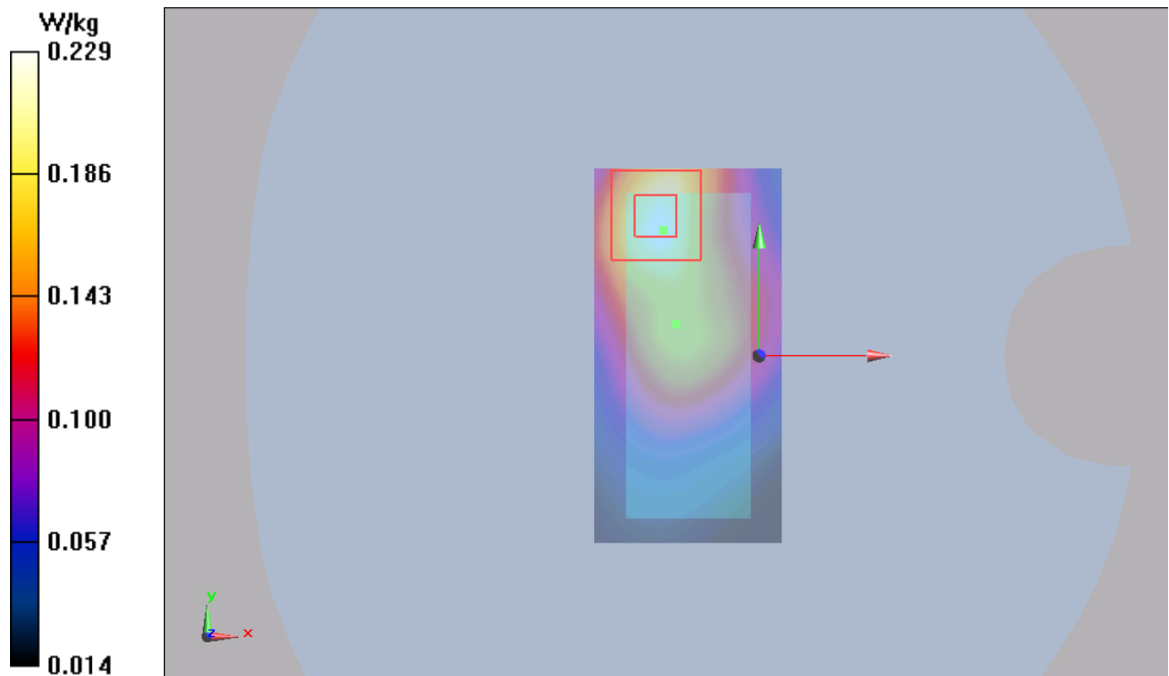
Figure 114 LTE Band 17 with Test Position 2 Channel 23780
