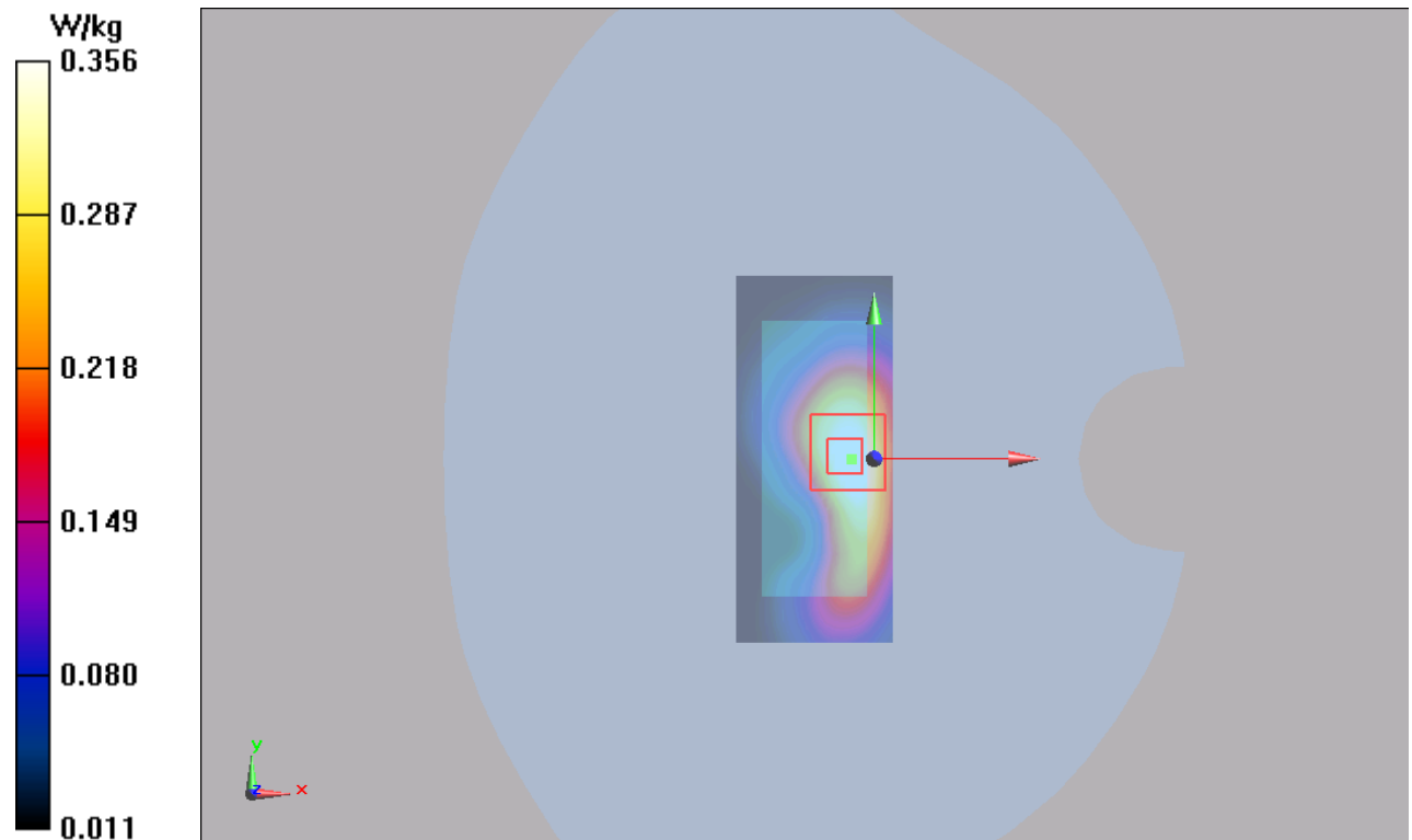
Figure 51 LTE Band 2 with Test Position 2 Channel 18700
