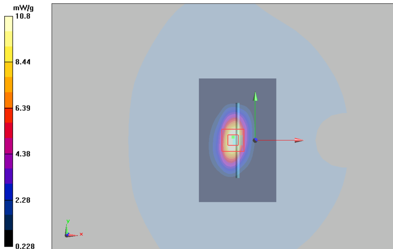
Figure 10 System Performance Check 1750MHz 250mW
