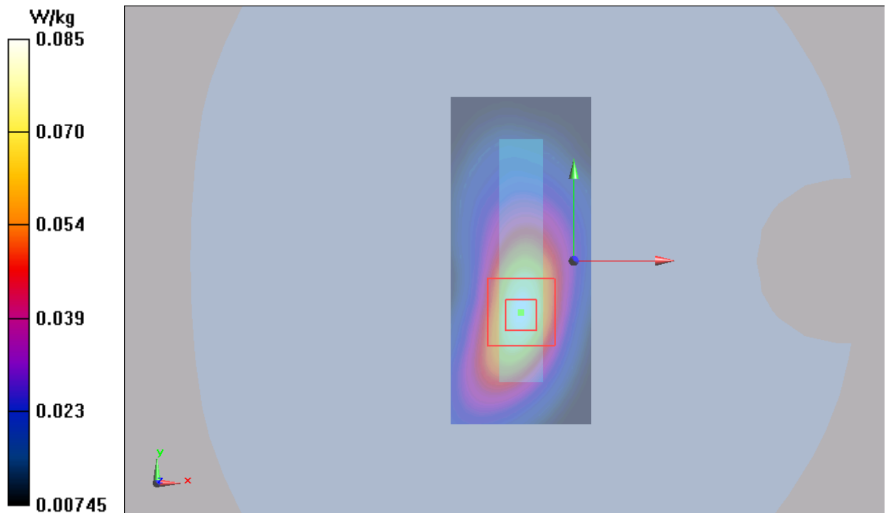
Figure 109 LTE Band 12 with Test Position 3 Channel 23060
