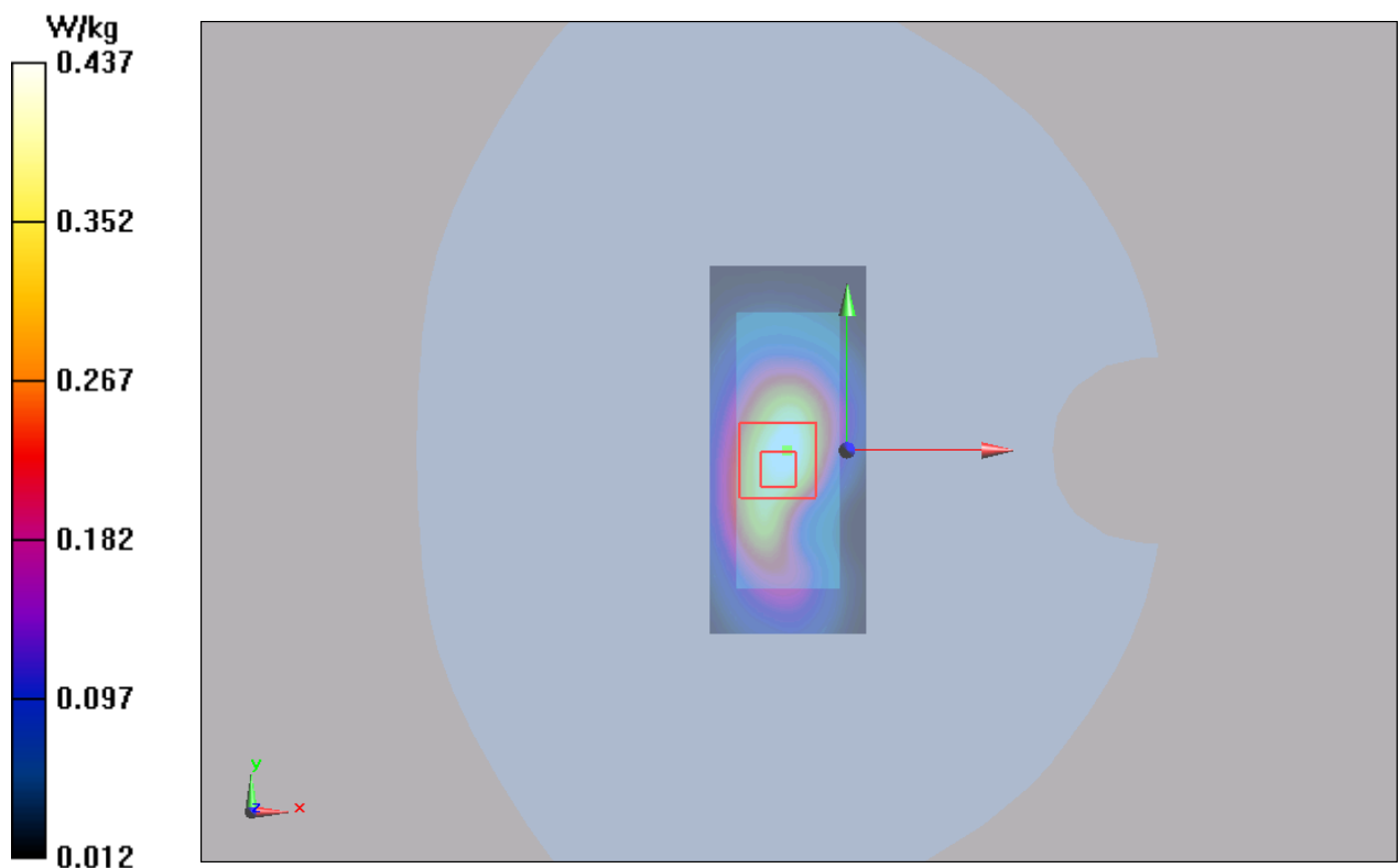
Figure 29 UMTS Band II with Test Position 1 Channel 9400
