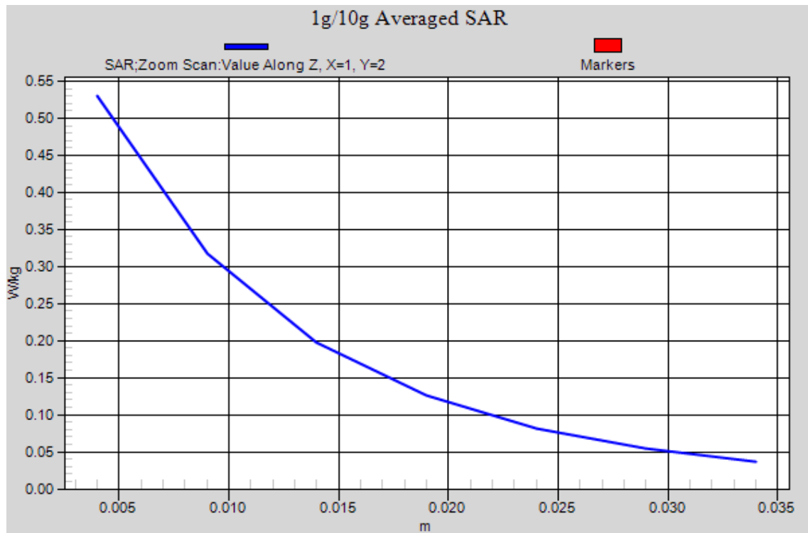
Figure 16 GSM 850 GPRS (2TXslots) with Test Position 1 Channel 128
