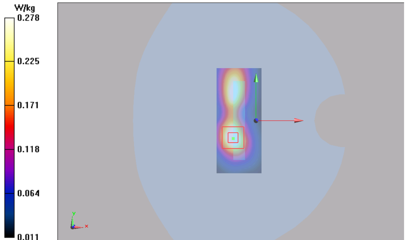
Figure 25 GSM 1900 GPRS (2TXslots) with Test Position 3 Channel 661
