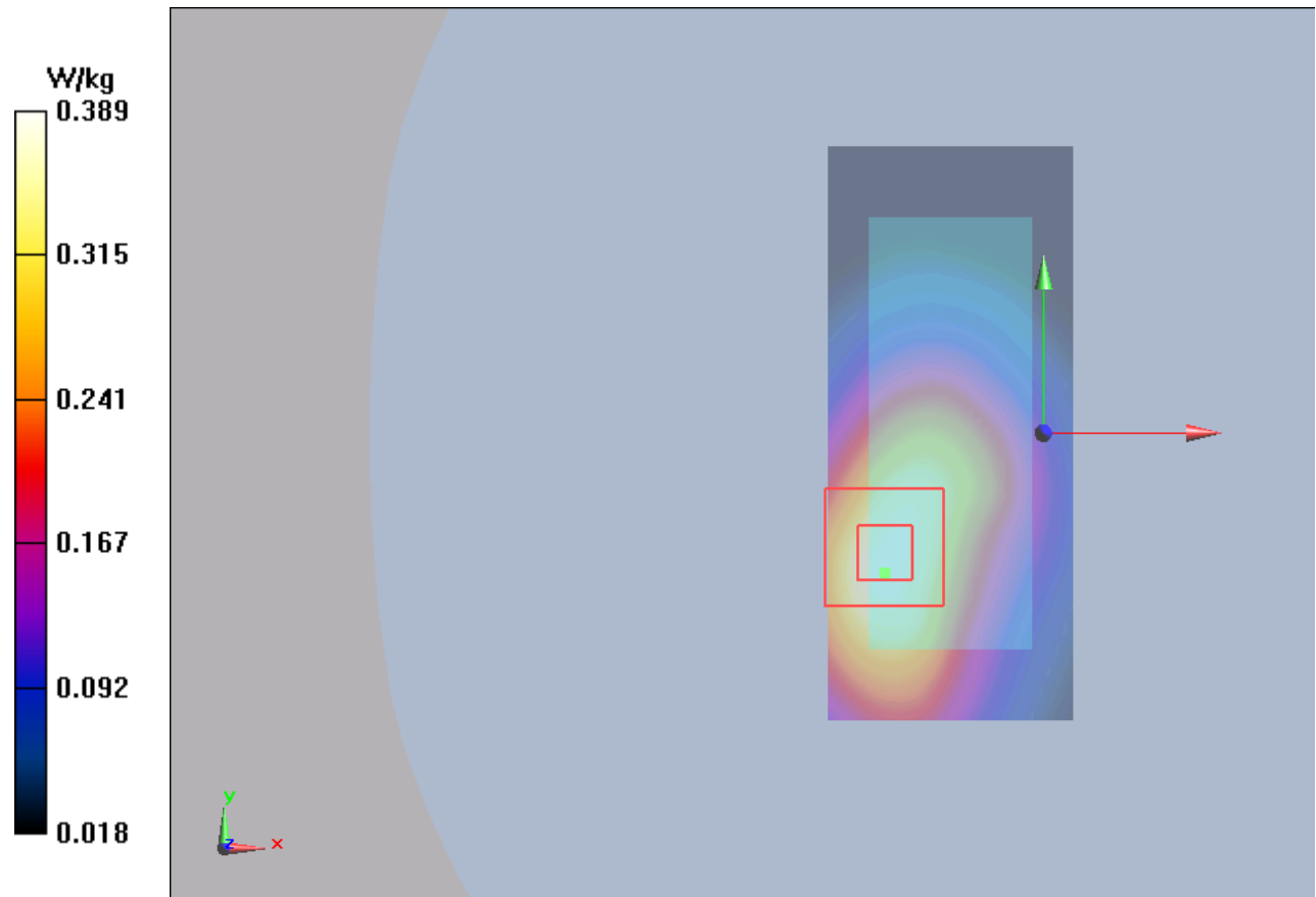
Figure 79 LTE Band 5 with Test Position 1 Channel 20600
