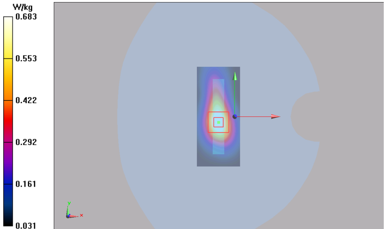
Figure 60 LTE Band 2 with Test Position 3 Channel 18900
