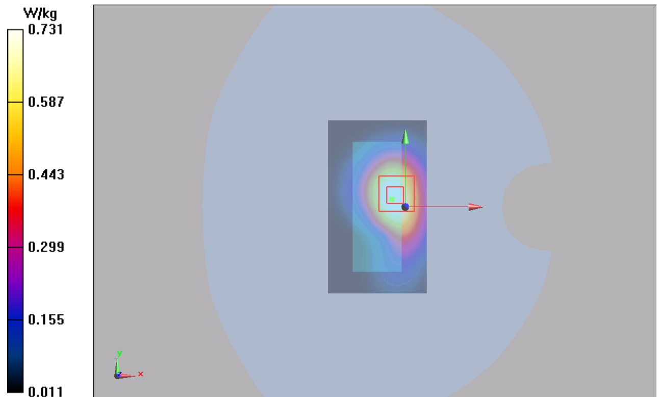
Figure 63 LTE Band 2 with Test Position 2 Channel 18900
