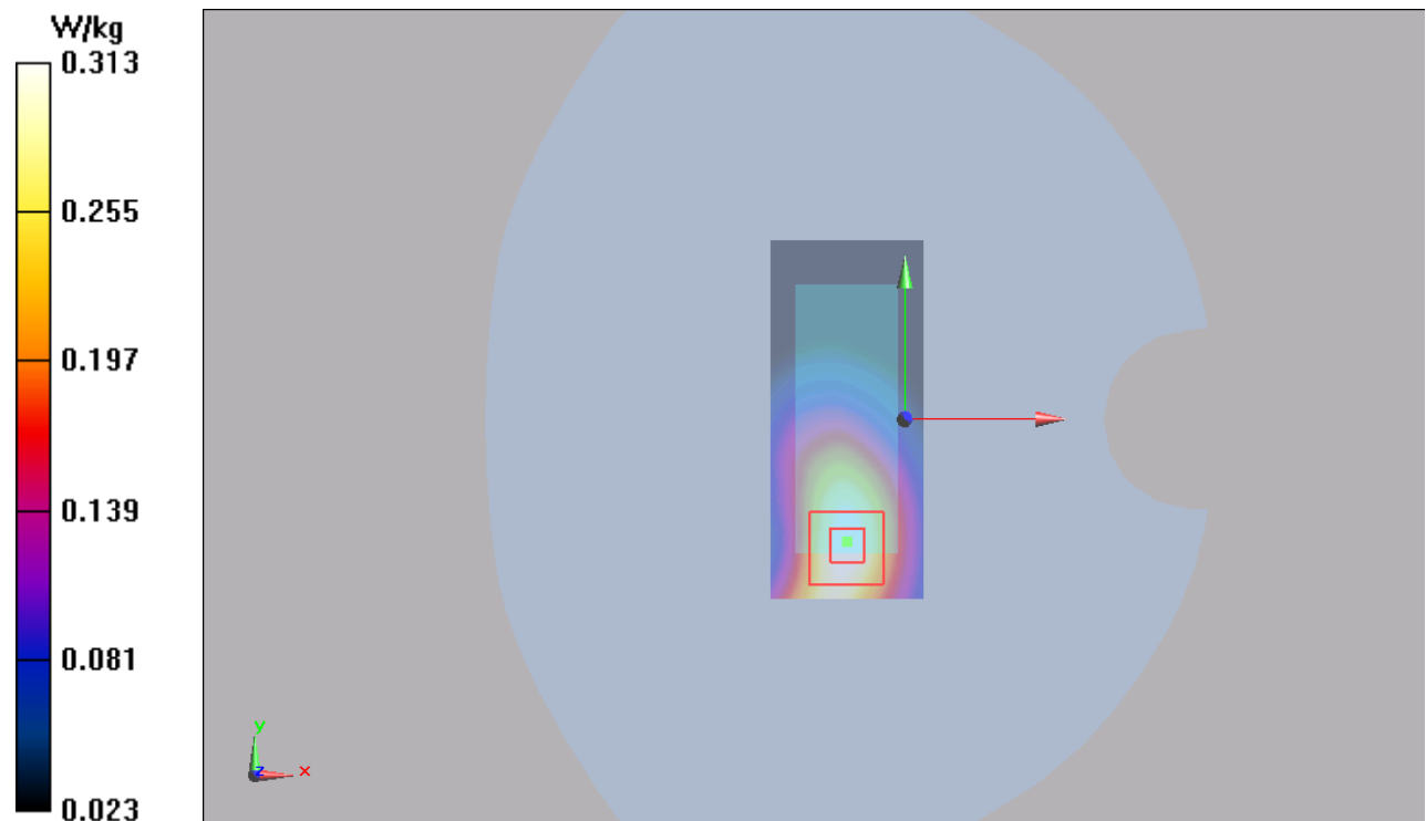
Figure 17 GSM 850 GPRS (2TXslots) with Test Position 2 Channel 190
