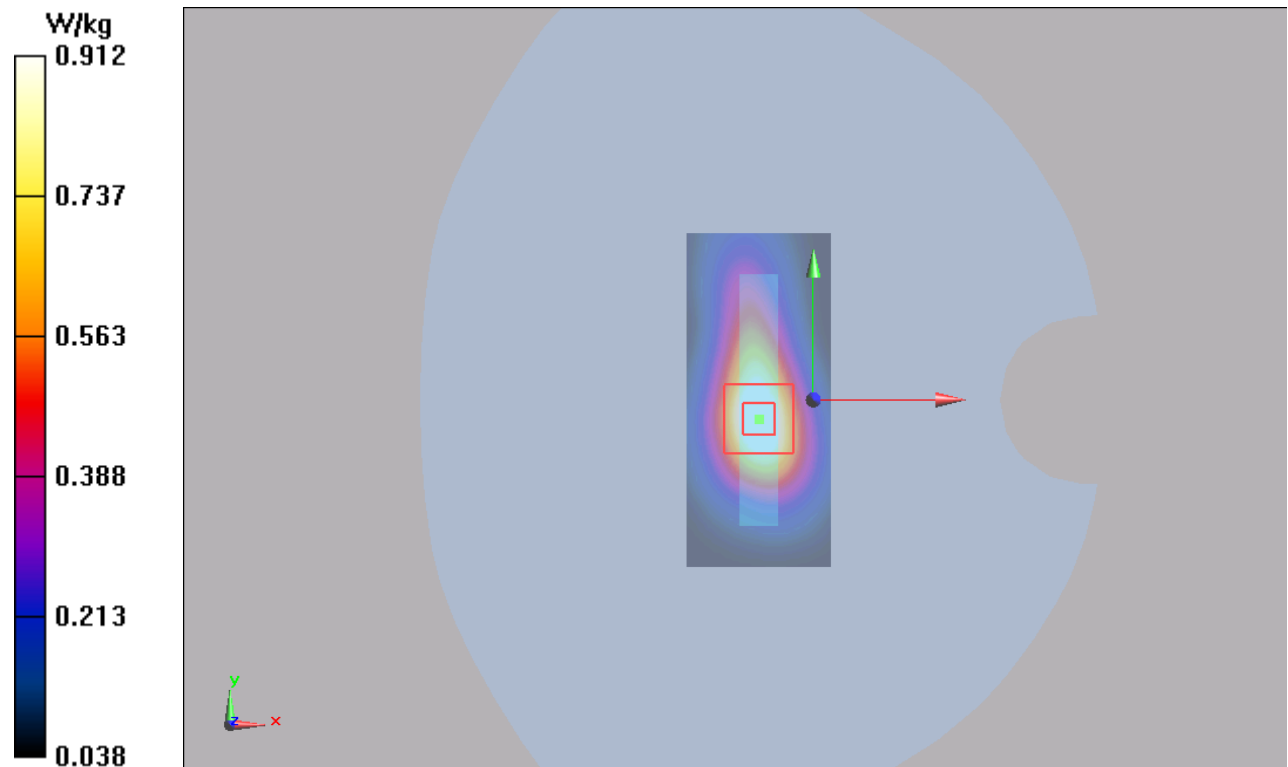
Figure 53 LTE Band 2 with Test Position 3 Channel 18900
