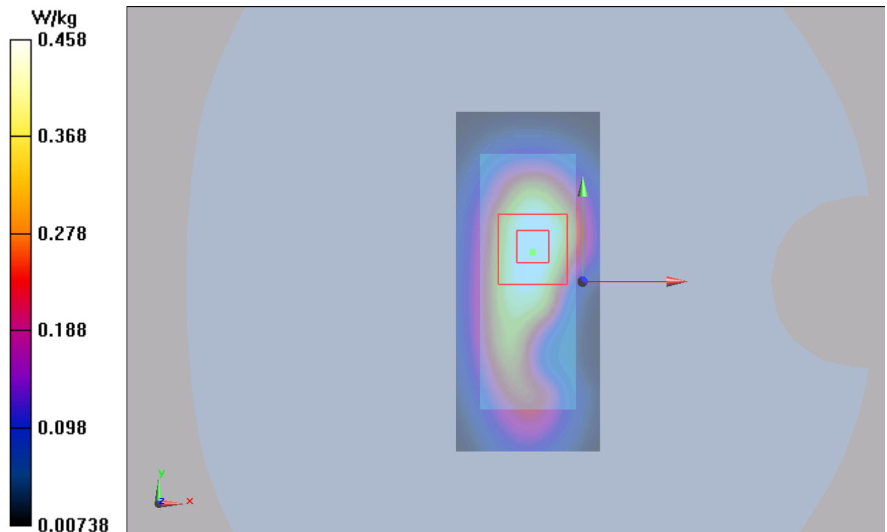
Figure 21 GSM 1900 GPRS (2TXslots) with Test Position 1 Channel 810
