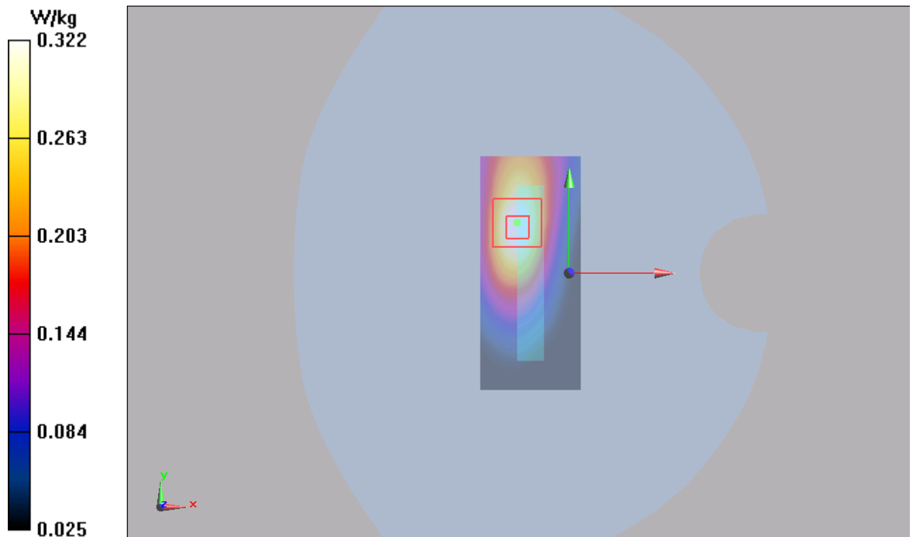
Figure 44 UMTS Band V with Test Position 3 Channel 4182
