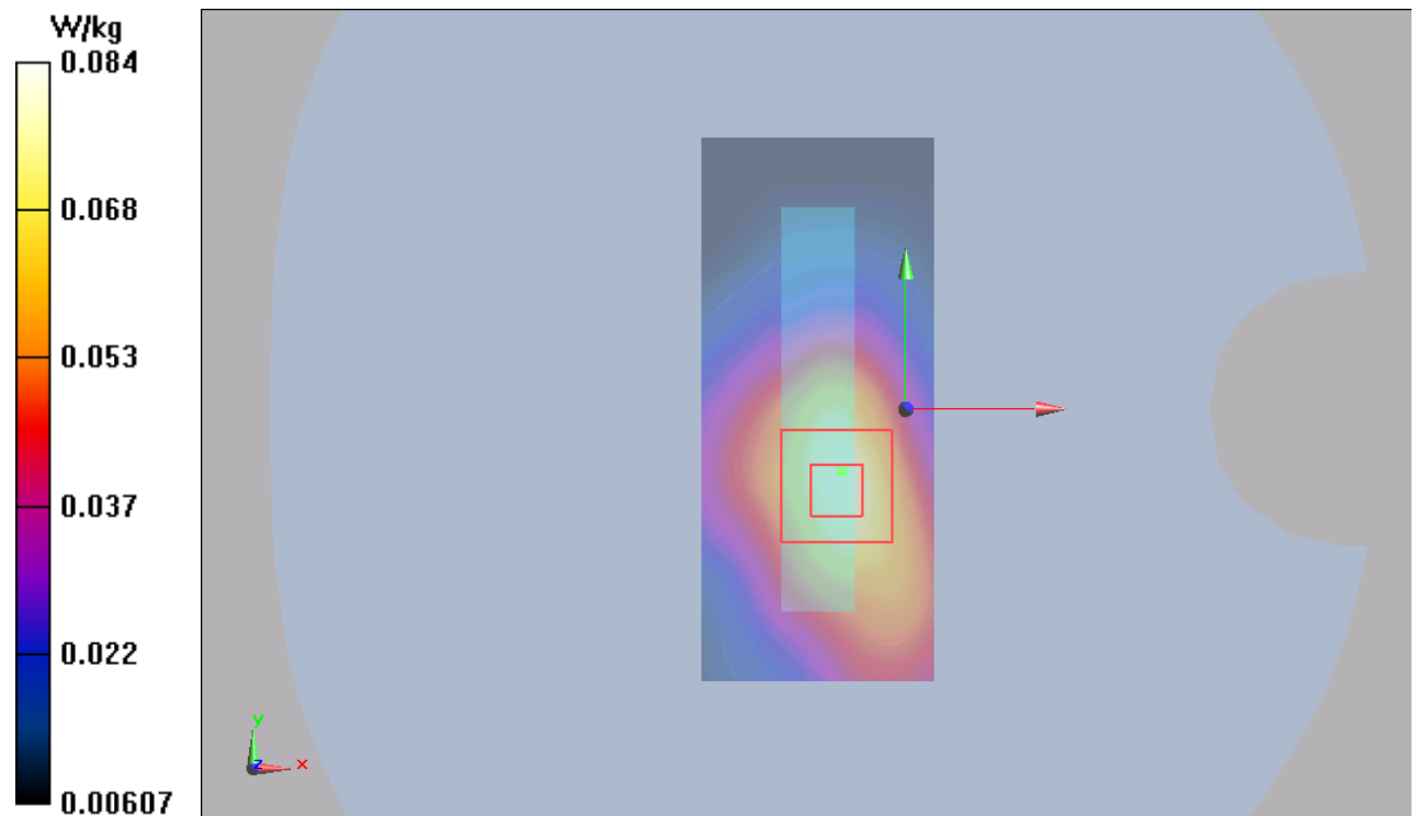
Figure 121 LTE Band 17 with Test Position 3 Channel 23780
