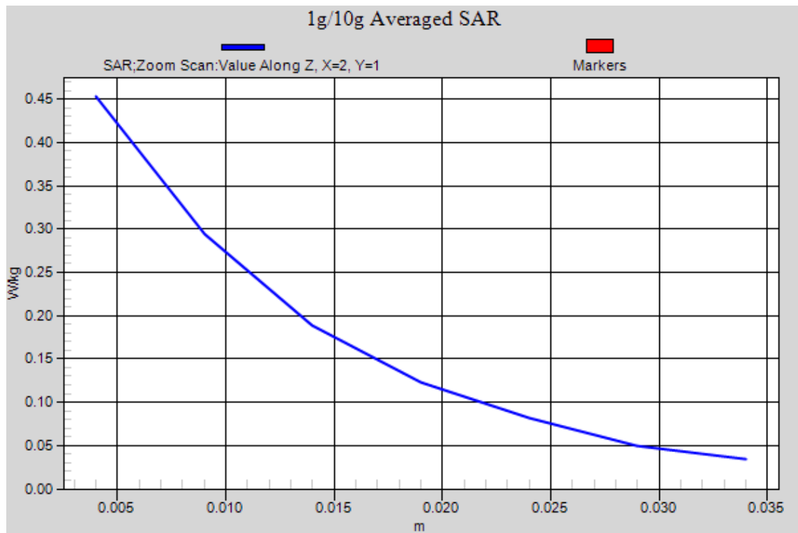
Figure 35 UMTS Band IV with Test Position 1 Channel 1413
