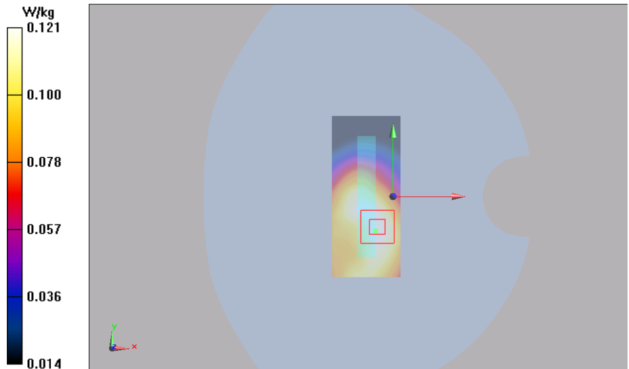
Figure 45 UMTS Band V with Test Position 4 Channel 4182
