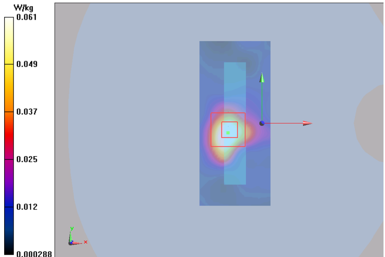
Figure 134 802.11b Test Position 4 Channel 1
