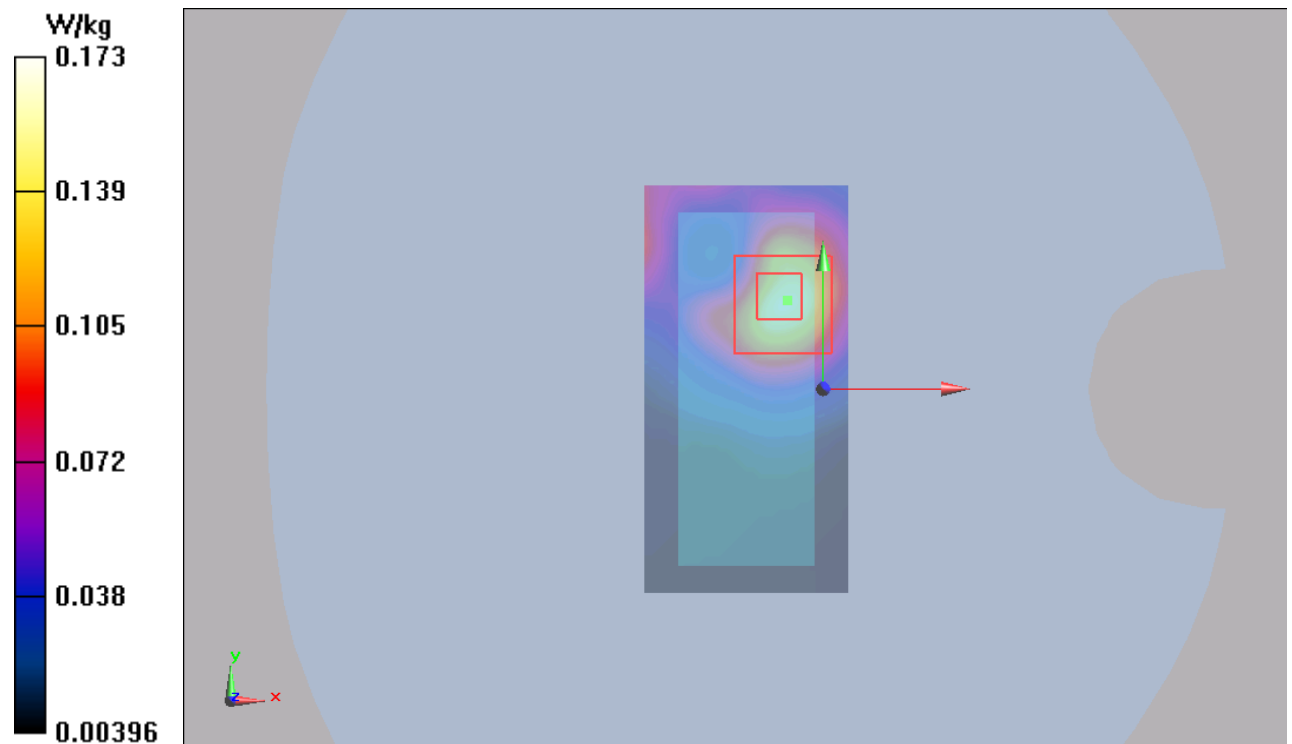
Figure 117 LTE Band 17 with Test Position 1 Channel 23780
