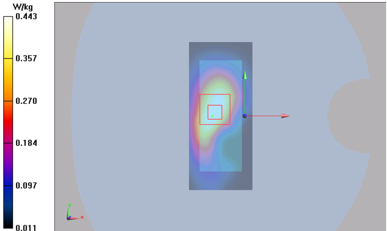
Figure 34 UMTS Band IV with Test Position 1 Channel 1513
