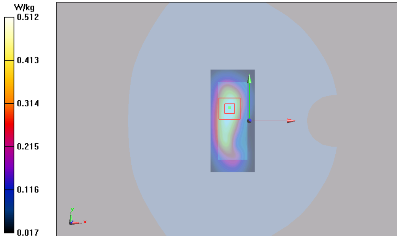
Figure 56 LTE Band 2 with Test Position 1 Channel 19100
