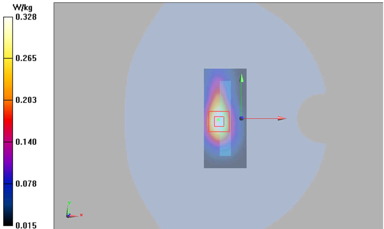
Figure 32 UMTS Band II with Test Position 3 Channel 9400
