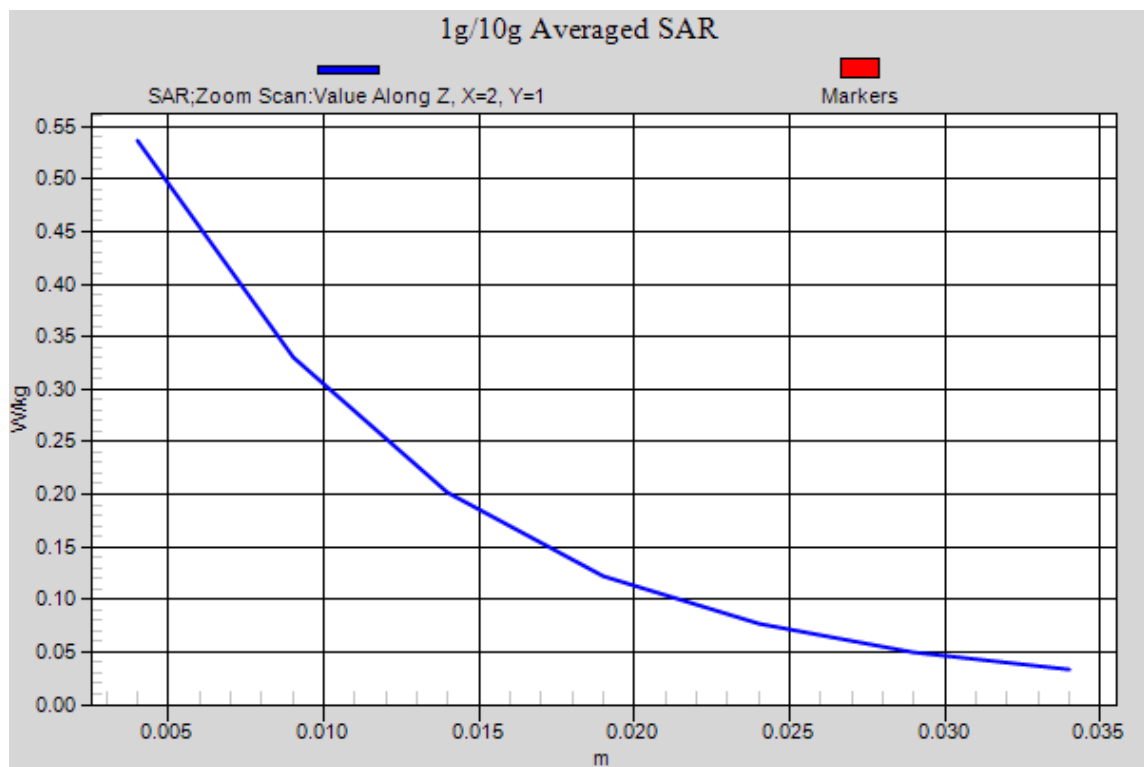
Figure 93 UMTS Band II with Test Position 1 Channel 9262
