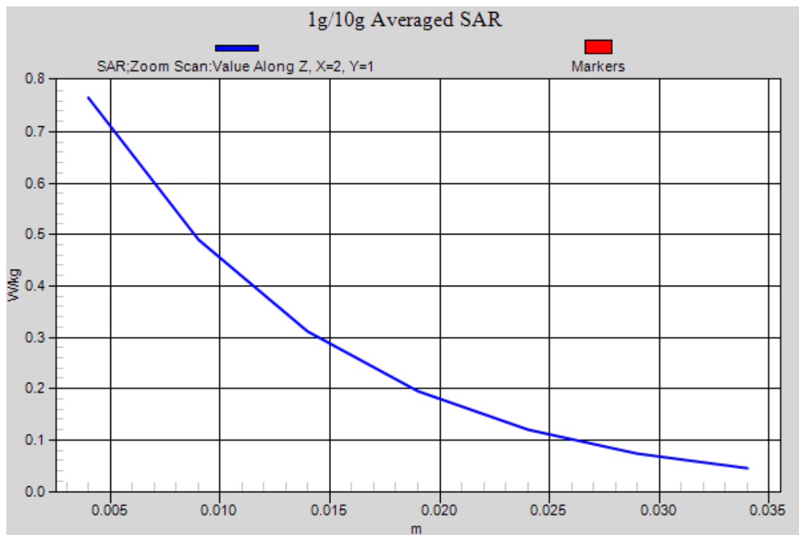
Figure 97 LTE Band 4 with Test Position 1 Channel 20175
