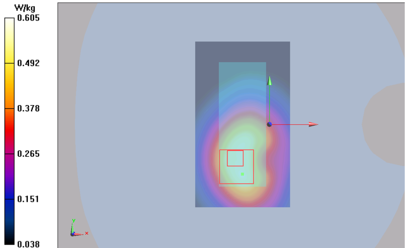
Figure 107 LTE Band 12 with Test Position 1 Channel 23060
