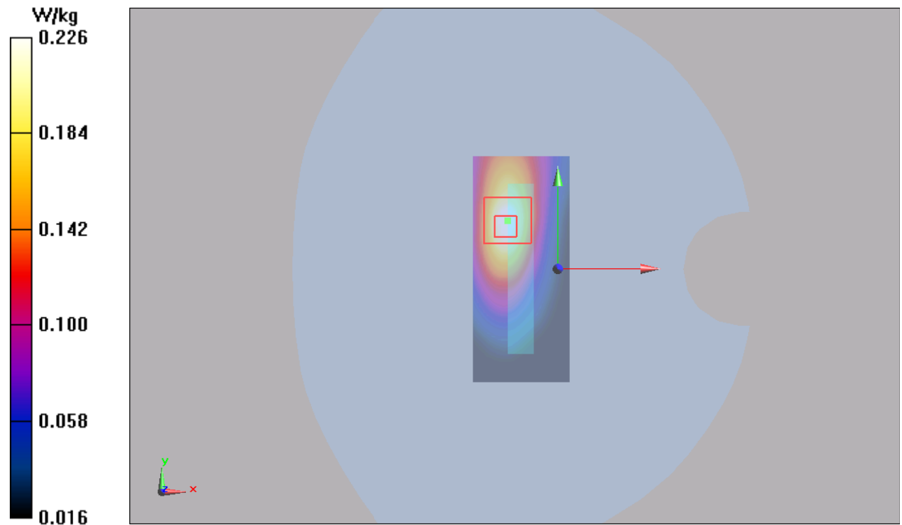
Figure 18 GSM 850 GPRS (2TXslots) with Test Position 3 Channel 190
