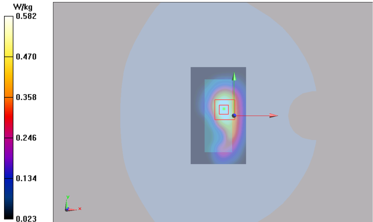
Figure 67 LTE Band 4 with Test Position 1 Channel 20175
