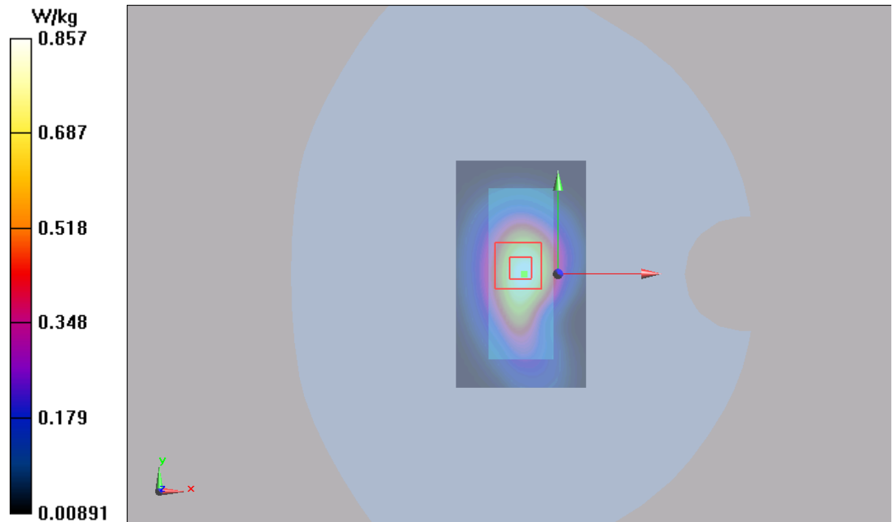
Figure 62 LTE Band 2 with Test Position 1 Channel 18900
