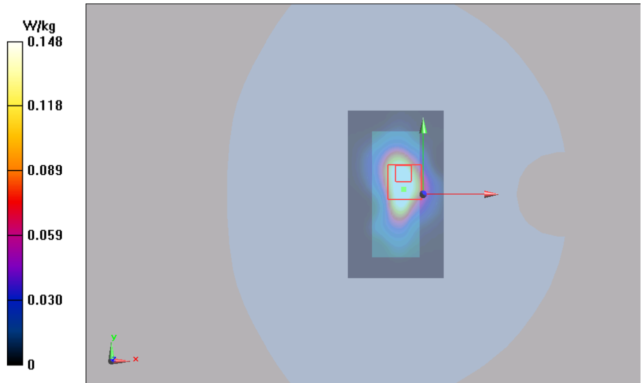
Figure 126 802.11b Test Position 2 Channel 1
