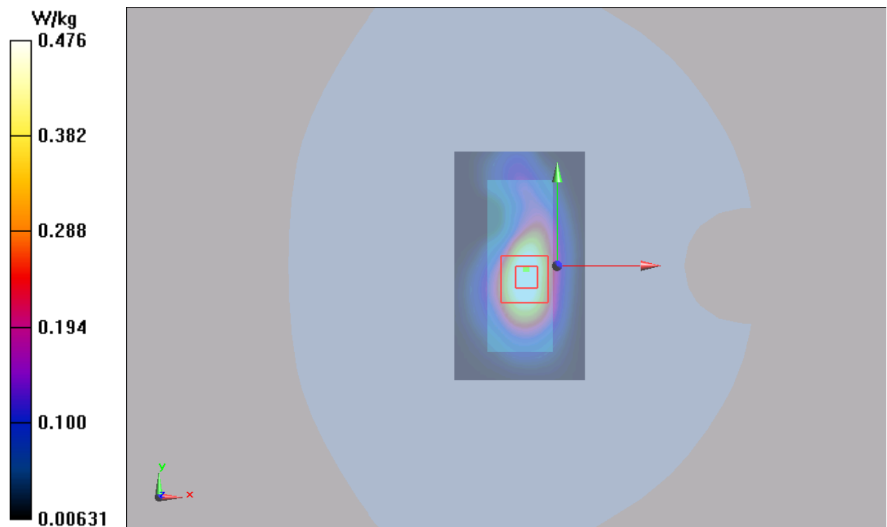
Figure 73 LTE Band 4 with Test Position 1 Channel 20175
