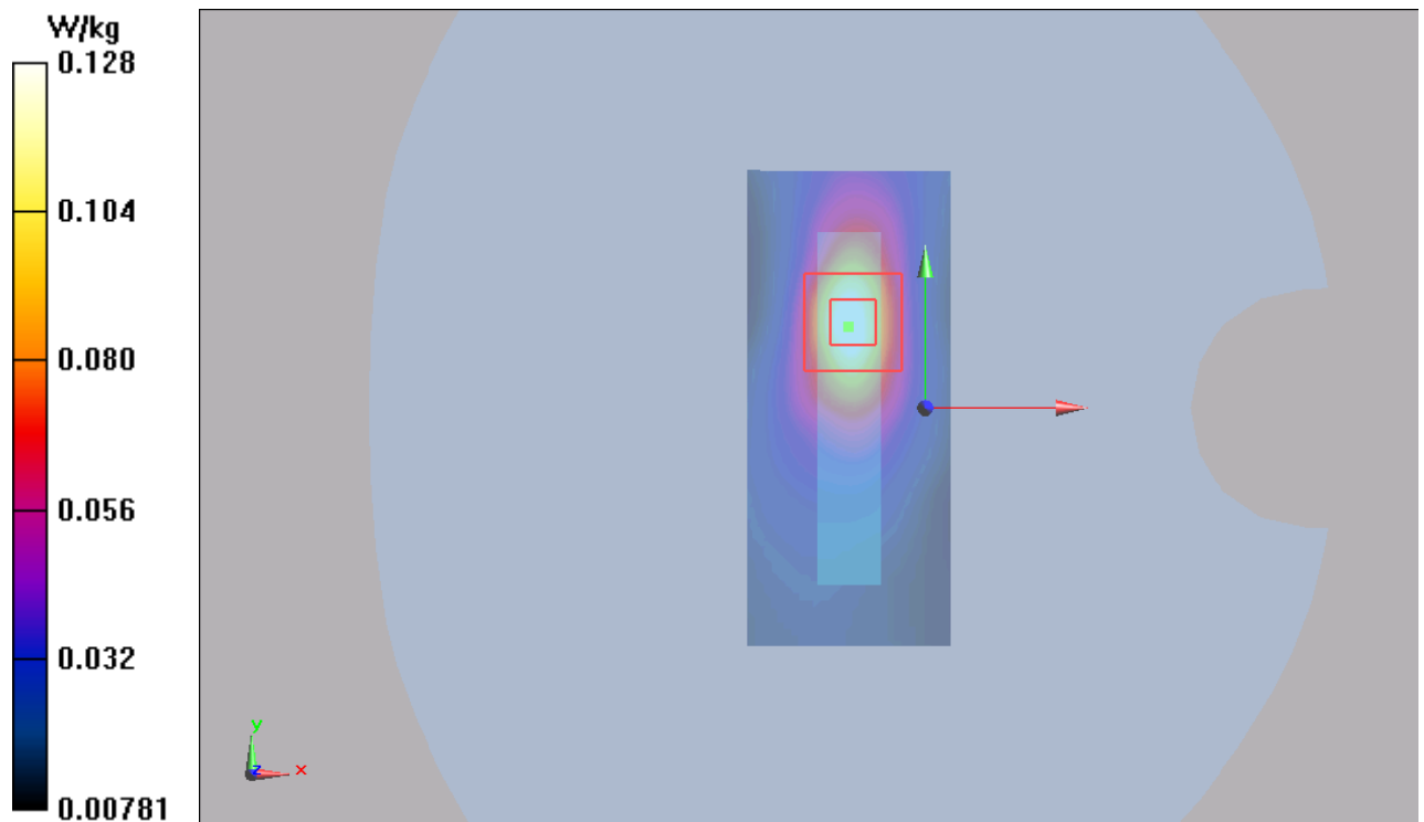
Figure 104 LTE Band 12 with Test Position 4 Channel 23060
