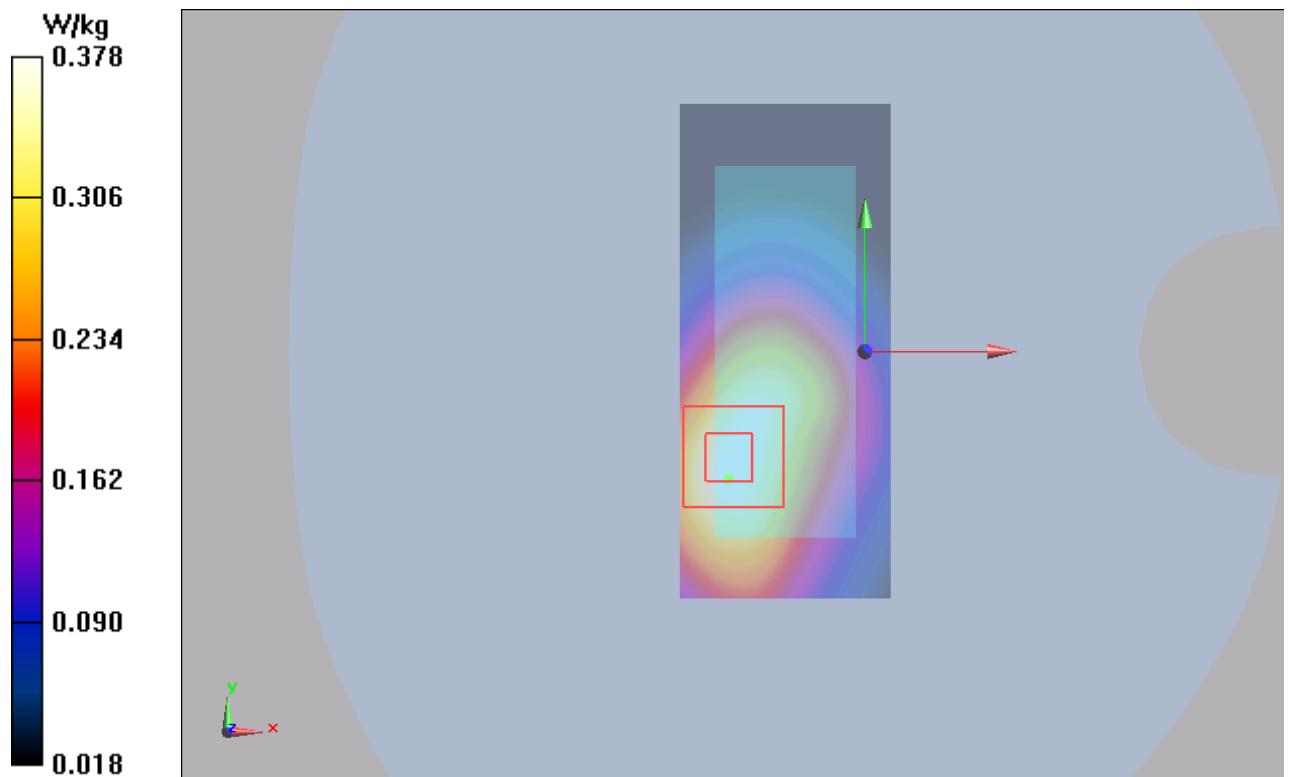
Figure 87 LTE Band 5 with Test Position 1 Channel 20450
