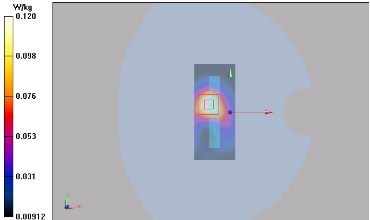
Figure 33 UMTS Band II with Test Position 4 Channel 9400
