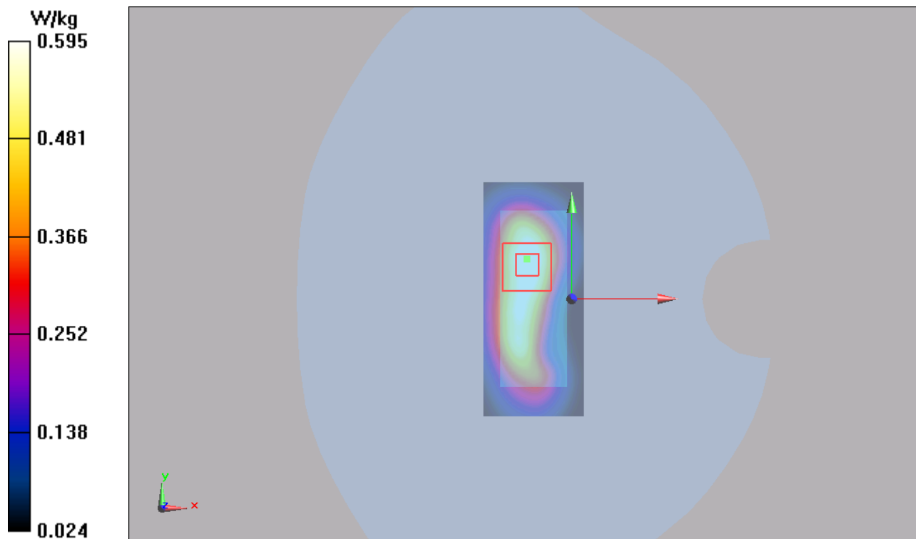
Figure 46 LTE Band 2 with Test Position 1 Channel 19100
