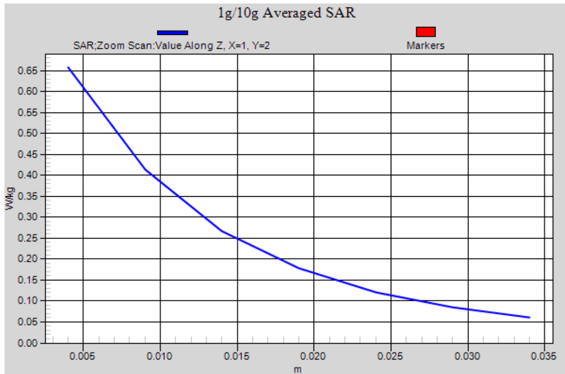
Figure 40 UMTS Band V with Test Position 1 Channel 4233
