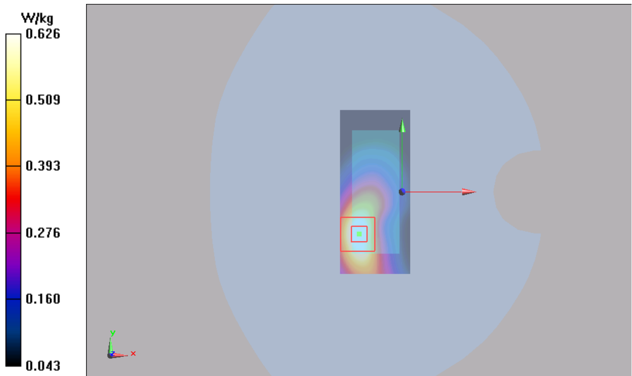
Figure 41 UMTS Band V with Test Position 1 Channel 4182
