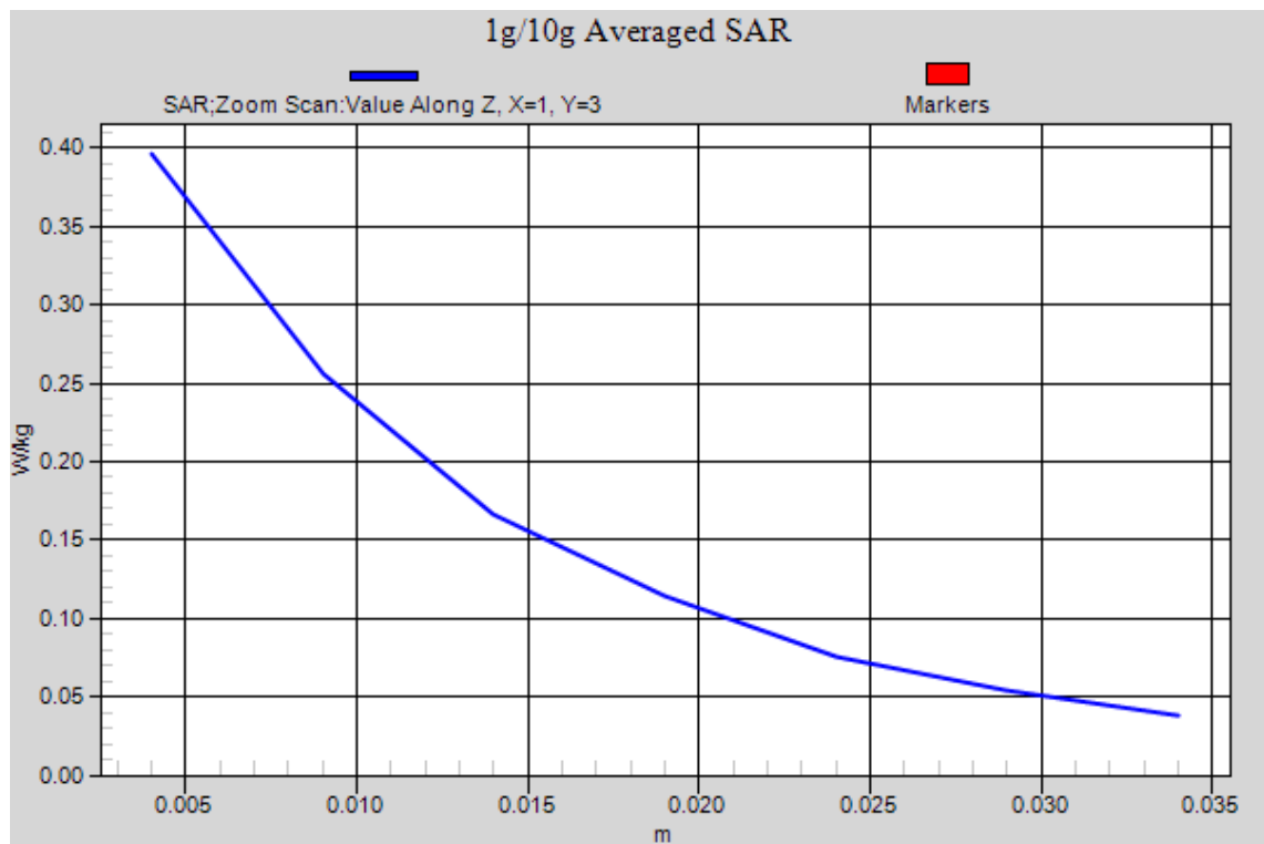
Figure 98 LTE Band 5 with Test Position 1 Channel 20450
