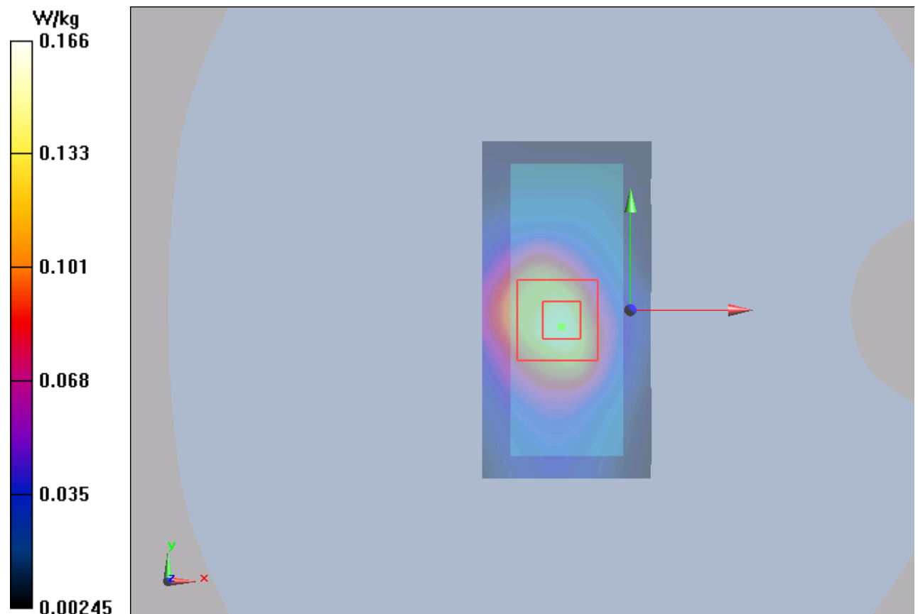
Figure 130 802.11b Test Position 2 Channel 1
