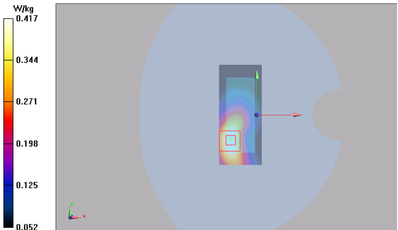
Figure 15 GSM 850 GPRS (2TXslots) with Test Position 1 Channel 190
