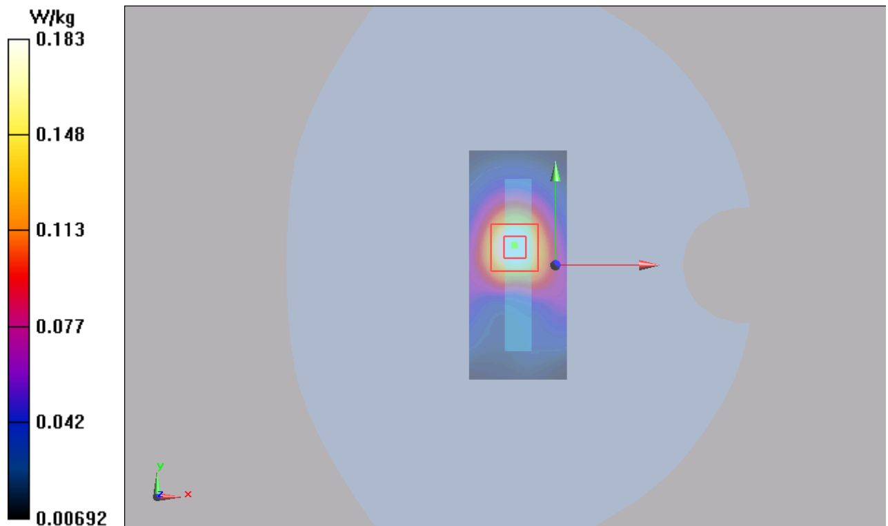
Figure 71 LTE Band 4 with Test Position 4 Channel 20050
