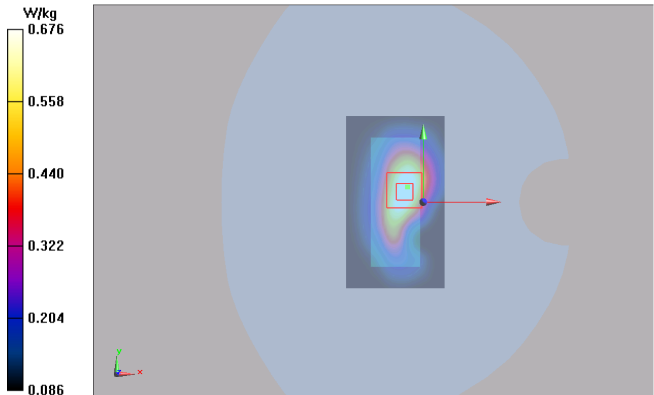
Figure 78 LTE Band 4 with Test Position 1 Channel 20175
