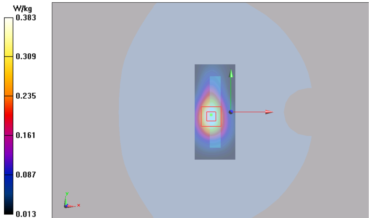
Figure 38 UMTS Band IV with Test Position 3 Channel 1413
