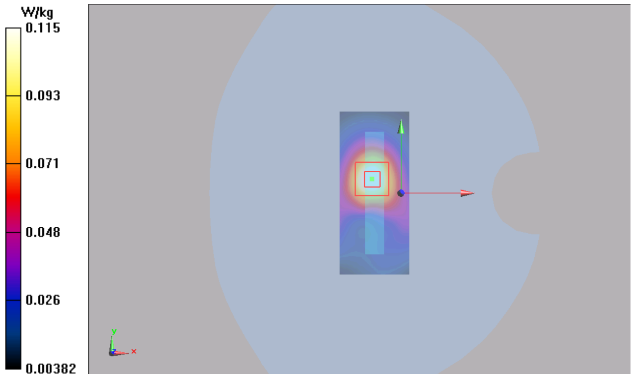
Figure 77 LTE Band 4 with Test Position 4 Channel 20175
