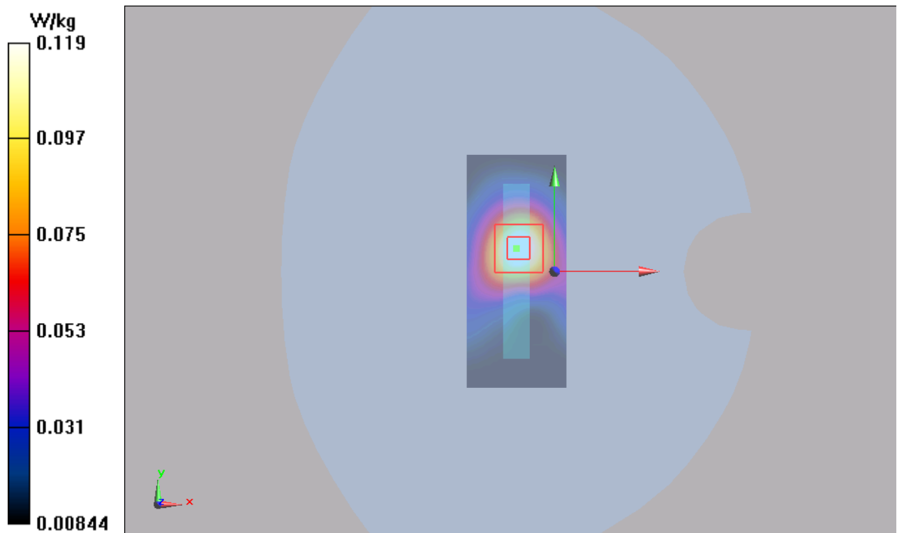
Figure 39 UMTS Band IV with Test Position 4 Channel 1413
