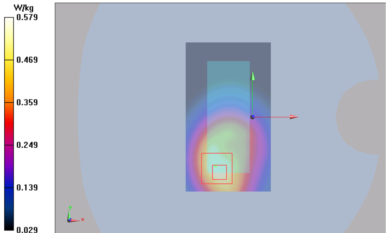
Figure 113 LTE Band 17 with Test Position 1 Channel 23780
