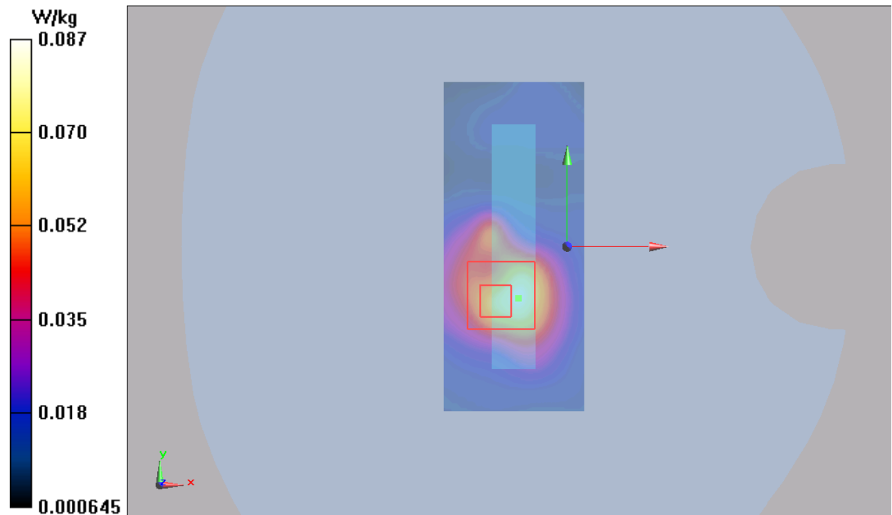
Figure 128 802.11b Test Position 4 Channel 6
