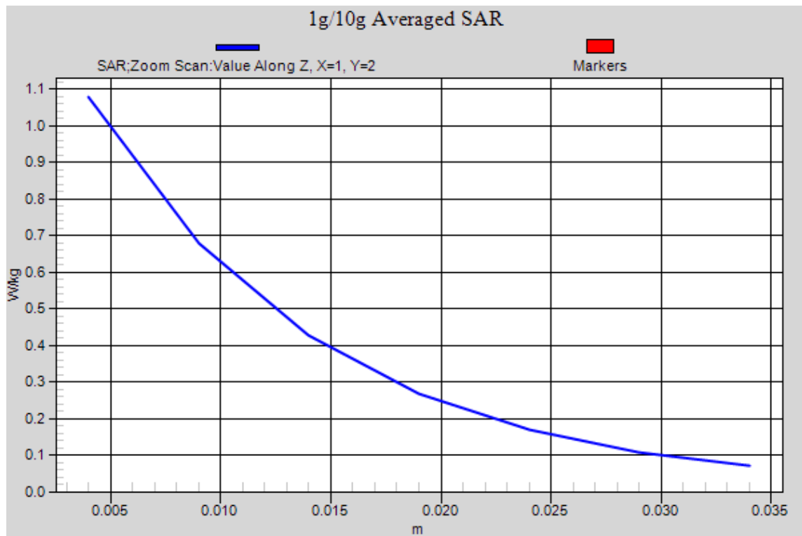
Figure 47 LTE Band 2 with Test Position 1 Channel 18900
