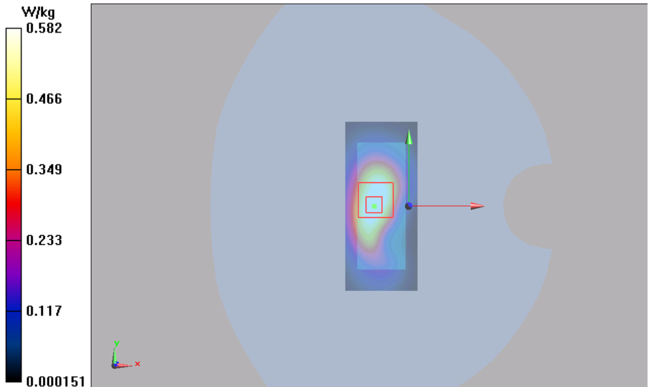
Figure 58 LTE Band 2 with Test Position 1 Channel 18700
