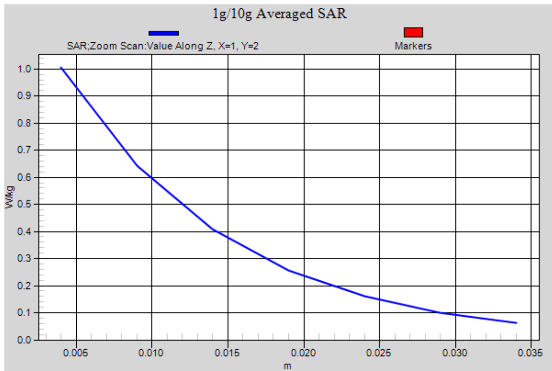
Figure 96 LTE Band 2 with Test Position 1 Channel 18900
