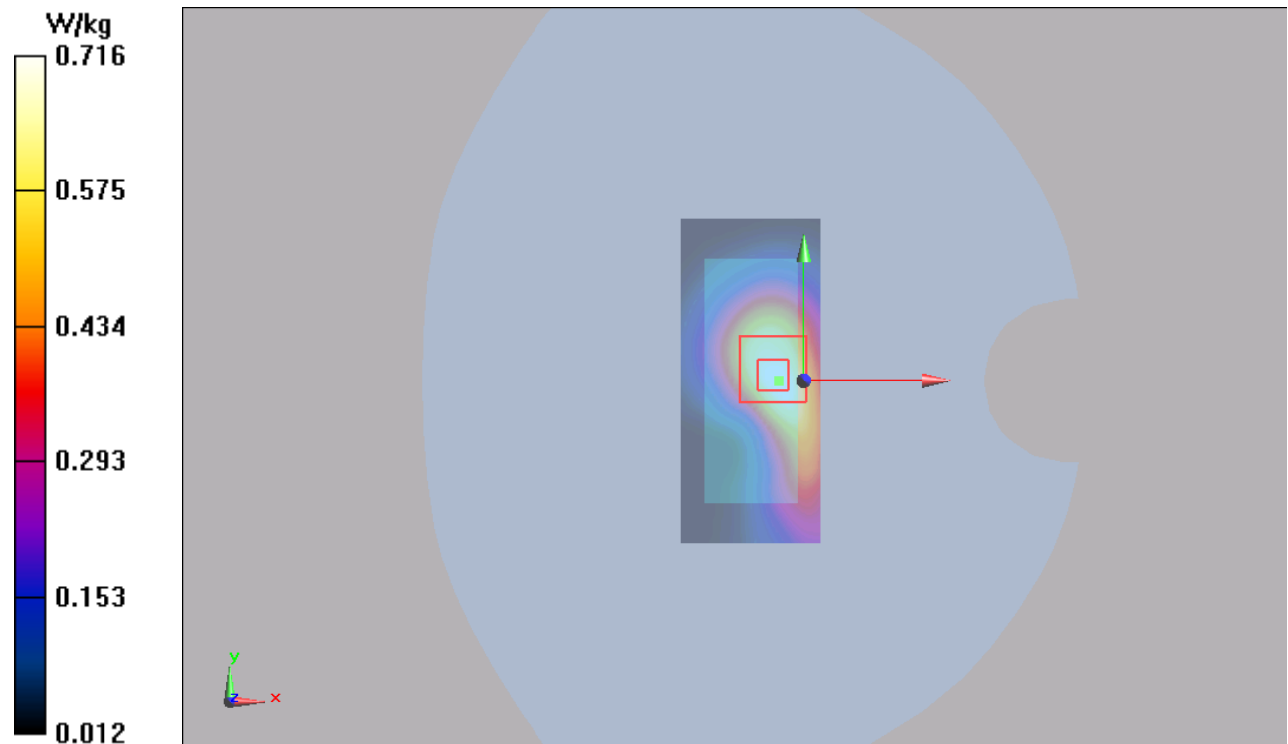
Figure 59 LTE Band 2 with Test Position 2 Channel 18900
