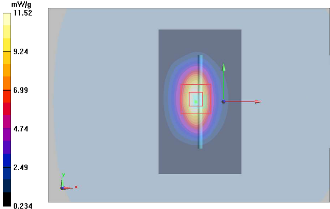
Figure 12 System Performance Check 1900MHz 250mW
