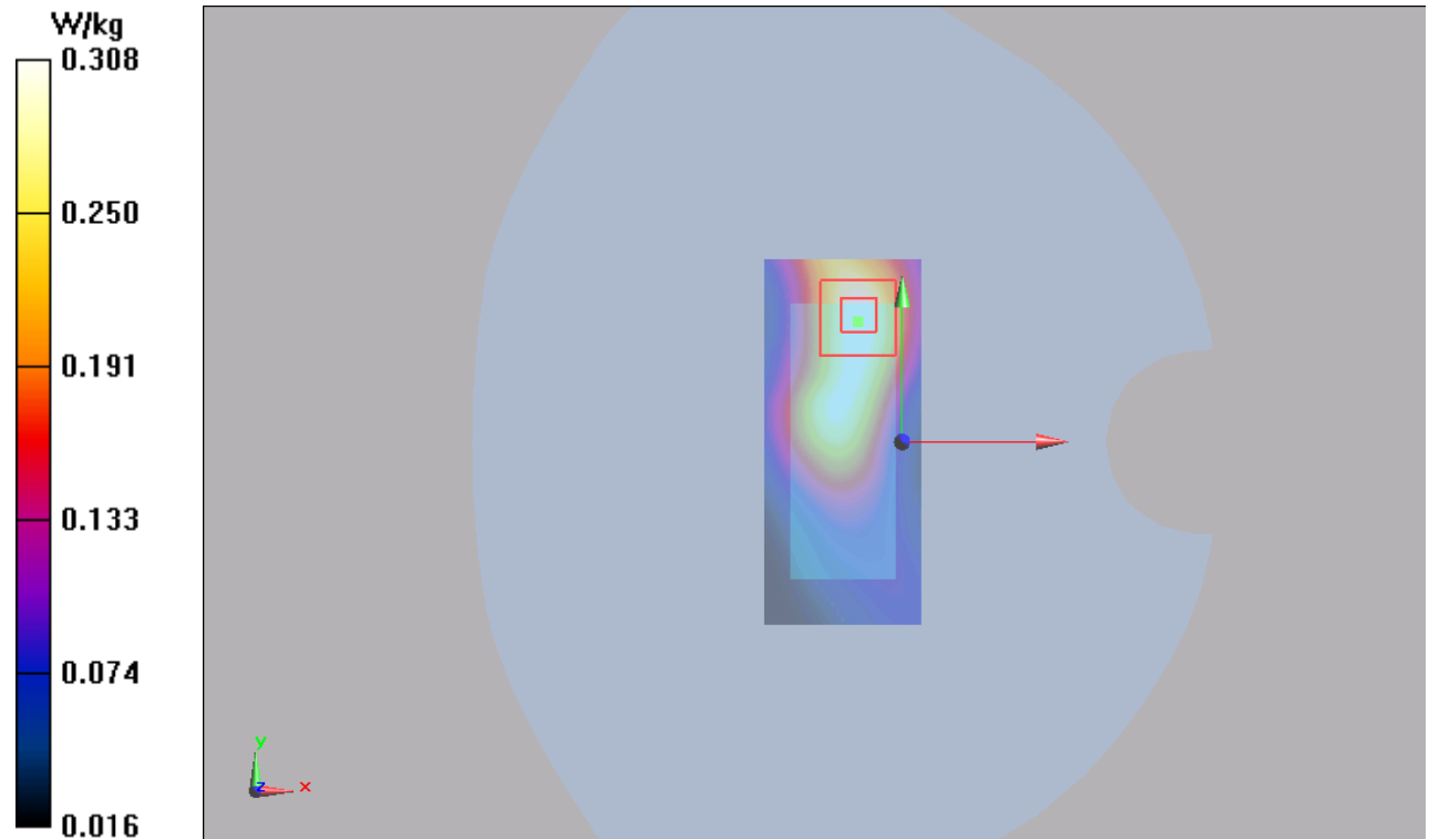
Figure 88 LTE Band 5 with Test Position 2 Channel 20525
