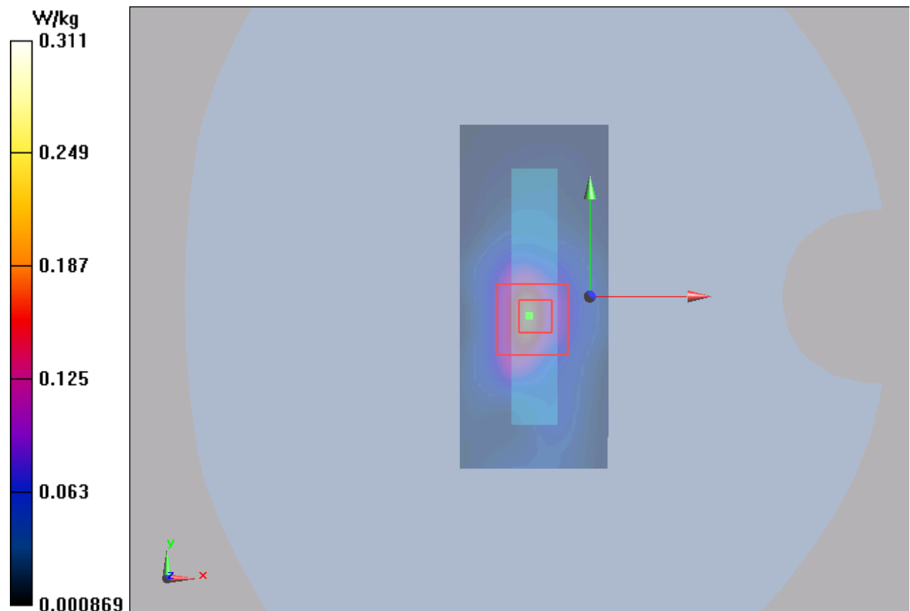
Figure 133 802.11b Test Position 3 Channel 1
