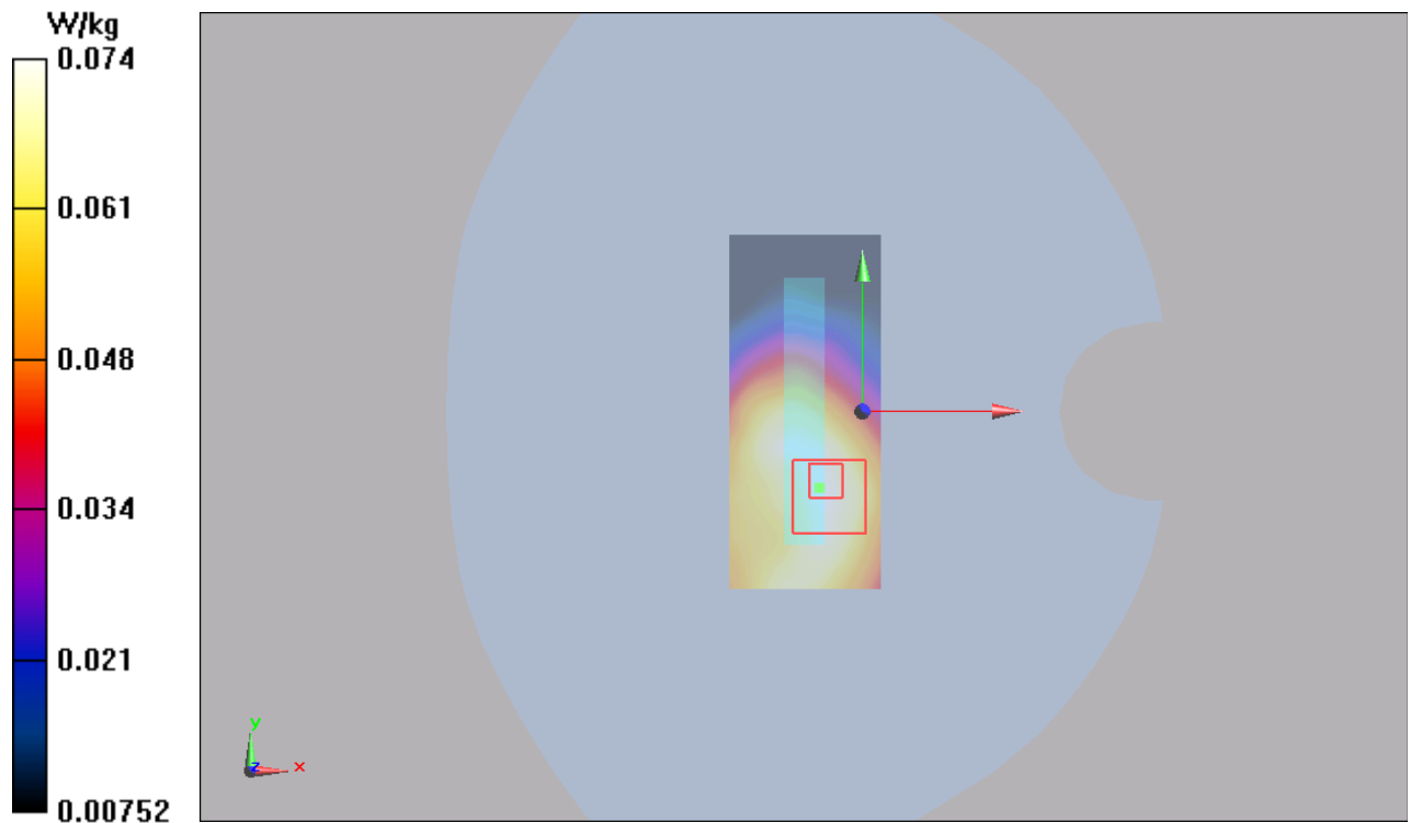
Figure 19 GSM 850 GPRS (2TXslots) with Test Position 4 Channel 190
