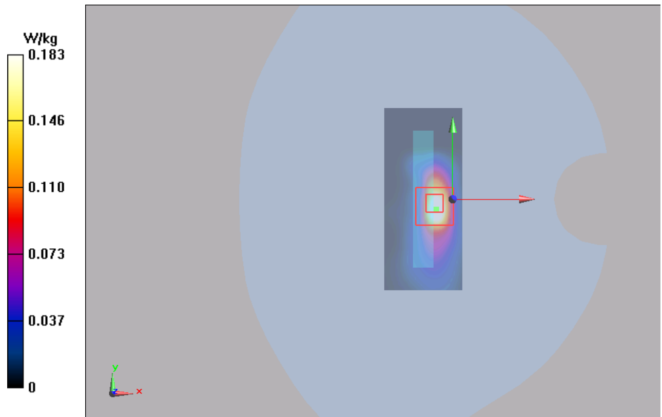
Figure 131 802.11b Test Position 3 Channel 11
