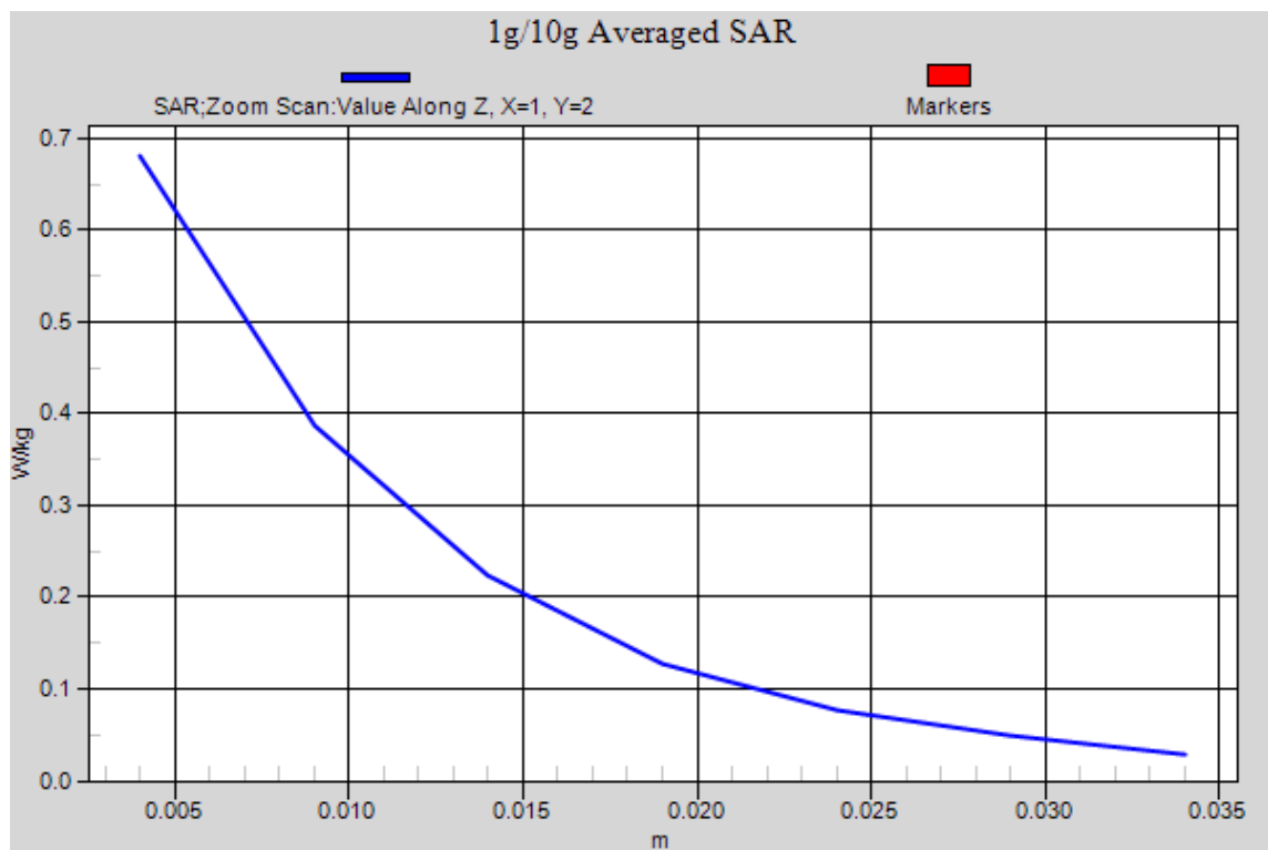
Figure 92 GSM 1900 GPRS (2TXslots) with Test Position 1 Channel 512
