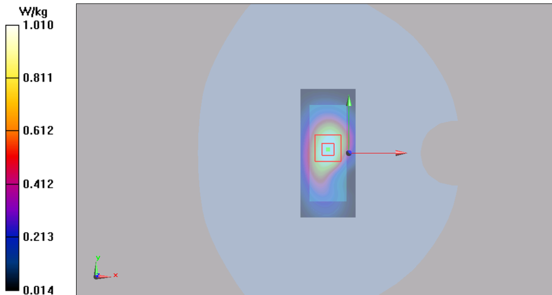
Figure 65 LTE Band 2 with Test Position 1 Channel 18900
