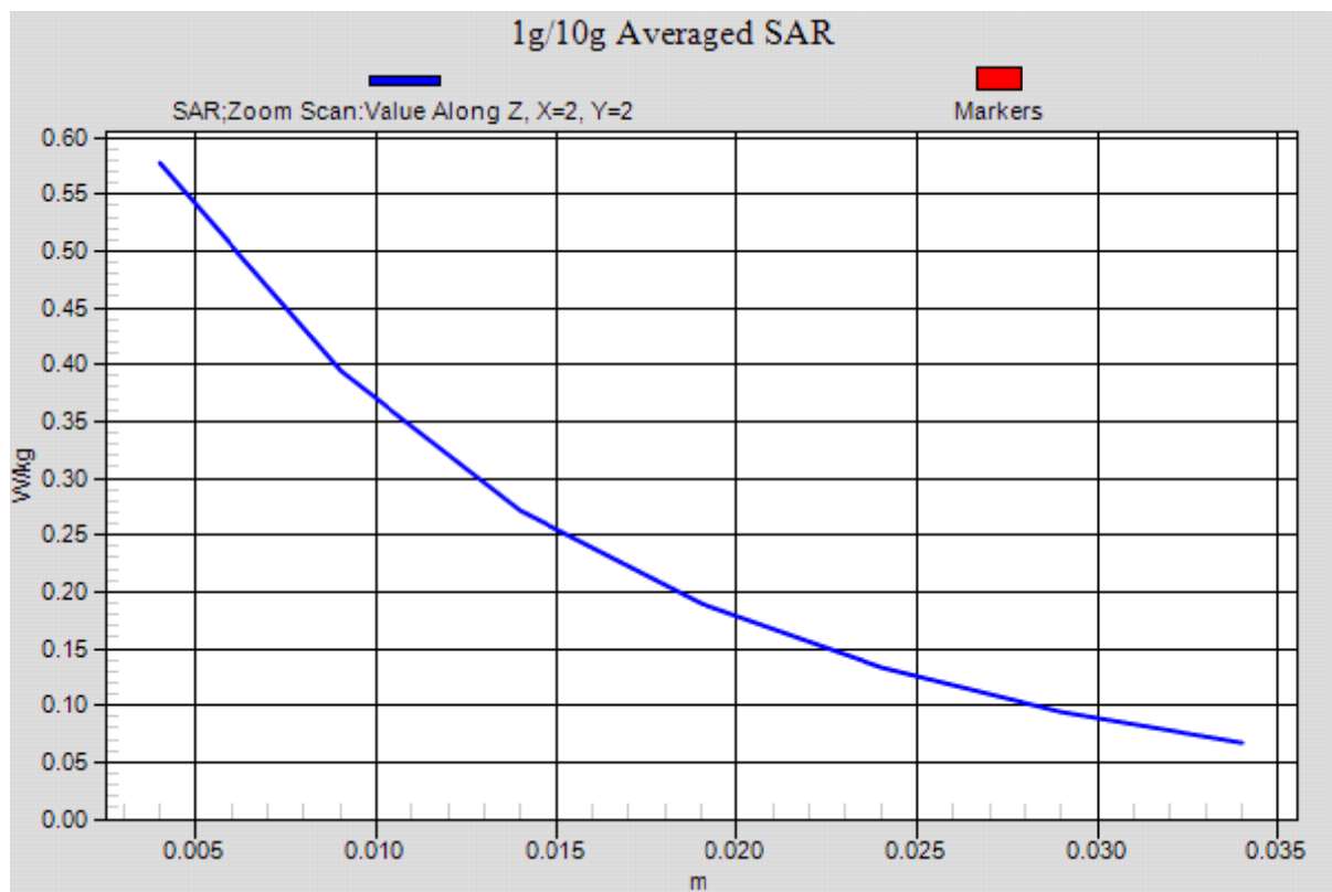
Figure 106 LTE Band 12 with Test Position 1 Channel 23095
