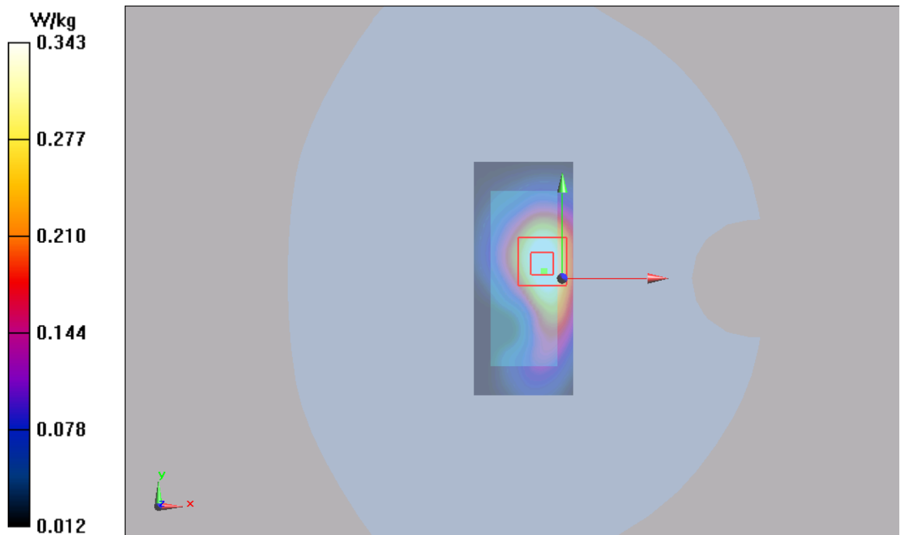
Figure 37 UMTS Band IV with Test Position 2 Channel 1413
