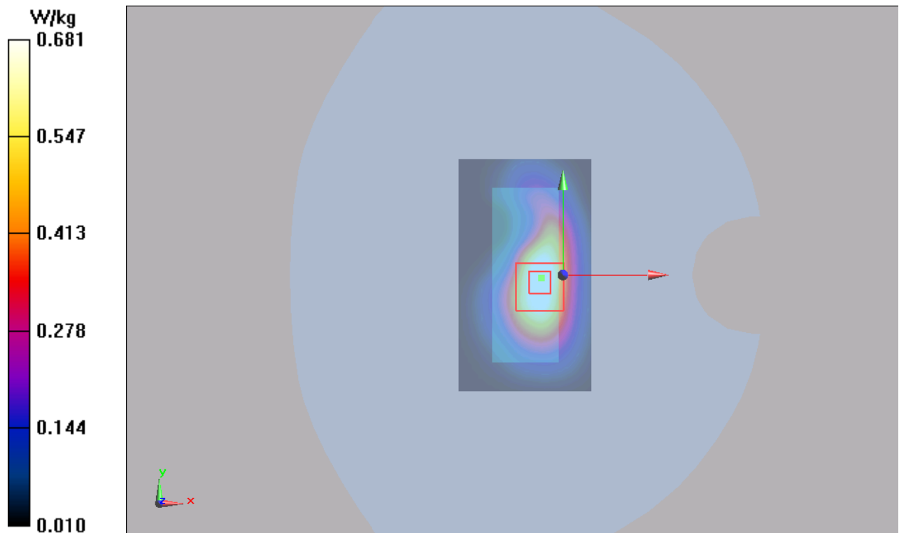
Figure 68 LTE Band 4 with Test Position 1 Channel 20050
