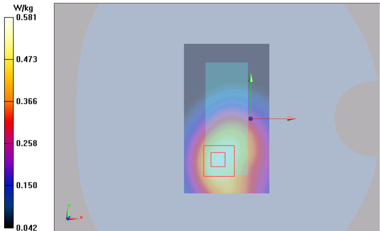
Figure 100 LTE Band 12 with Test Position 1 Channel 23095
