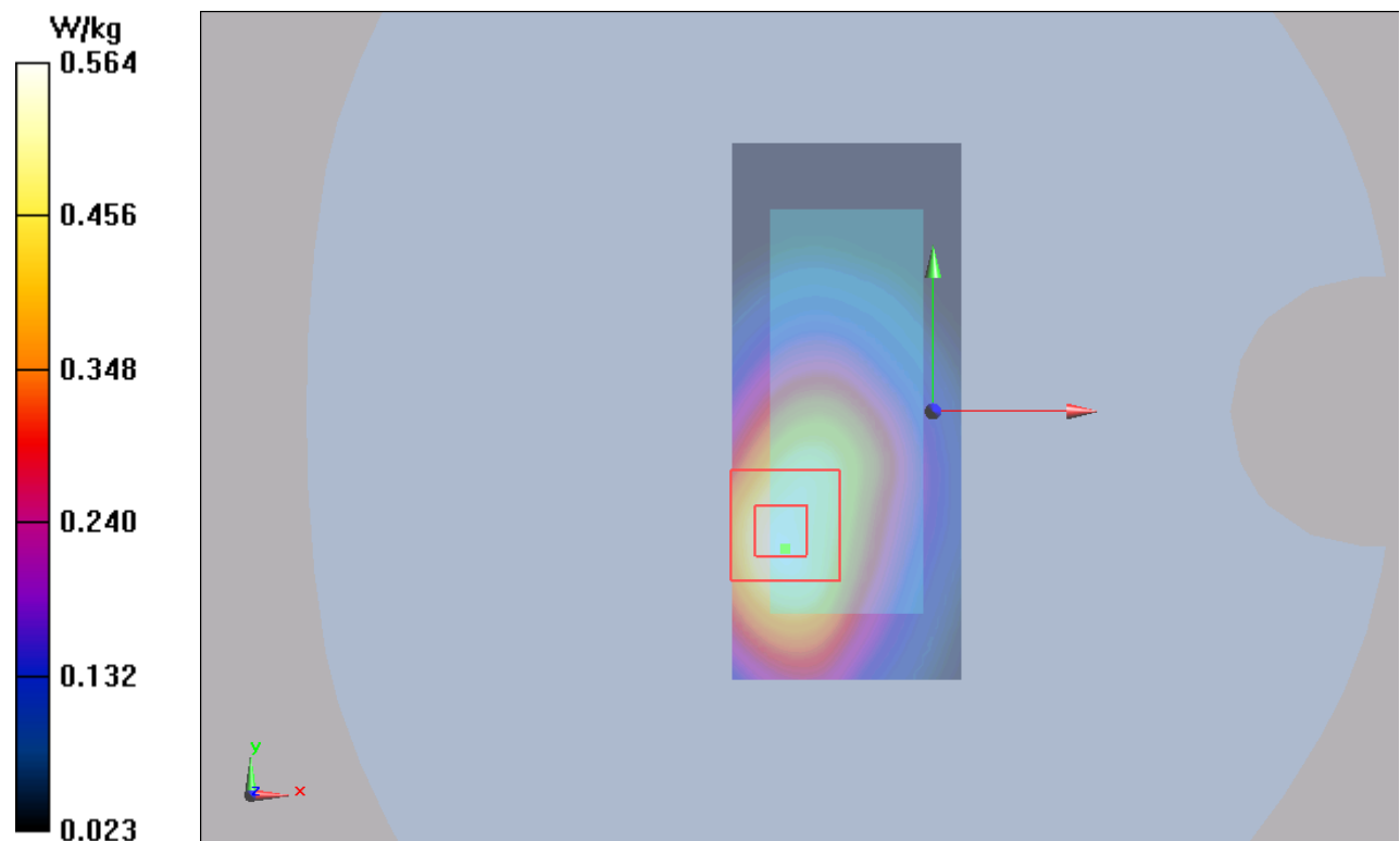
Figure 42 UMTS Band V with Test Position 1 Channel 4132
