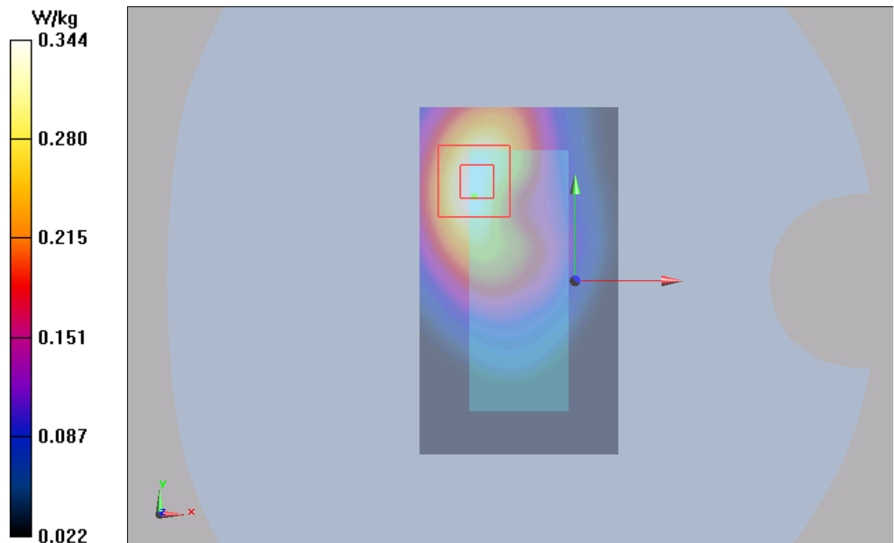
Figure 120 LTE Band 17 with Test Position 2 Channel 23780
