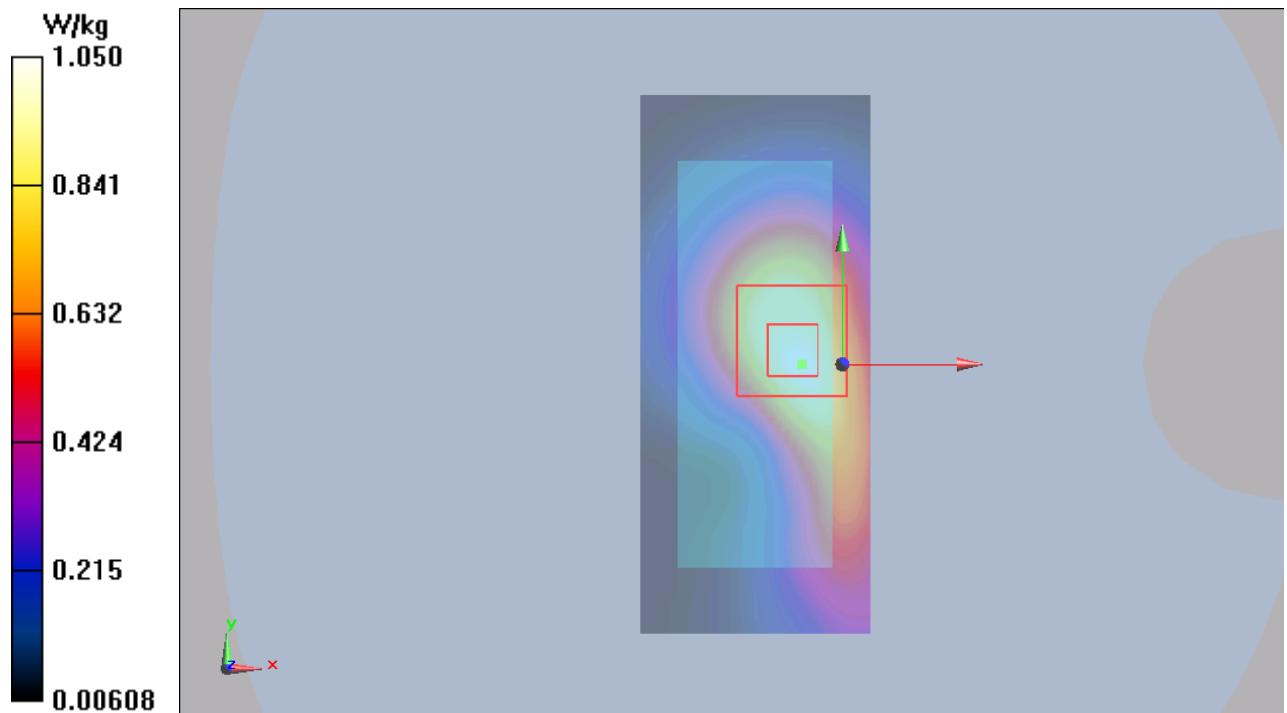
Figure 50 LTE Band 2 with Test Position 2 Channel 18900
