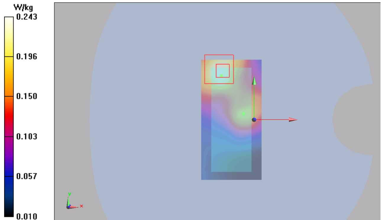
Figure 102 LTE Band 12 with Test Position 2 Channel 23060
