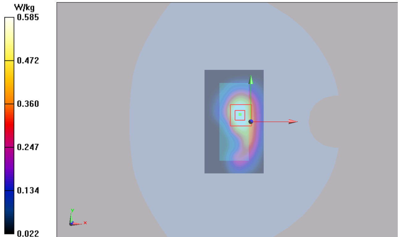
Figure 66 LTE Band 4 with Test Position 1 Channel 20300
