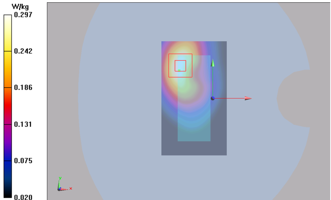
Figure 118 LTE Band 17 with Test Position 2 Channel 23800
