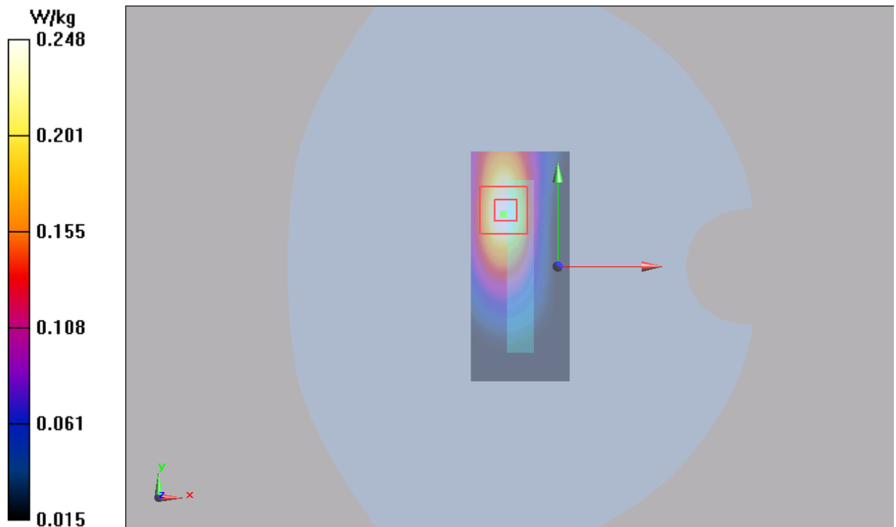
Figure 89 LTE Band 5 with Test Position 3 Channel 20525
