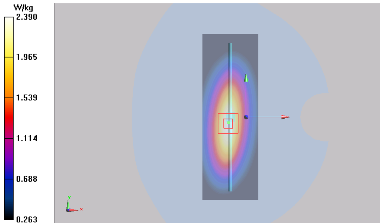
Figure 6 System Performance Check 750MHz 250mW
