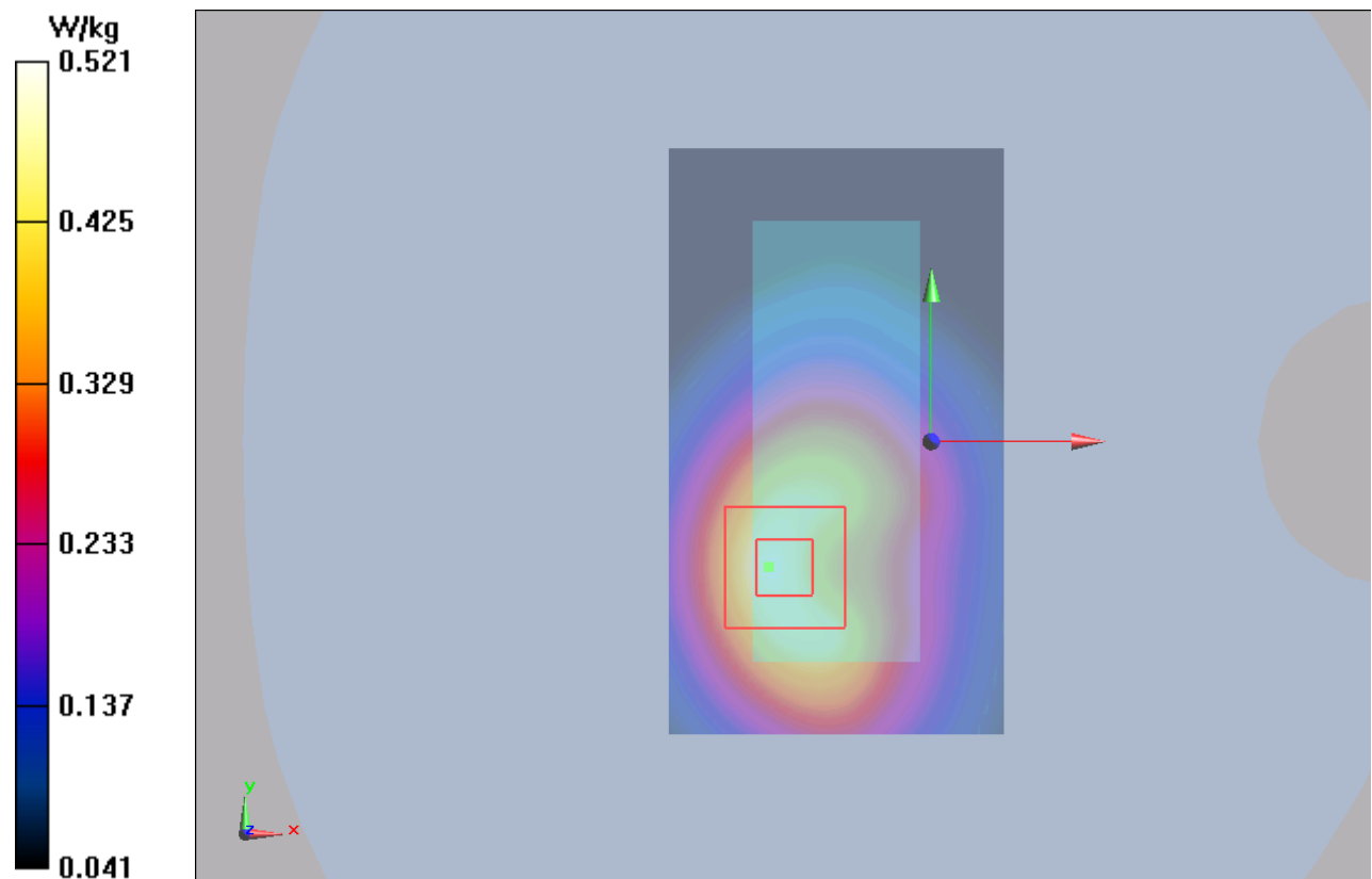
Figure 99 LTE Band 12 with Test Position 1 Channel 23130
