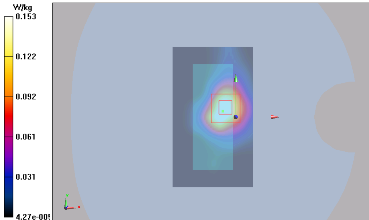
Figure 123 802.11b Test Position 1 Channel 6
