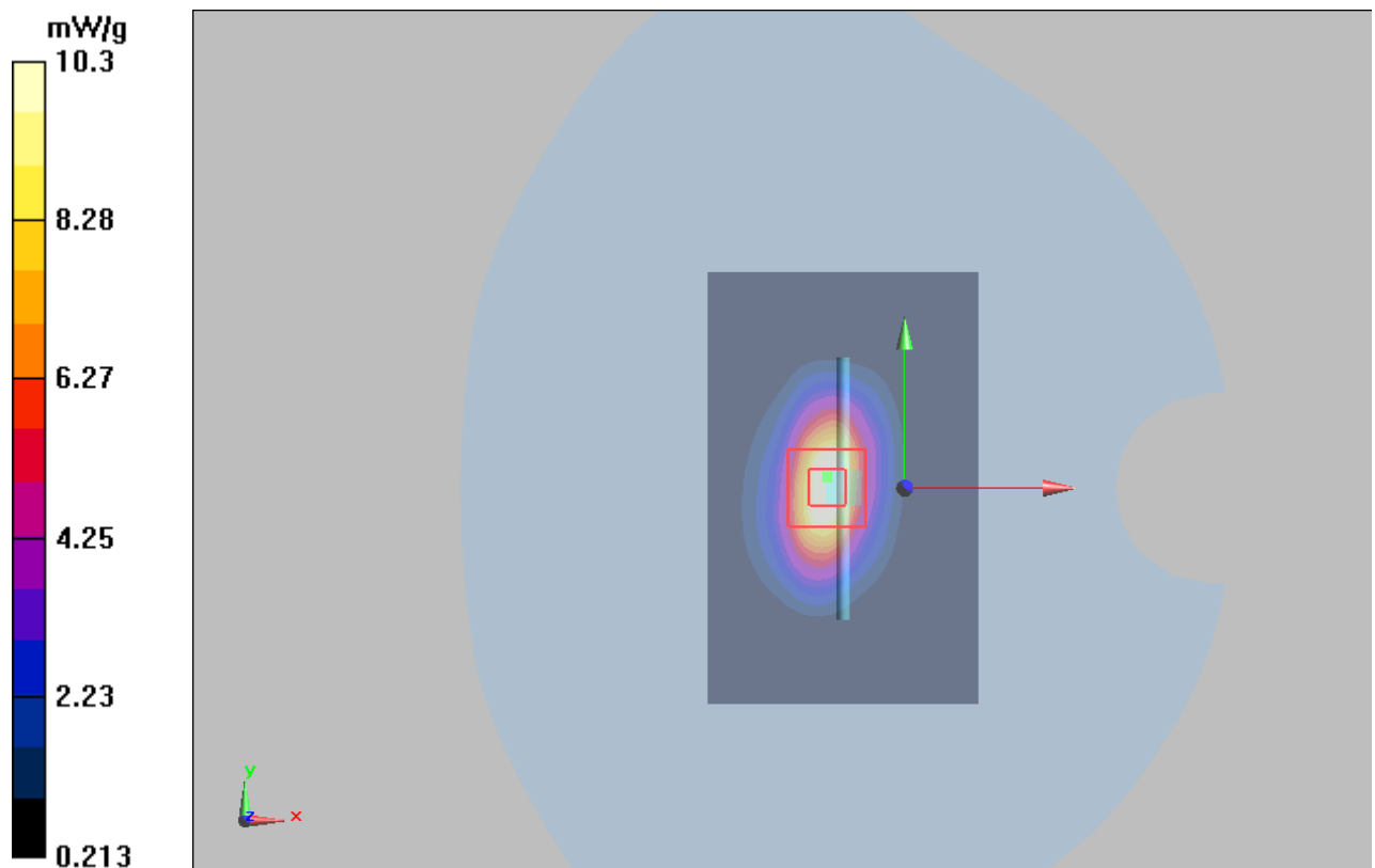
Figure 9 System Performance Check 1750MHz 250mW
