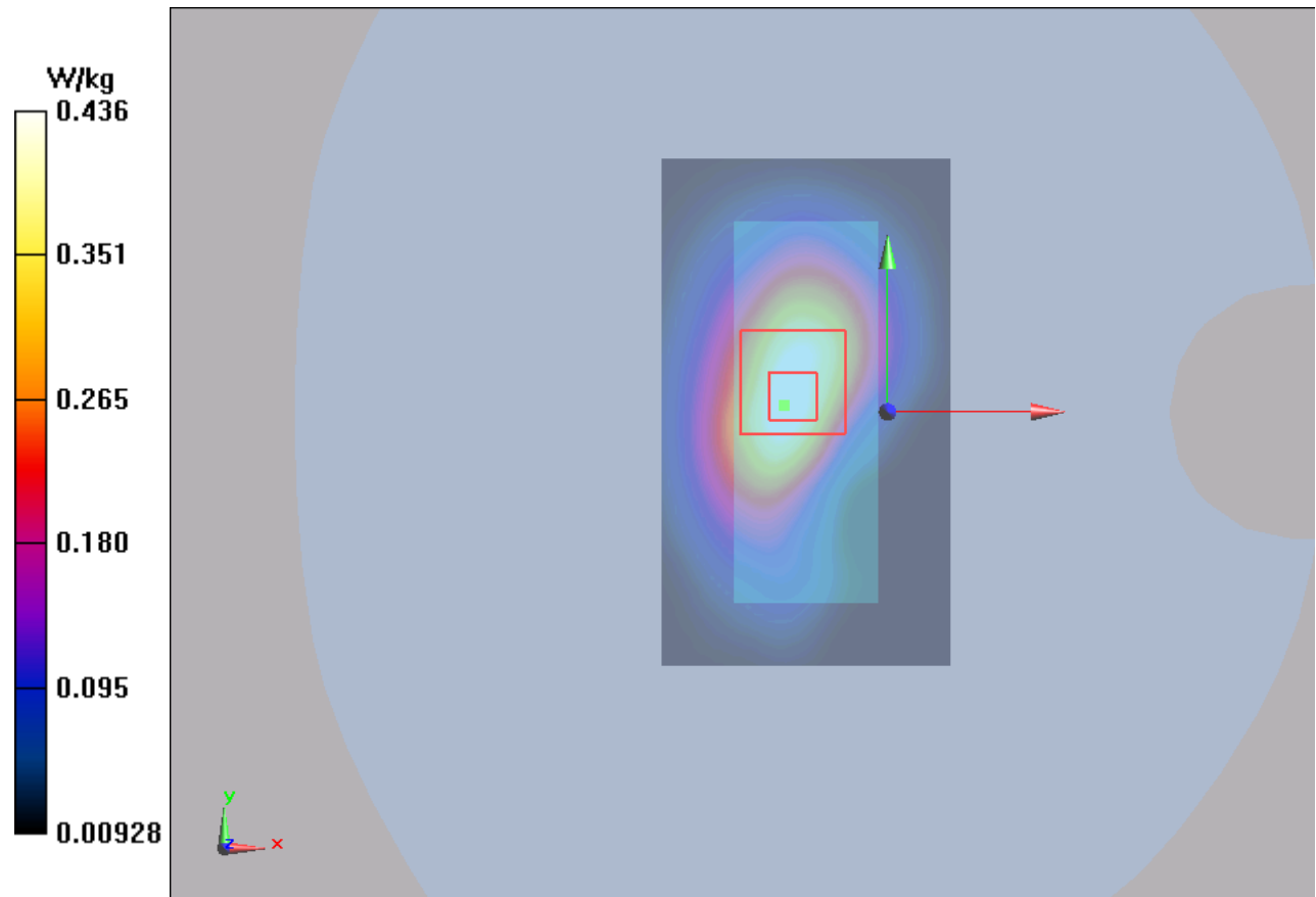
Figure 74 LTE Band 4 with Test Position 1 Channel 20050
