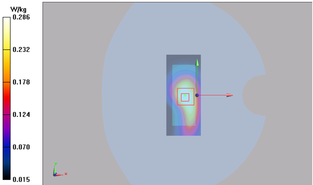
Figure 31 UMTS Band II with Test Position 2 Channel 9400
