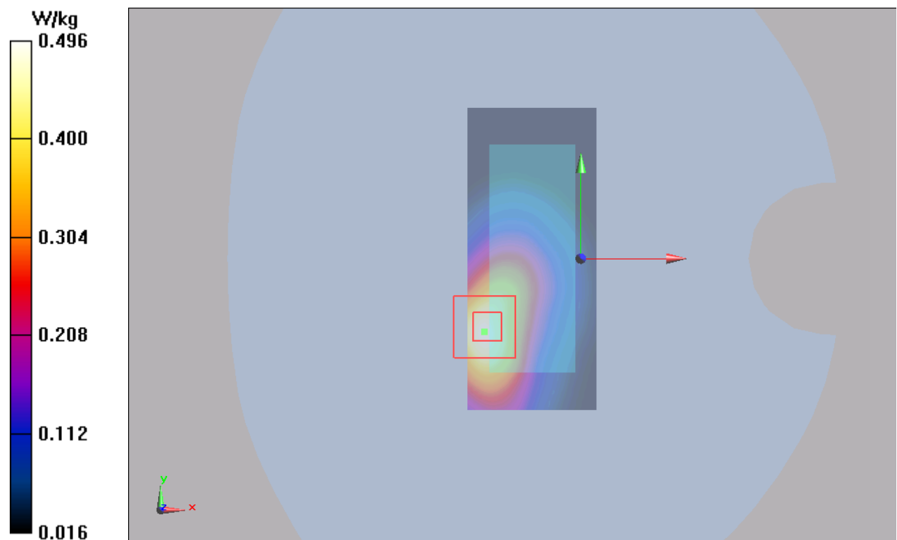
Figure 14 GSM 850 GPRS (2TXslots) with Test Position 1 Channel 251
