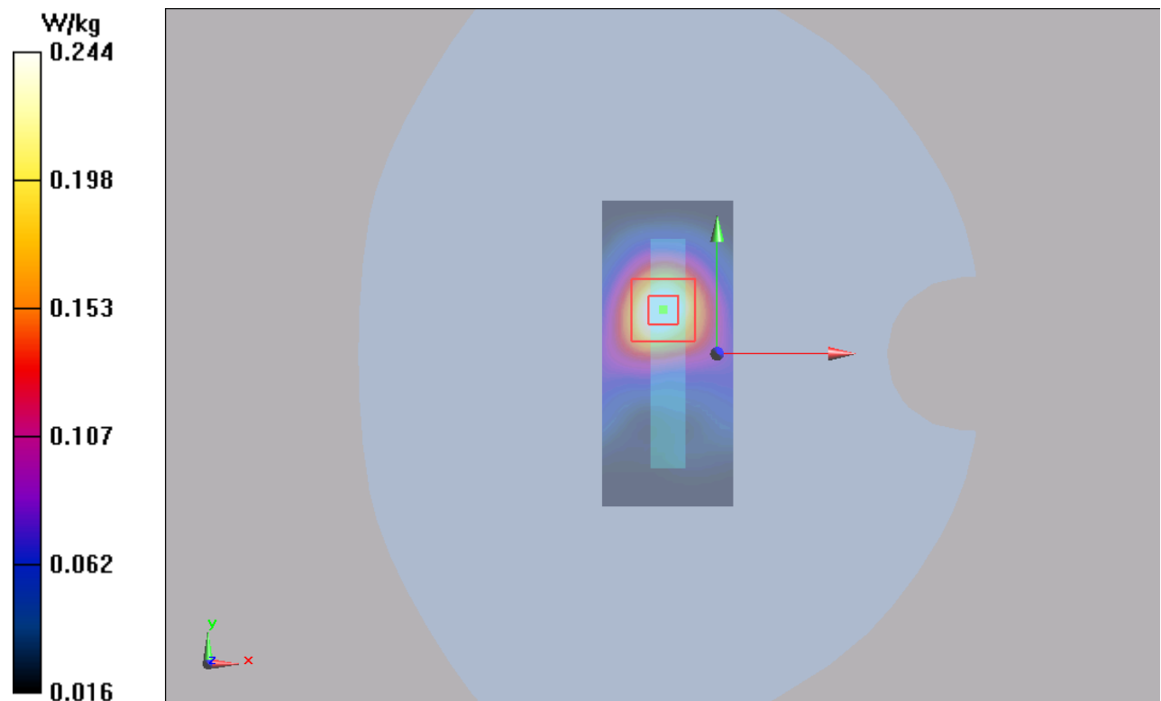
Figure 61 LTE Band 2 with Test Position 4 Channel 18900
