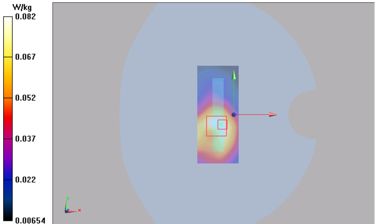
Figure 26 GSM 1900 GPRS (2TXslots) with Test Position 4 Channel 661
