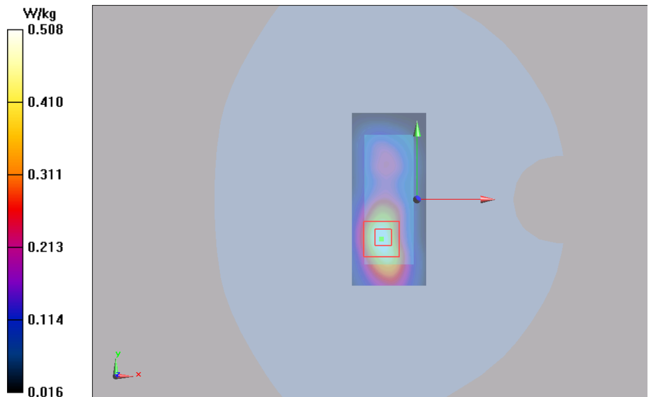
Figure 22 GSM 1900 GPRS (2TXslots) with Test Position 1 Channel 661
