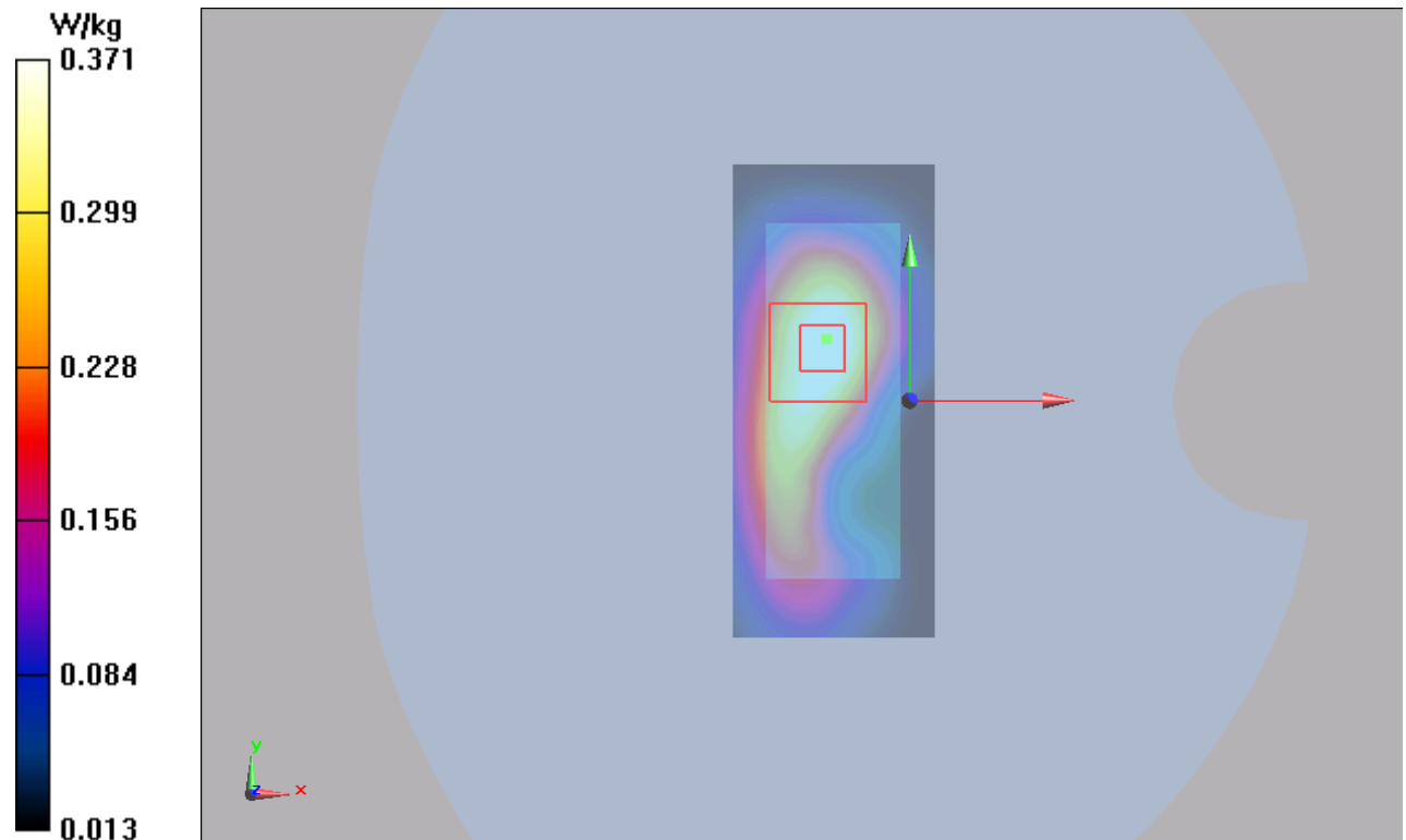
Figure 28 UMTS Band II with Test Position 1 Channel 9538
