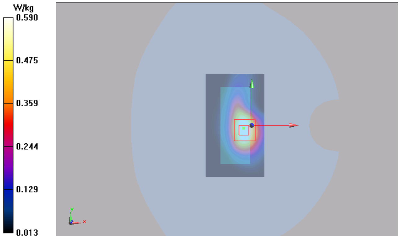
Figure 69 LTE Band 4 with Test Position 2 Channel 20050
