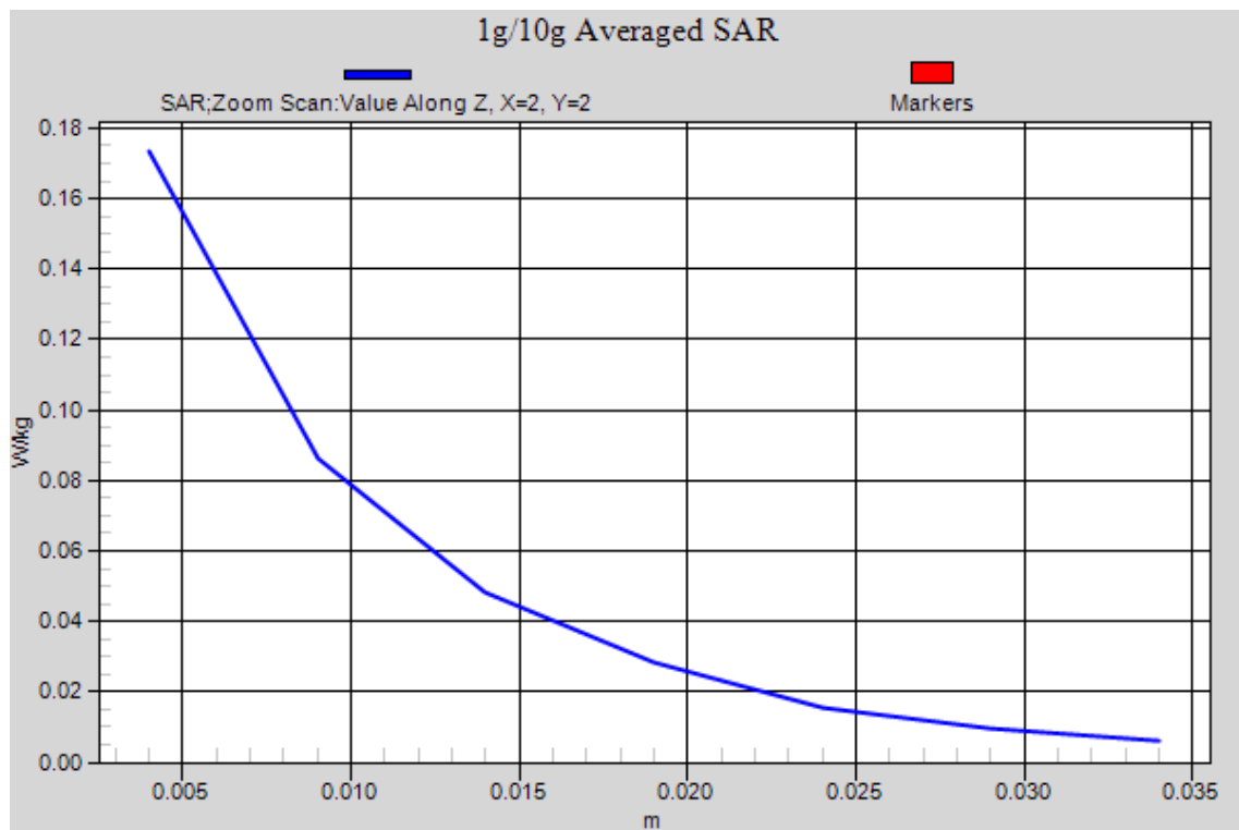
Figure 125 802.11b Test Position 2 Channel 6
