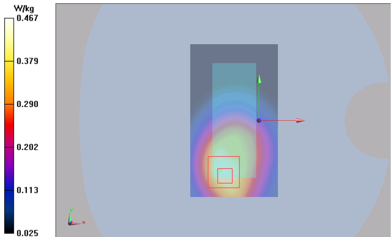
Figure 112 LTE Band 17 with Test Position 1 Channel 23790
