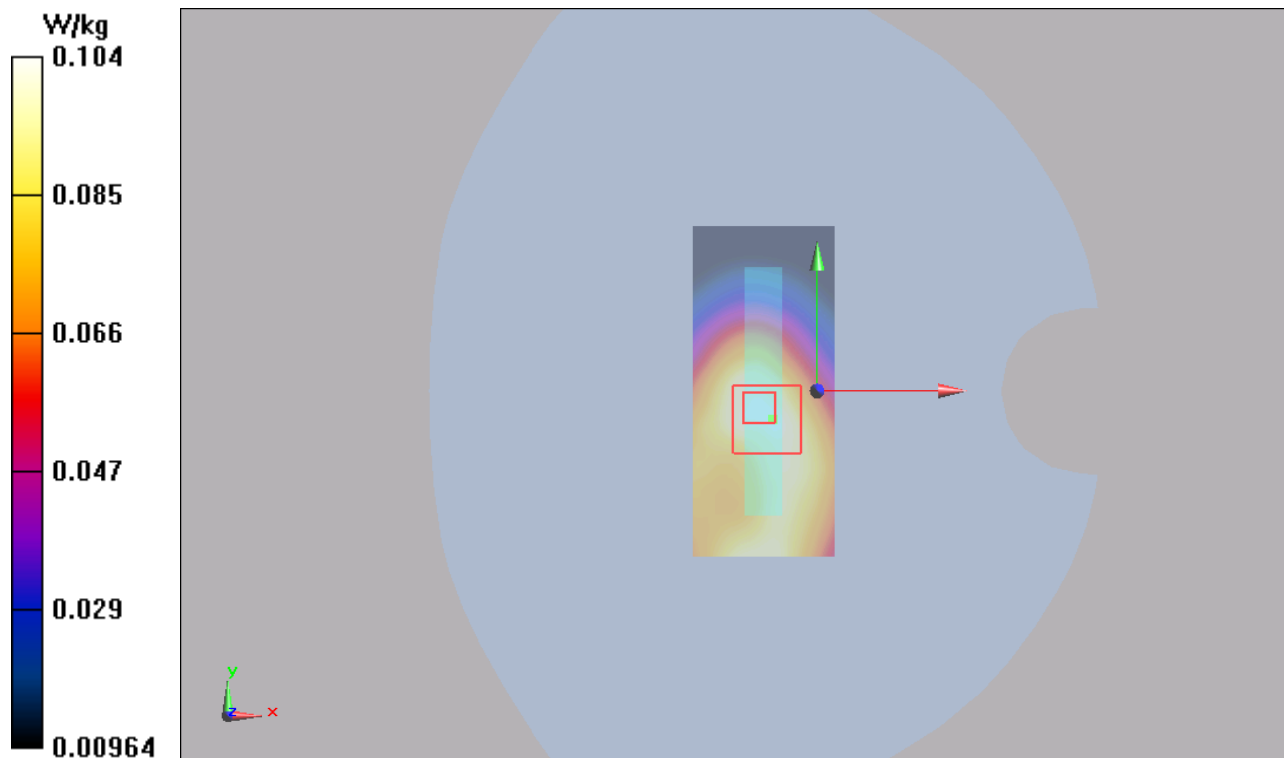
Figure 90 LTE Band 5 with Test Position 4 Channel 20525
