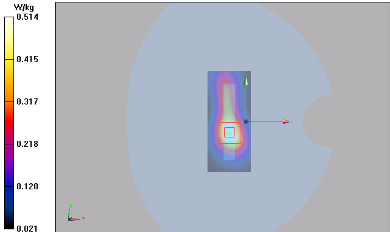
Figure 52 LTE Band 2 with Test Position 3 Channel 19100
