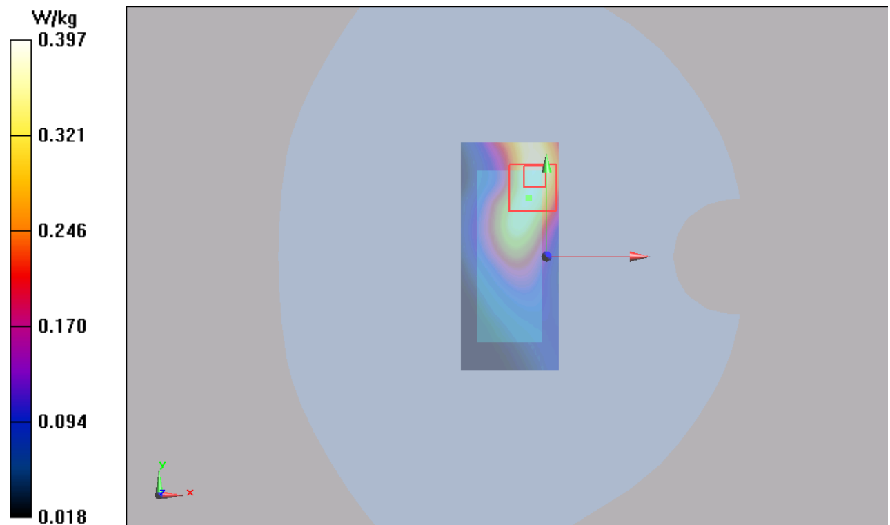
Figure 86 LTE Band 5 with Test Position 1 Channel 20525
