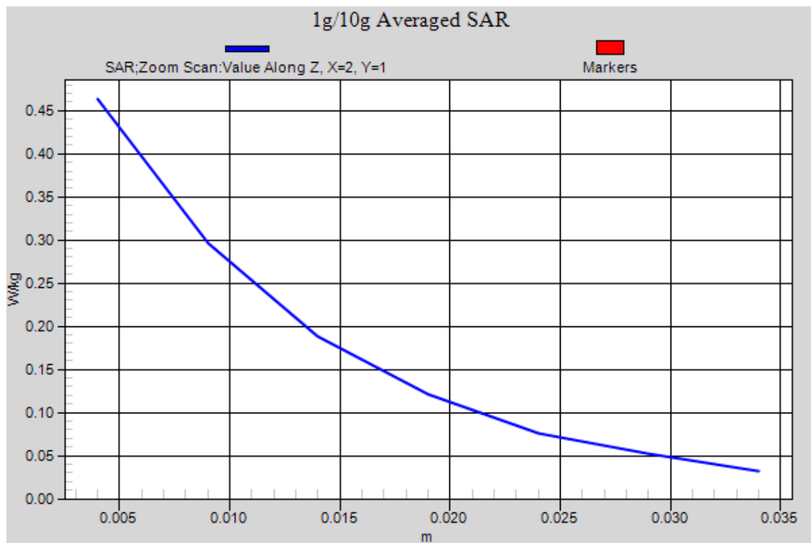
Figure 94 UMTS Band IV with Test Position 1 Channel 1413
