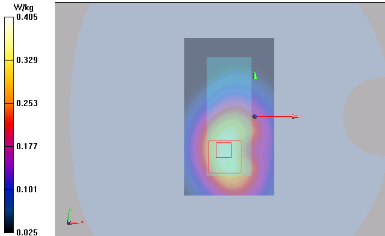
Figure 105 LTE Band 12 with Test Position 1 Channel 23130
