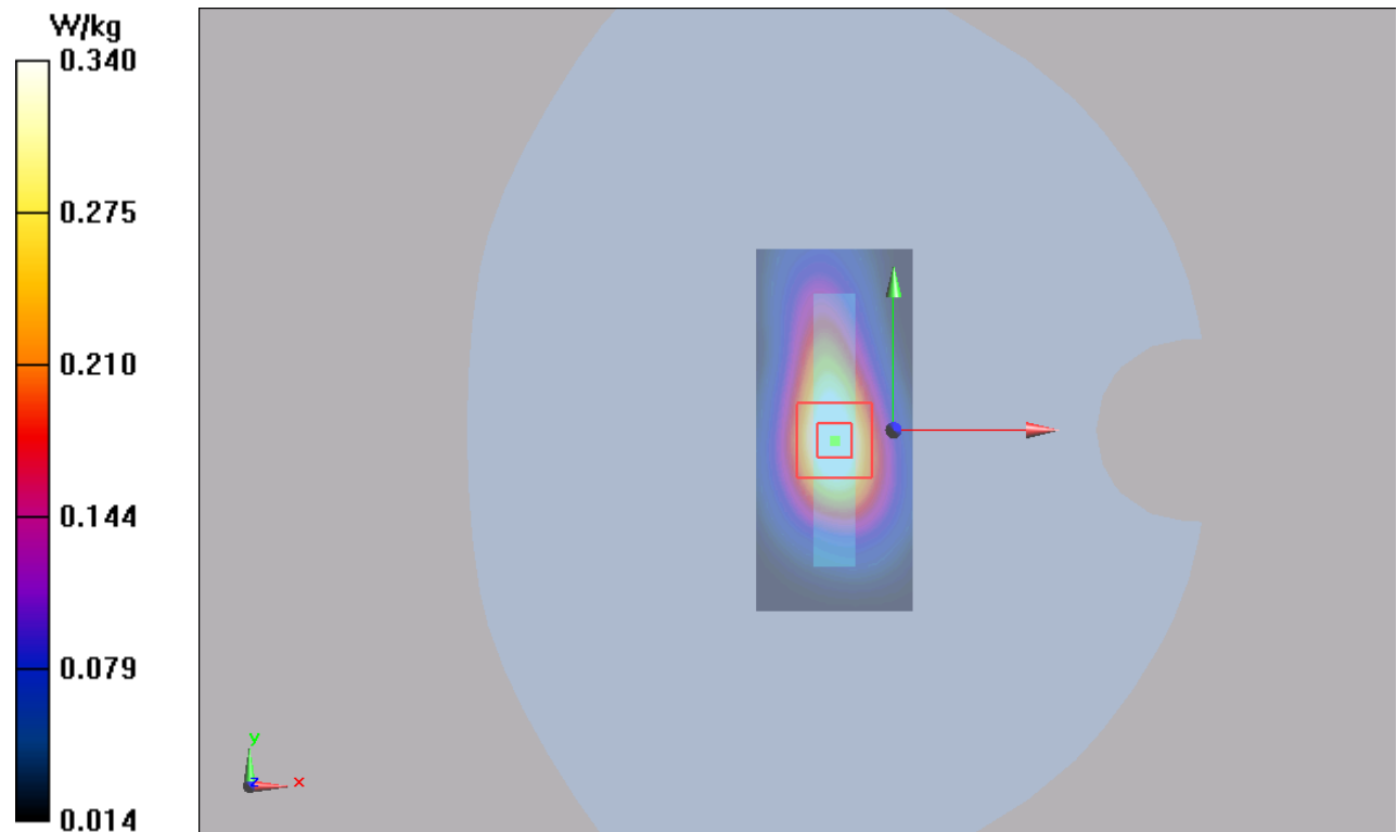
Figure 54 LTE Band 2 with Test Position 3 Channel 18700
