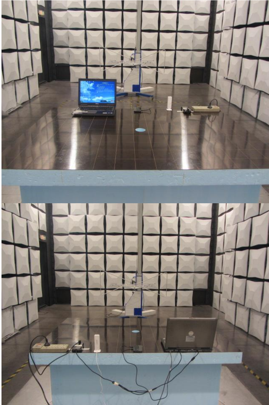
Radiated Spurious Emission (below 1GHz)
