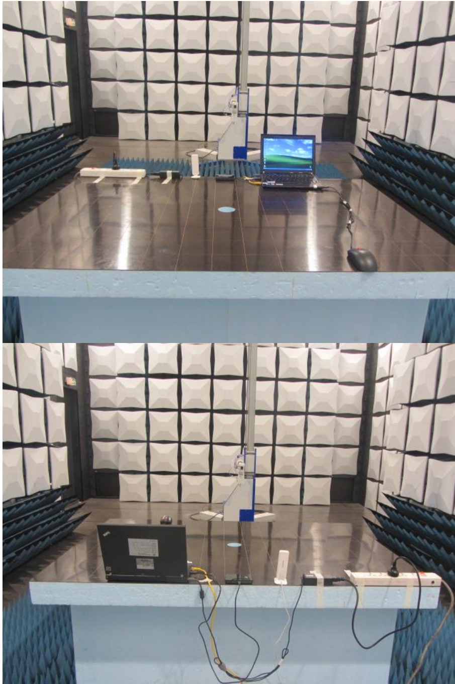
Radiated Spurious Emission (above 18GHz)
