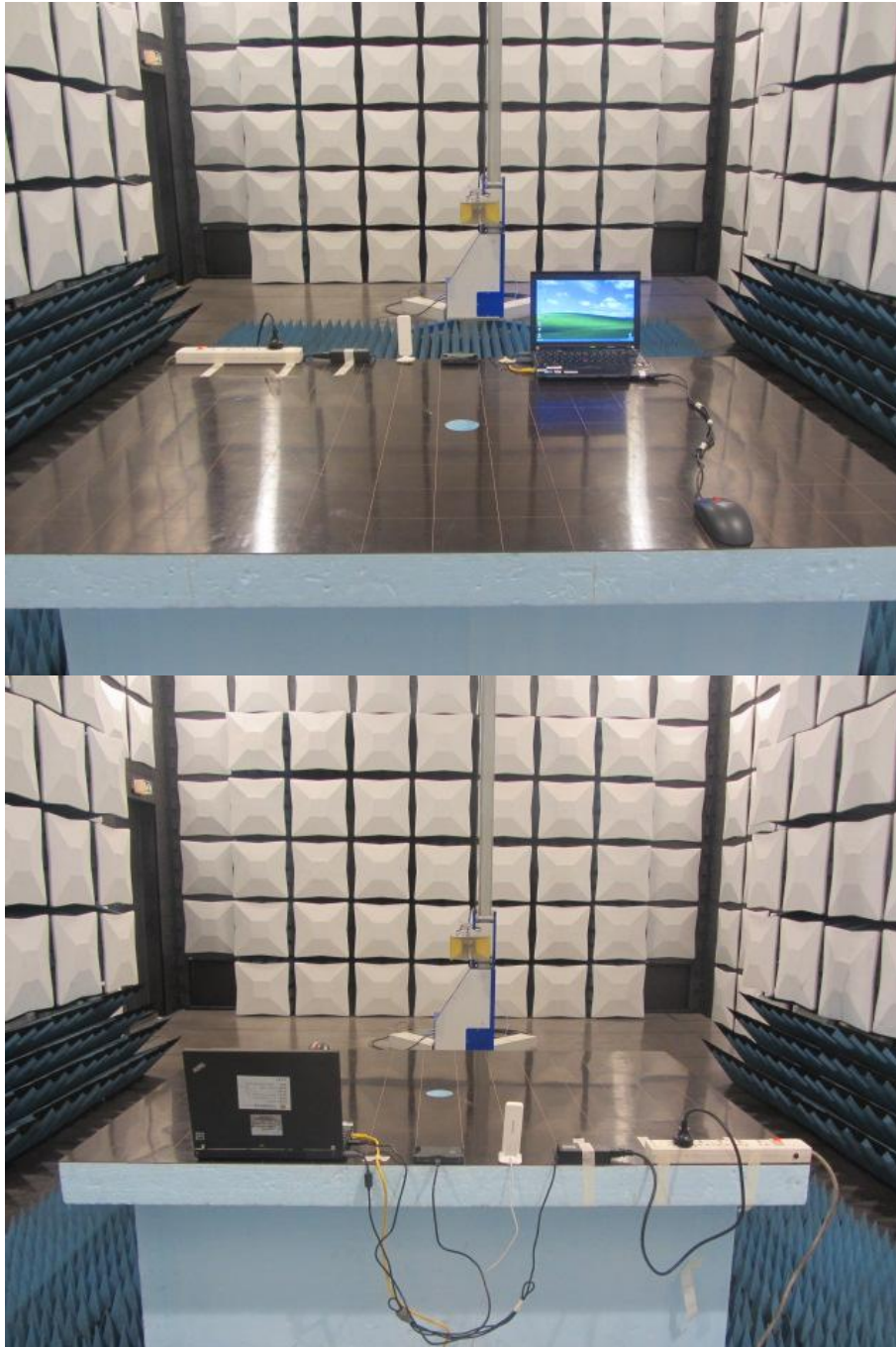
Radiated Spurious Emission (1GHz to18GHz)
