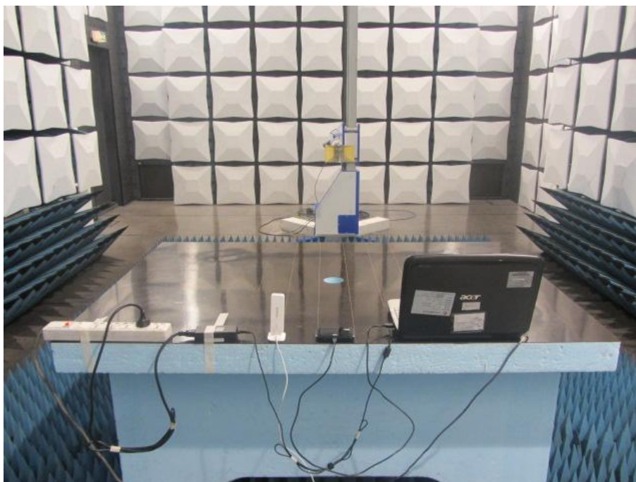
Receiver Spurious Emissions (above 1GHz)
