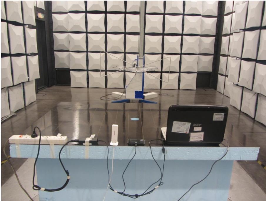
Receiver Spurious Emissions (30MHz-1GHz)
