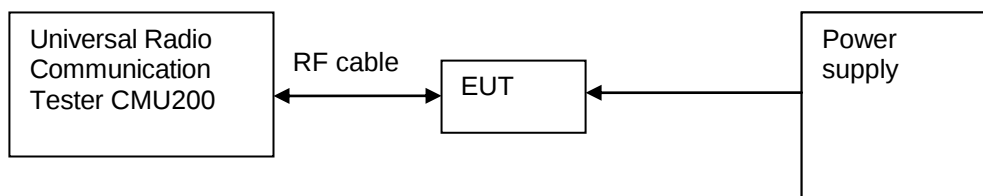
Figure 4. Test Set-up
