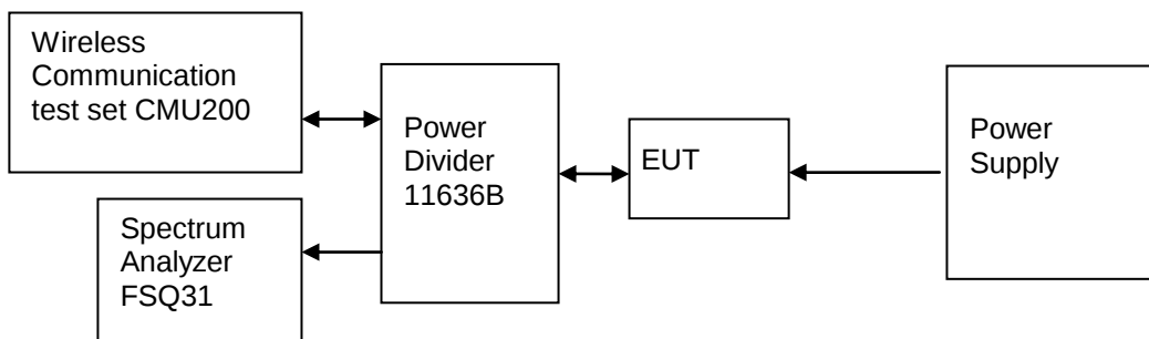
Figure 5. Test Set-up
