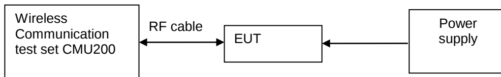
Figure 8. Test Set-up
