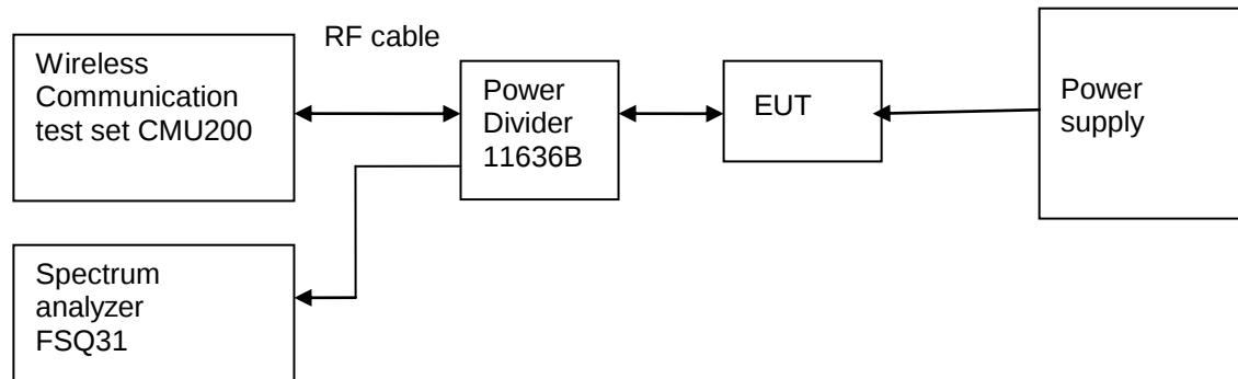
Figure 7. Test Set-up
