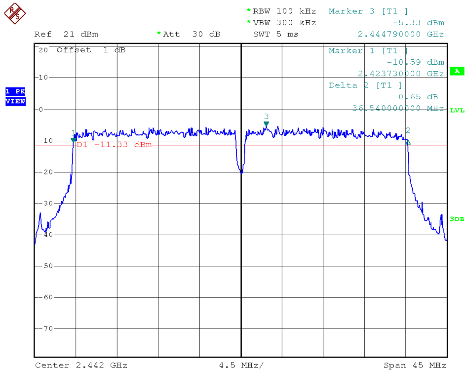
Antenna A - Channel 7 / 6 dB Bandwidth
