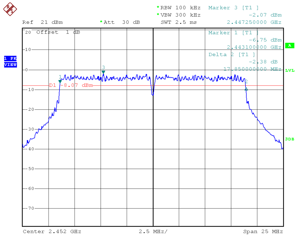
Antenna A - Channel 9 / 6 dB Bandwidth
