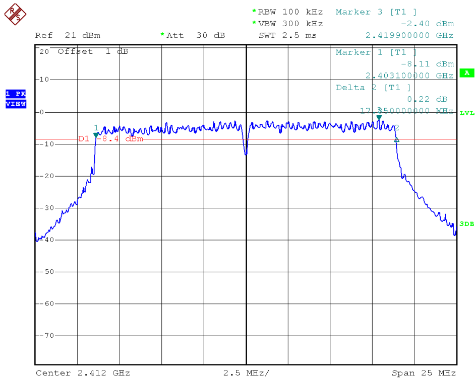
Antenna A - Channel 1 / 6 dB Bandwidth
