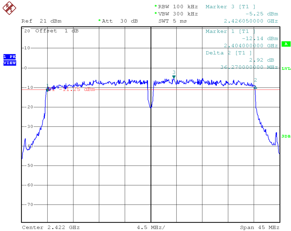
Antenna B - Channel 3 / 6 dB Bandwidth
