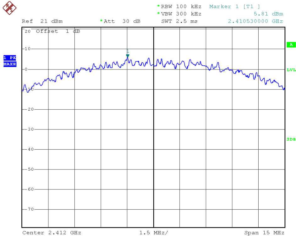
(Plot 2.5 A2: Channel = 1 @ 802.11b)
