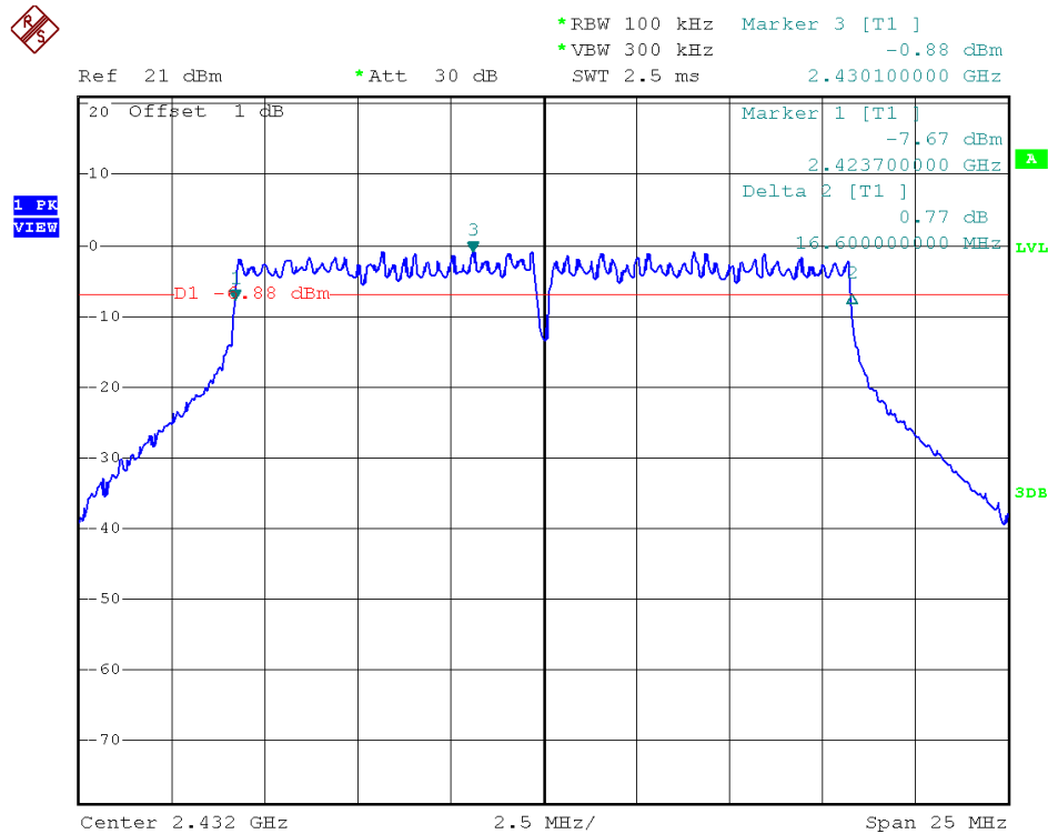
Antenna B - Channel 5/ 6 dB Bandwidth
