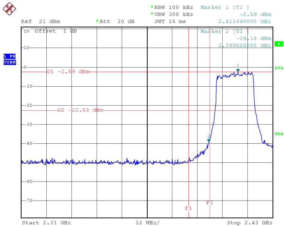
Antenna A Channel = 1 @ 802.11n-20
