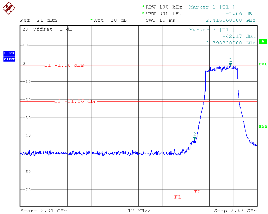
Antenna B Channel = 1 @ 802.11g
