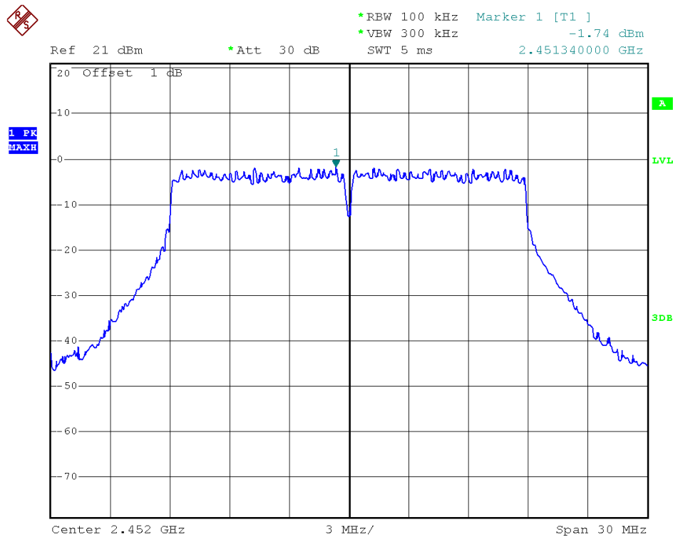
(Plot 2.5 I2: Channel = 9 @ 802.11n-20
