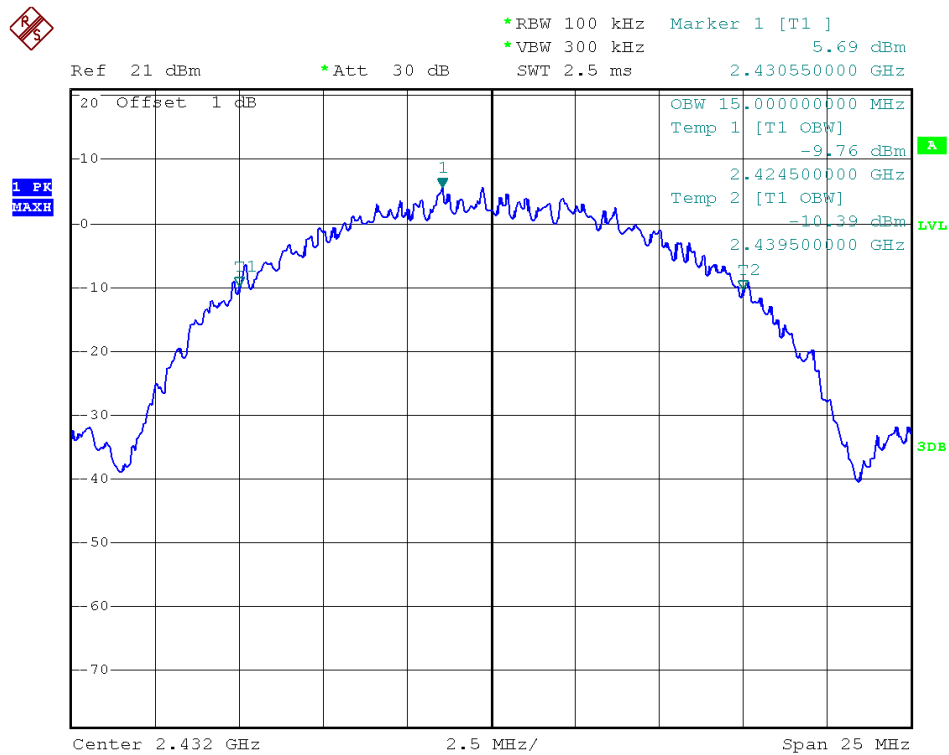
Antenna A - Channel 5 / 99% Occupied Bandwidth
