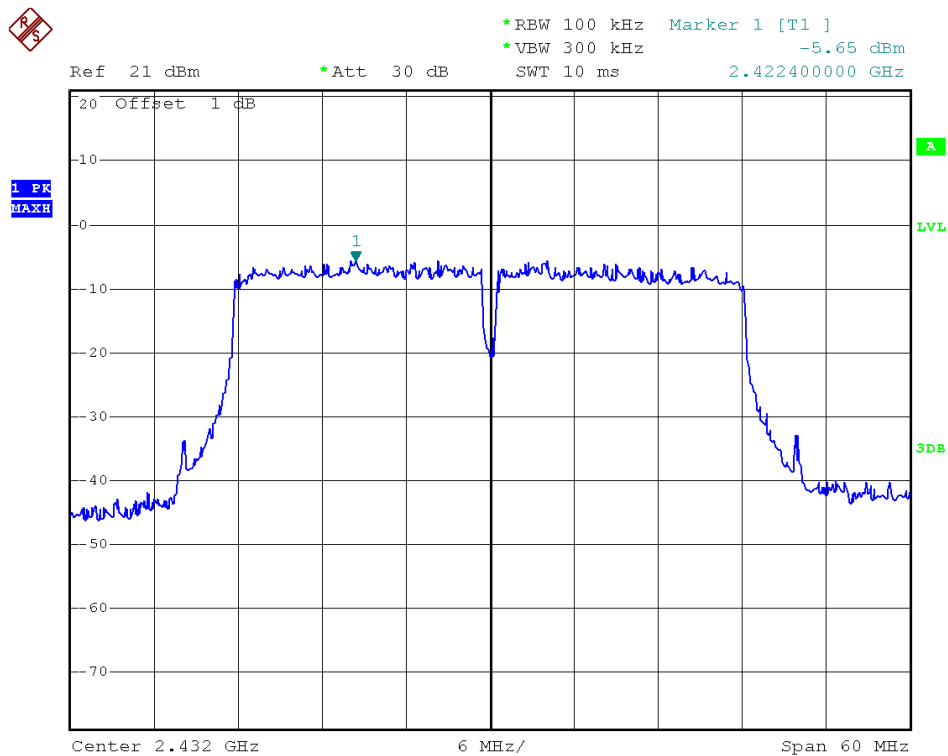
(Plot 2.5 K1: Channel = 5 @ 802.11n-40)
