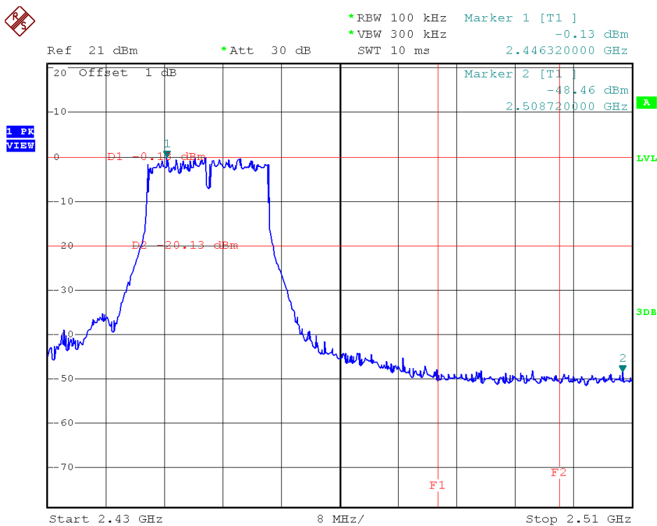
Antenna B Channel = 9 @ 802.11g
