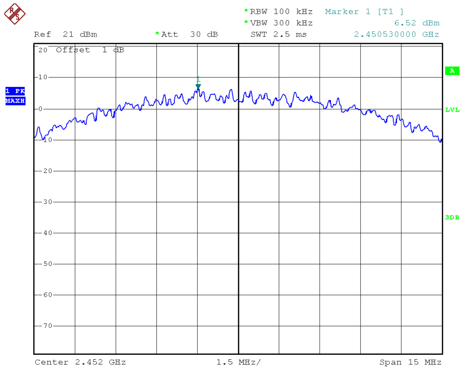
(Plot 2.5 C1: Channel = 9 @ 802.11b)
