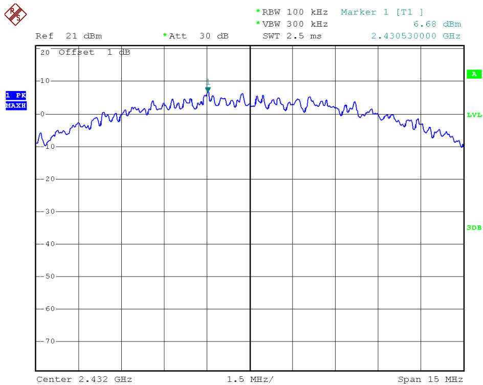
(Plot 2.5 B2: Channel = 5 @ 802.11b)
