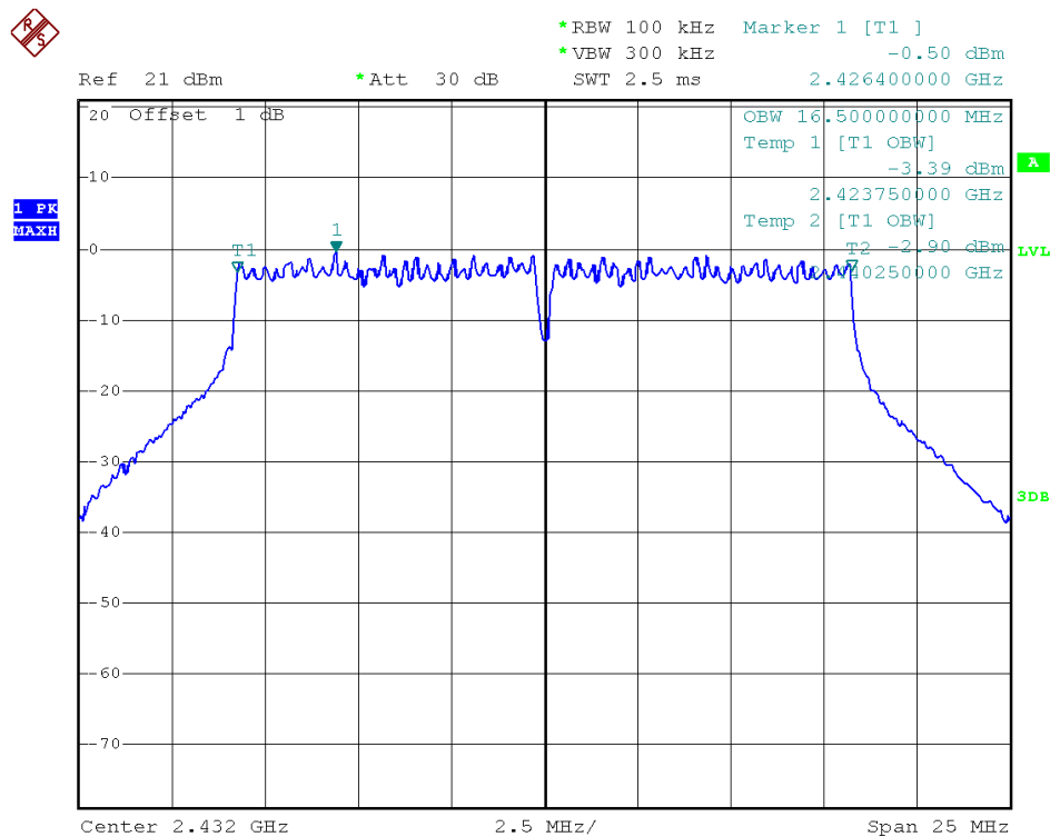
Antenna B - Channel 5 / 99% Occupied Bandwidth
