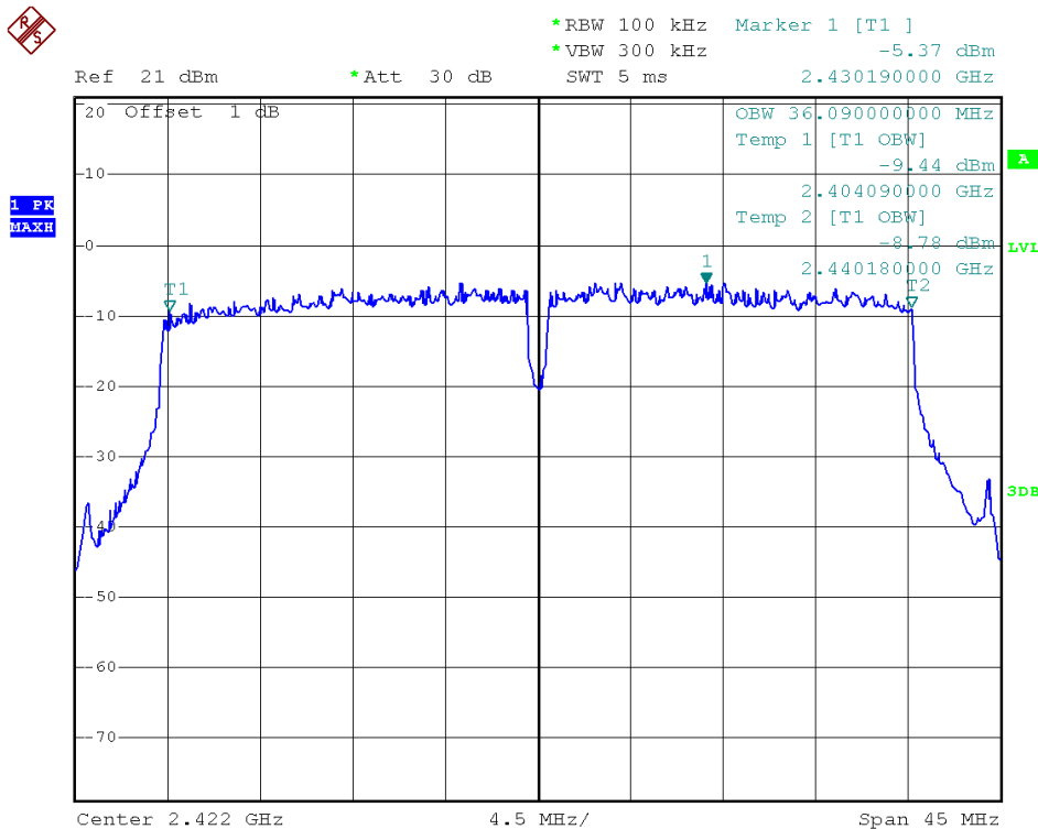
Antenna B - Channel 3 / 99% Occupied Bandwidth
