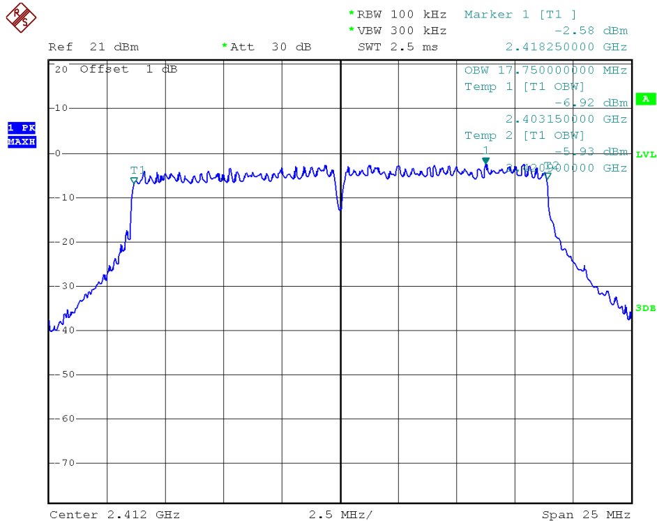
Antenna A - Channel 1 / 99% Occupied Bandwidth
