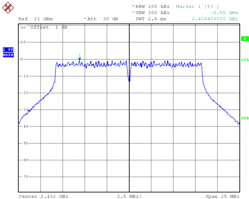
(Plot 2.5 E2: Channel = 5 @ 802.11g)
