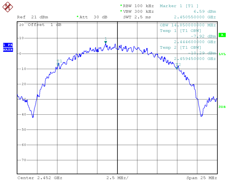
Antenna B - Channel 9 / 99% Occupied Bandwidth
