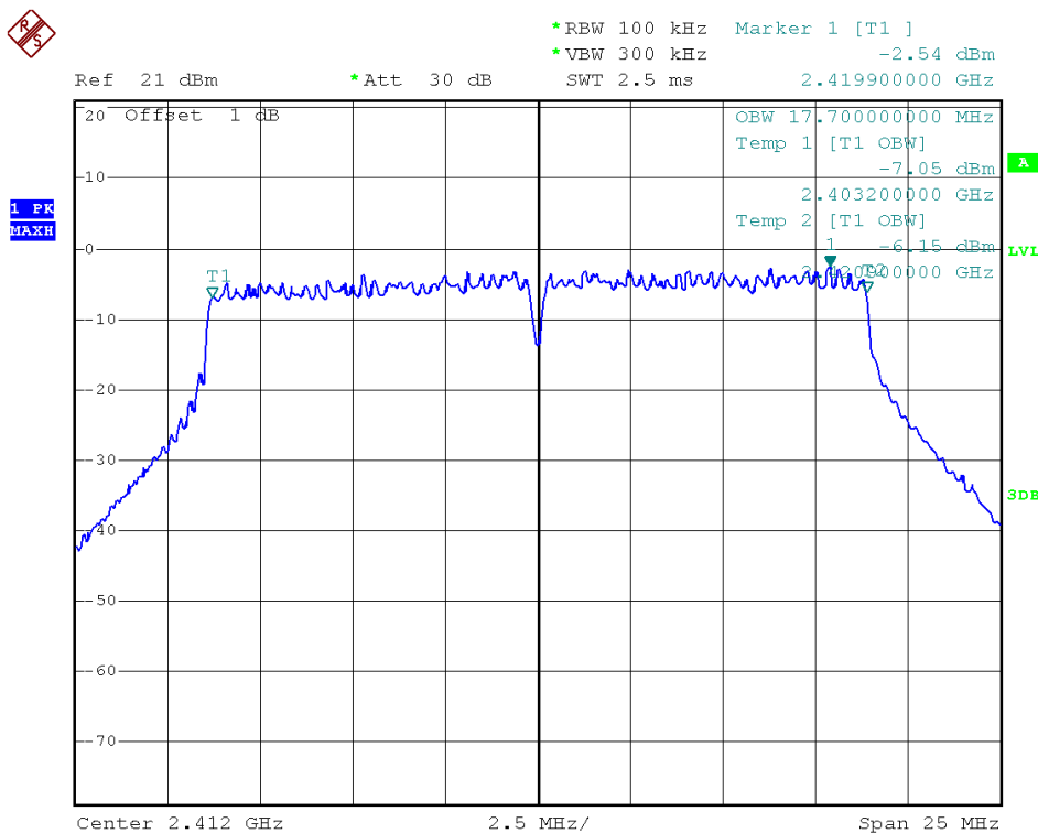
Antenna B - Channel 1/ 99% Occupied Bandwidth
