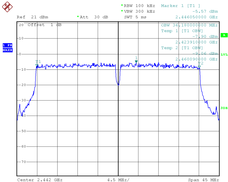
Antenna A - Channel 7 / 99% Occupied Bandwidth
