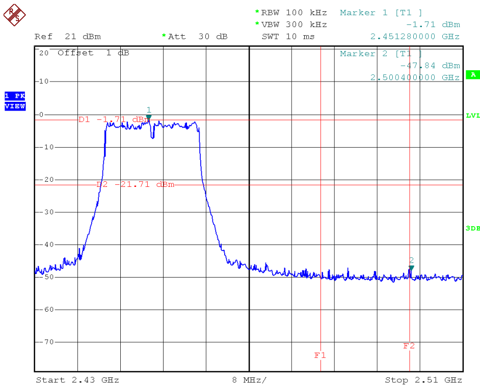
Antenna B Channel = 9 @ 802.11n-20
