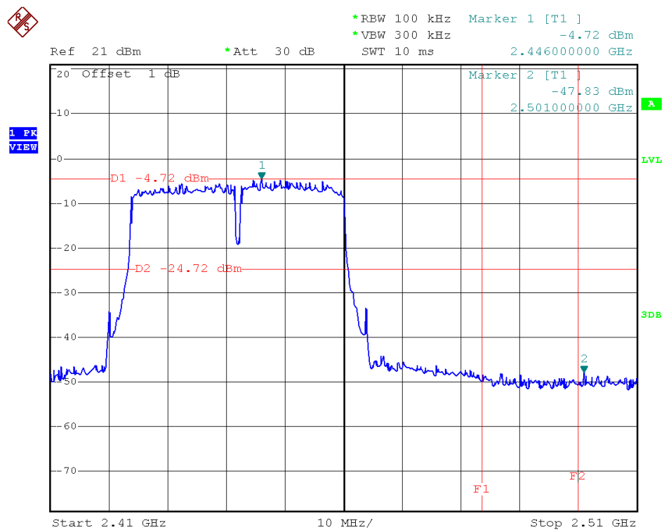
Antenna B Channel = 7 @ 802.11n-40
