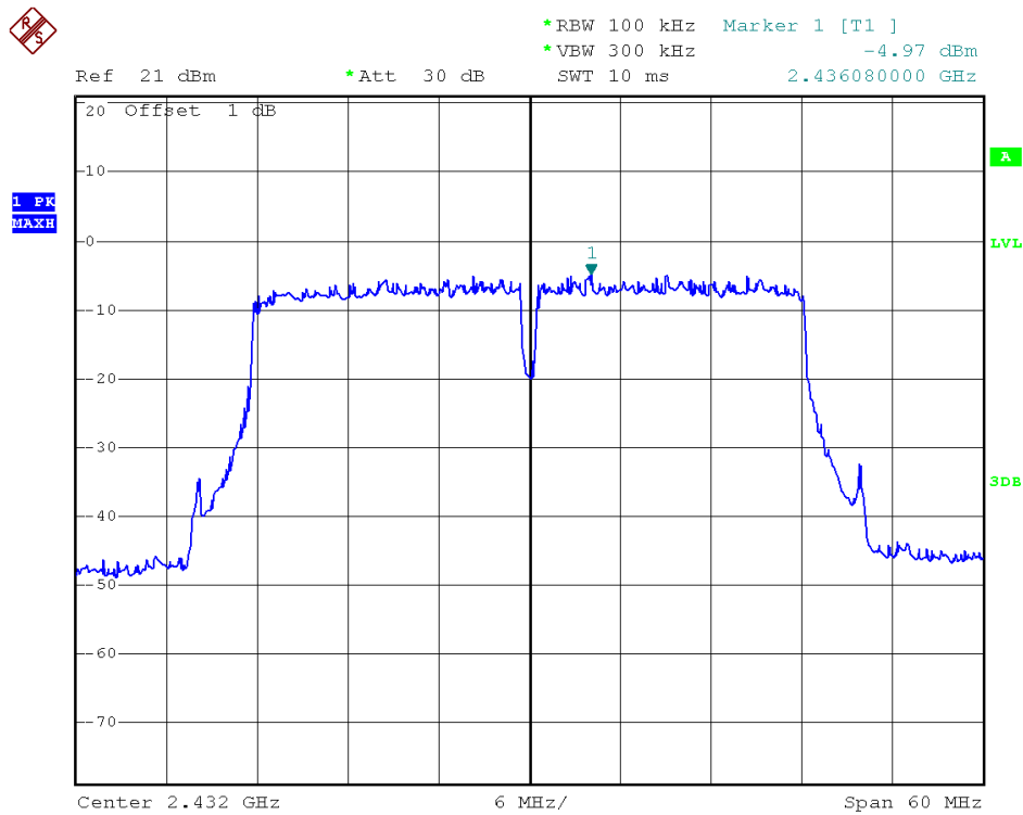
(Plot 2.5 K2: Channel = 5 @ 802.11n-40)
