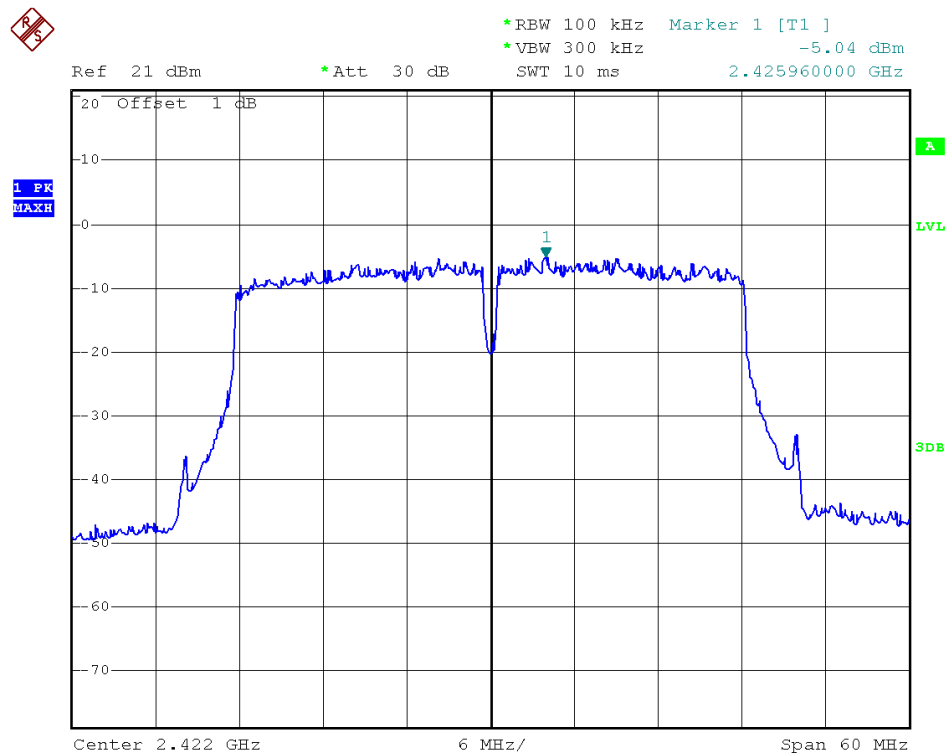
(Plot 2.5 J2: Channel = 3 @ 802.11n-40)
