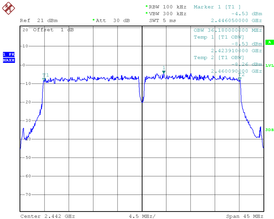
Antenna B - Channel 7 / 6 dB Bandwidth
