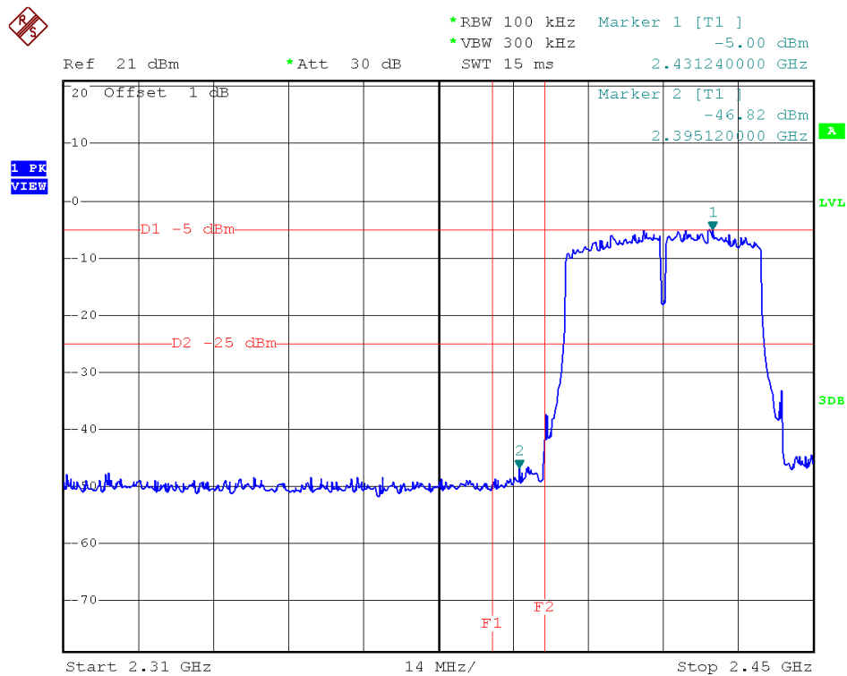
Antenna B Channel = 3 @ 802.11n-40
