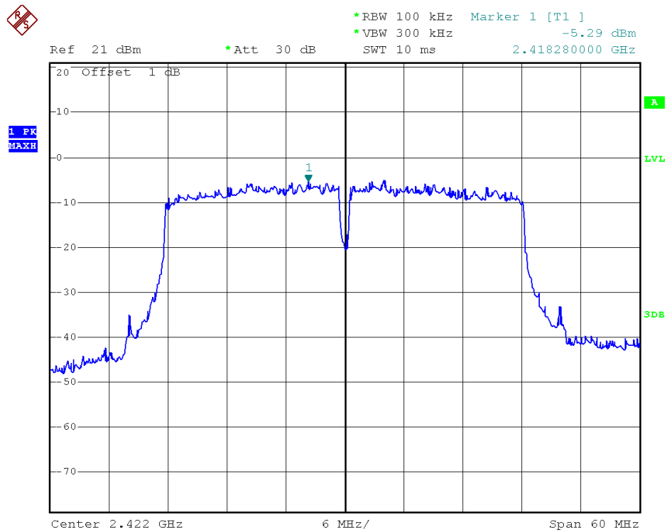
(Plot 2.5 J1: Channel = 3 @ 802.11n-40)
