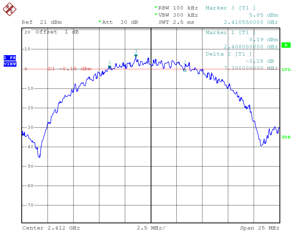
Antenna B - Channel 1 / 6 dB Bandwidth
