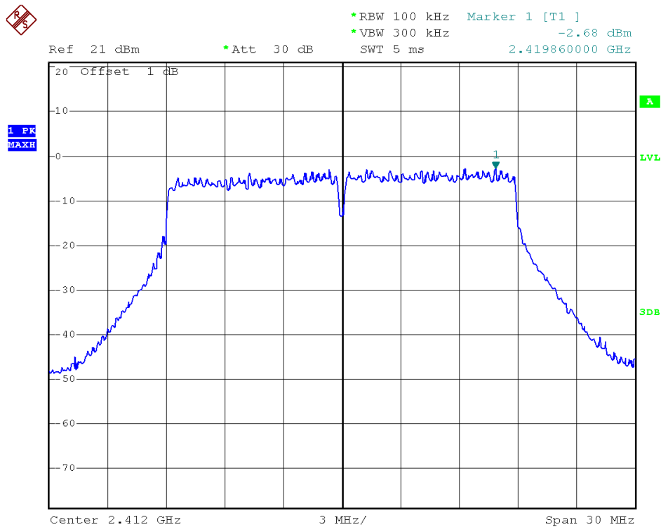
(Plot 2.5 G2: Channel = 1 @ 802.11n-20)
