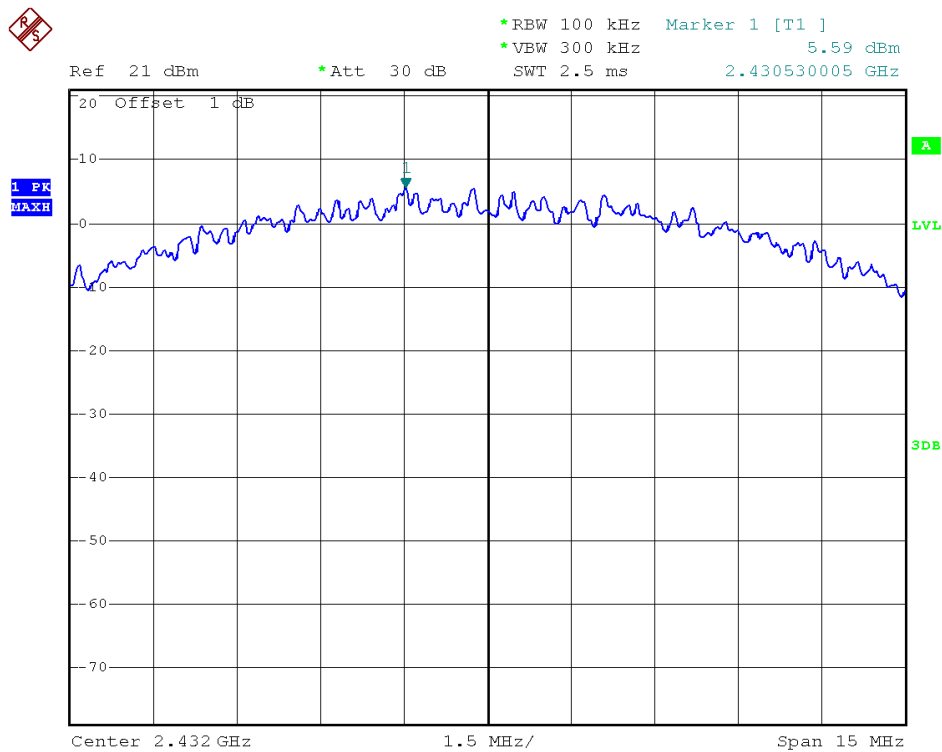
(Plot 2.5 B1: Channel = 5 @ 802.11b)
