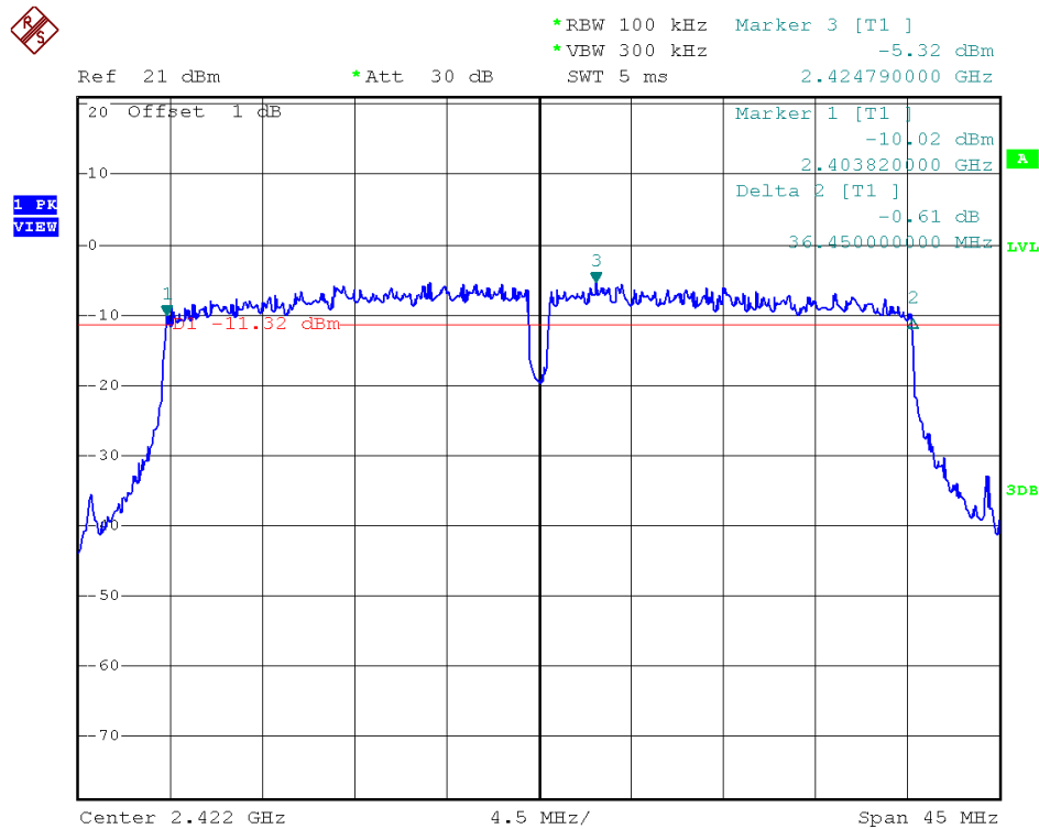
Antenna A - Channel 3/ 6 dB Bandwidth
