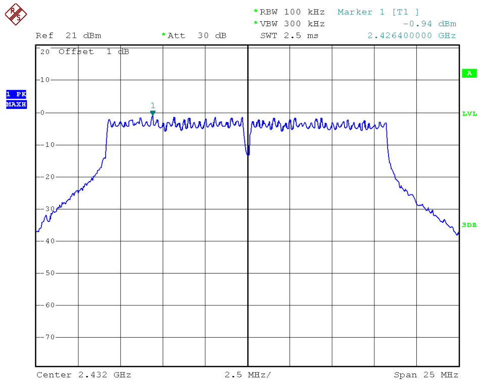
(Plot 2.5 E1: Channel = 5 @ 802.11g)
