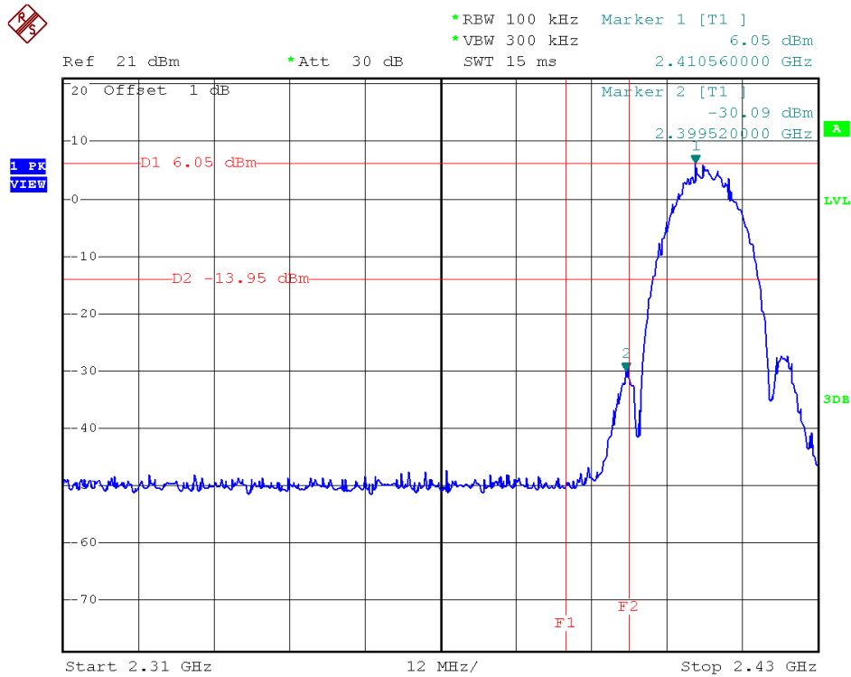
Antenna B Channel = 1 @ 802.11b
