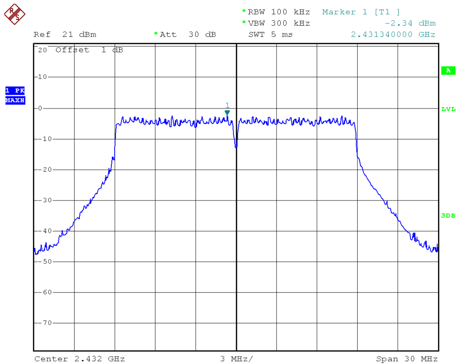
(Plot 2.5 H2: Channel = 5 @ 802.11n-20)
