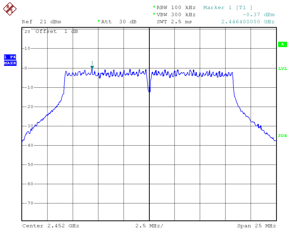
(Plot 2.5 F1: Channel = 9 @ 802.11g)
