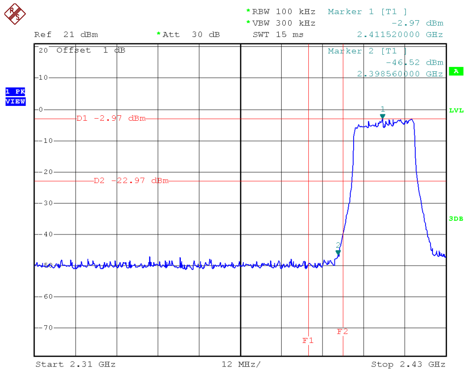
Antenna B Channel = 1 @ 802.11n-20
