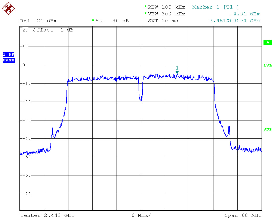
(Plot 2.5 L2: Channel = 7 @ 802.11n-40)
