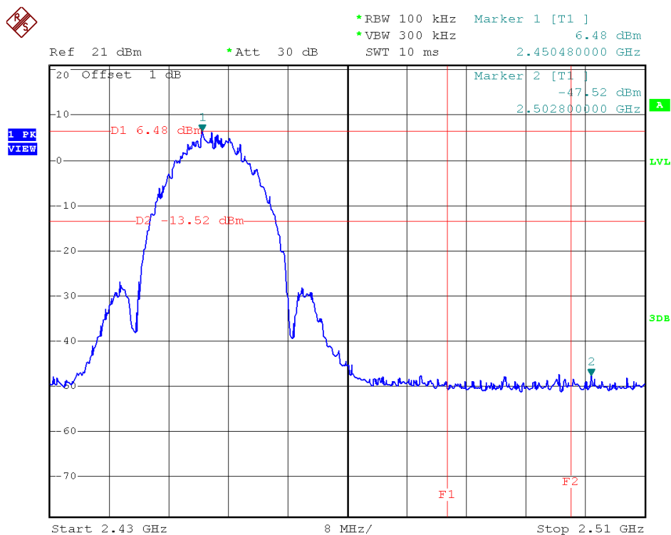
Antenna B Channel = 9 @ 802.11b
