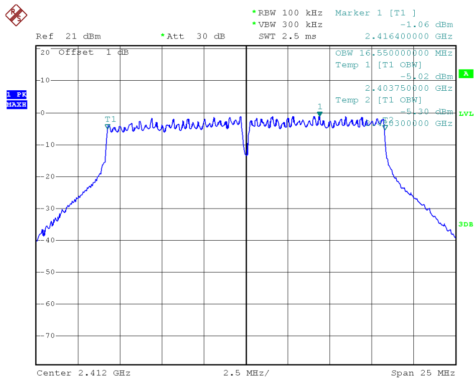
Antenna B - Channel 1/ 99% Occupied Bandwidth
