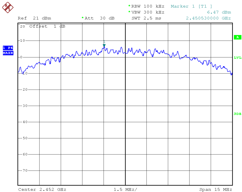
(Plot 2.5 C2: Channel = 9 @ 802.11b)
