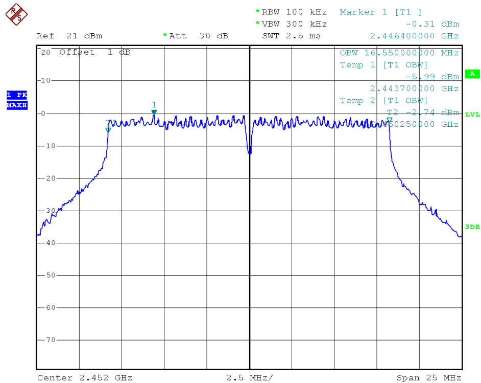
Antenna A - Channel 9 / 99% Occupied Bandwidth
