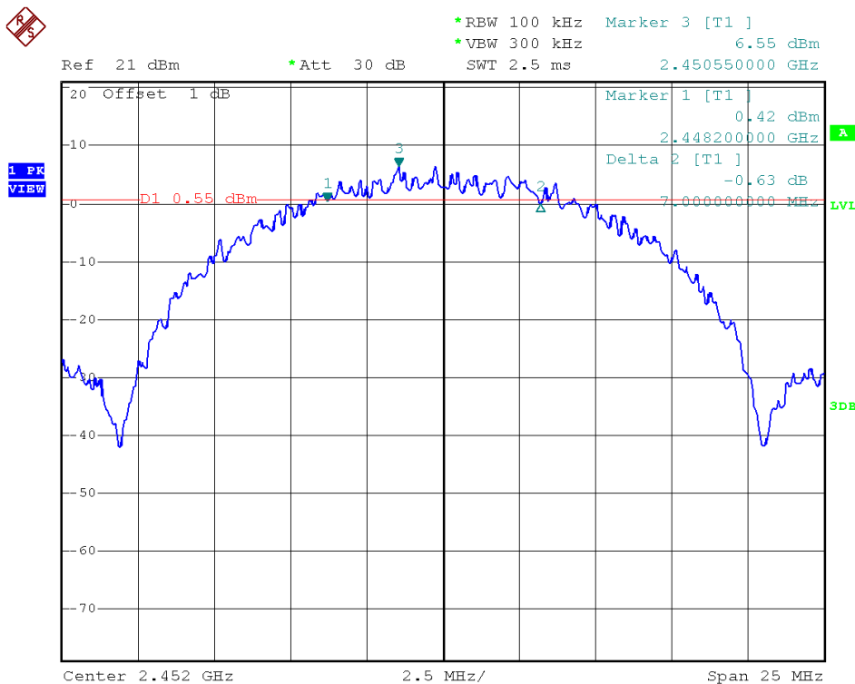
Antenna B - Channel 9 / 6 dB Bandwidth
