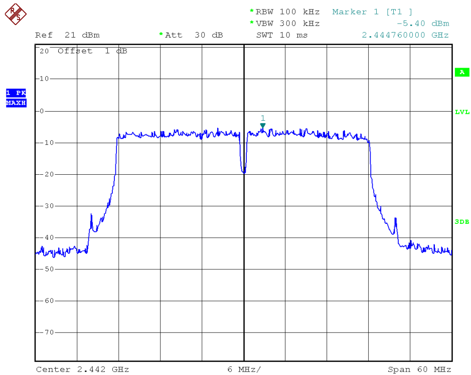
(Plot 2.5 L1: Channel = 7 @ 802.11n-40)
