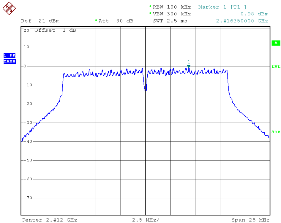
(Plot 2.5 D2: Channel = 1 @ 802.11g)
