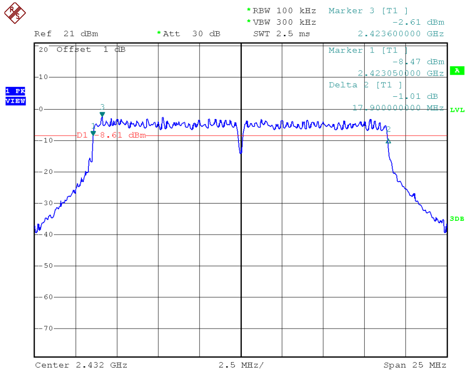
Antenna A - Channel 5/ 6 dB Bandwidth
