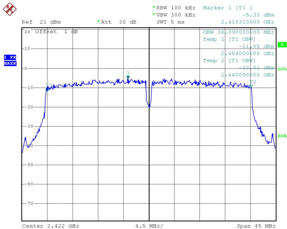
Antenna A - Channel 3/ 99% Occupied Bandwidth
