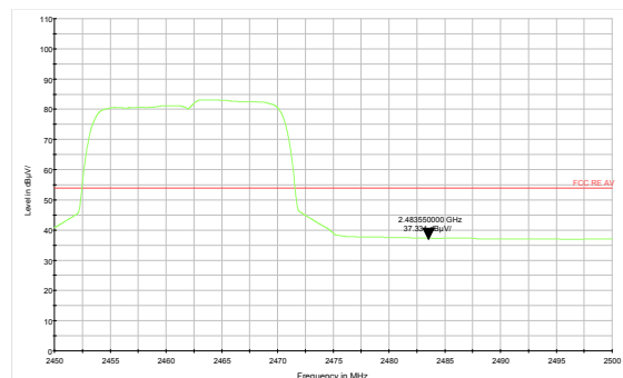
802.11g-Channel 11 Average
