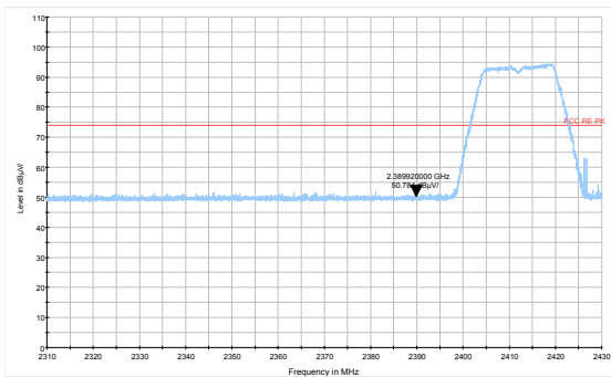
802.11g-Channel 1 Peak
