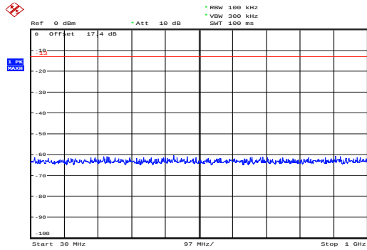
NB-IOT Band 4 CH-Low 30MHz~1GHz
