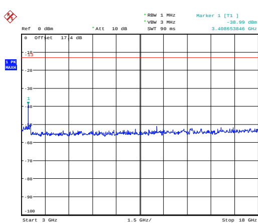
NB-IOT Band 4 CH-Low 3GHz~18GHz
