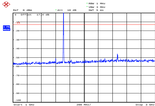
NB-IOT Band 4 CH-Low 1GHz~3GHz
