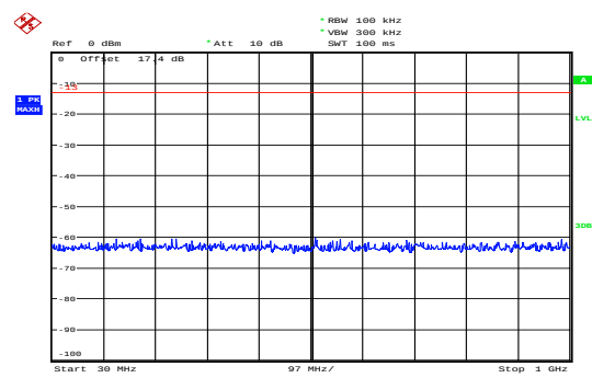
NB-IOT Band 4 CH-Middle 30MHz~1GHz
