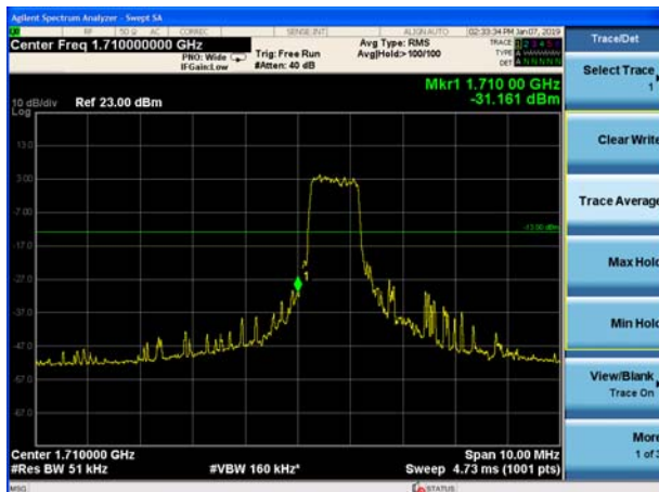
eMTC Band 4 16QAM 5MHz CH-Low, 100%RB
