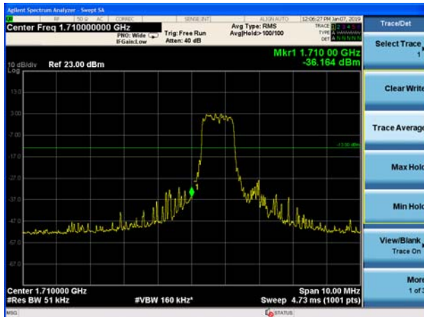
eMTC Band 4 16QAM 5MHz CH-Low, 1 RB
