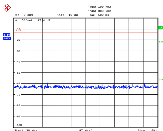
eMTC Band 4 5MHz CH-Middle 30MHz~1GHz
