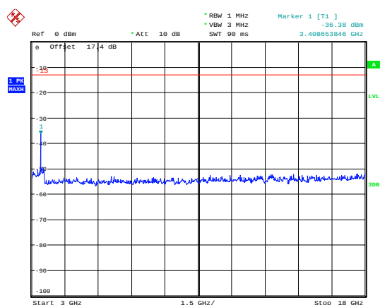
eMTC Band 4 5MHz CH-Low 3GHz~18GHz
