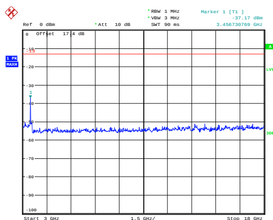
eMTC Band 4 5MHz CH-Middle 3GHz~18GHz
