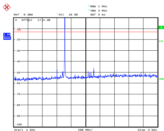
eMTC Band 4 5MHz CH-Low 1GHz~3GHz
