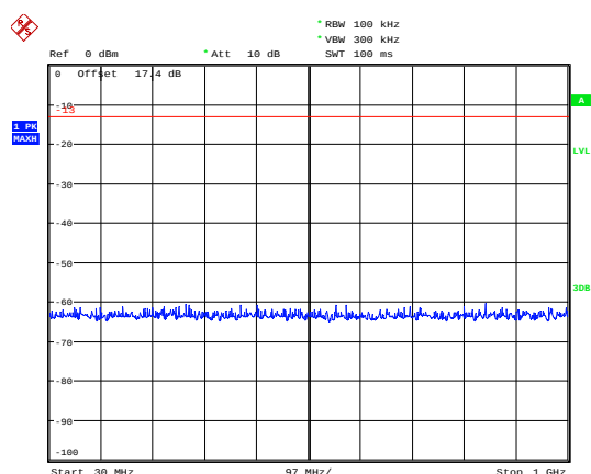
eMTC Band 4 5MHz CH-Low 30MHz~1GHz
