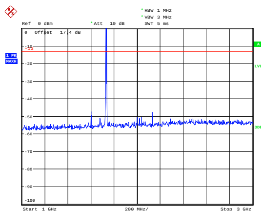
eMTC Band 4 5MHz CH-Middle 1GHz~3GHz
