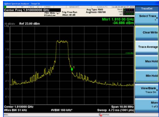
eMTC Band 2 5MHz 16QAM 1RB CH-High
