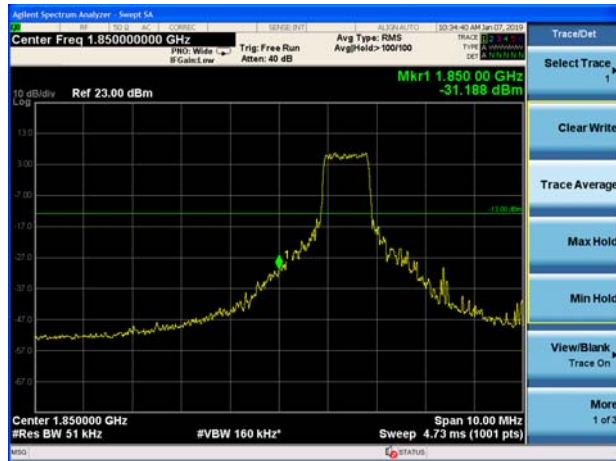
eMTC Band 2 20MHz 16QAM 1RB CH-Low
