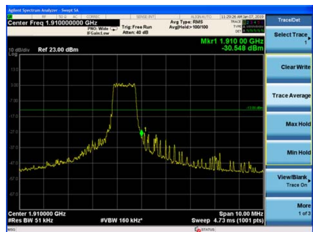
eMTC Band 2 5MHz 16QAM 100%RB CH-High
