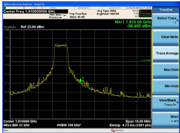
eMTC Band 2 20MHz 16QAM 1RB CH-High
