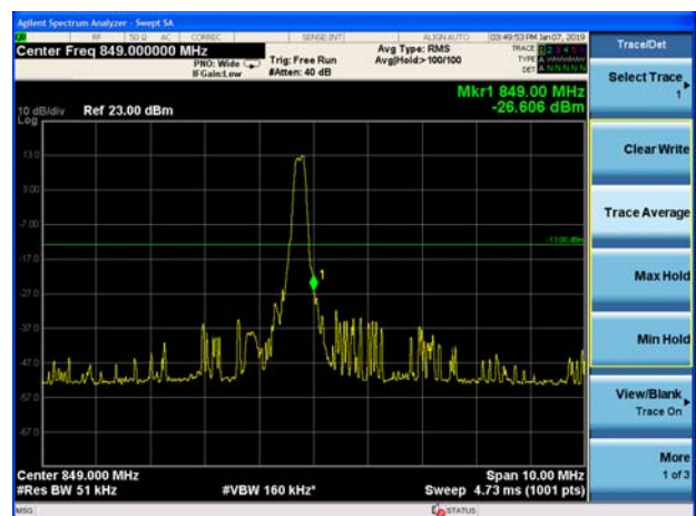
eMTC Band 5 16QAM 1.4MHz CH-High 1RB
