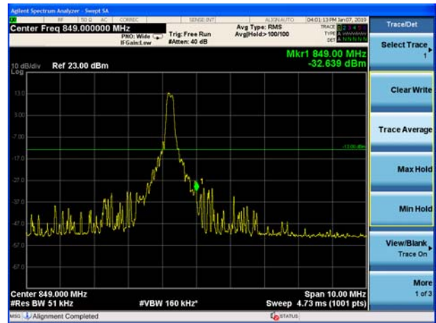
eMTC Band 5 QPSK 10MHz CH-High 100%RB
