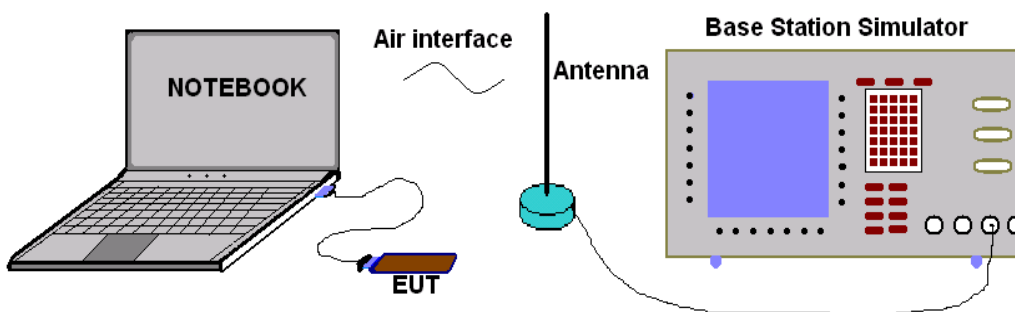
Connection Diagram (Mode 3~Mode 4)
