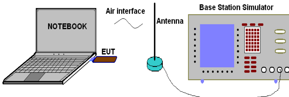
Connection Diagram (Mode 3~Mode 4)
