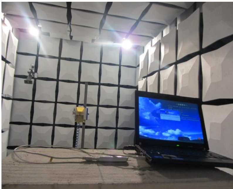
Radiated Spurious Emission (below 3GHz)
