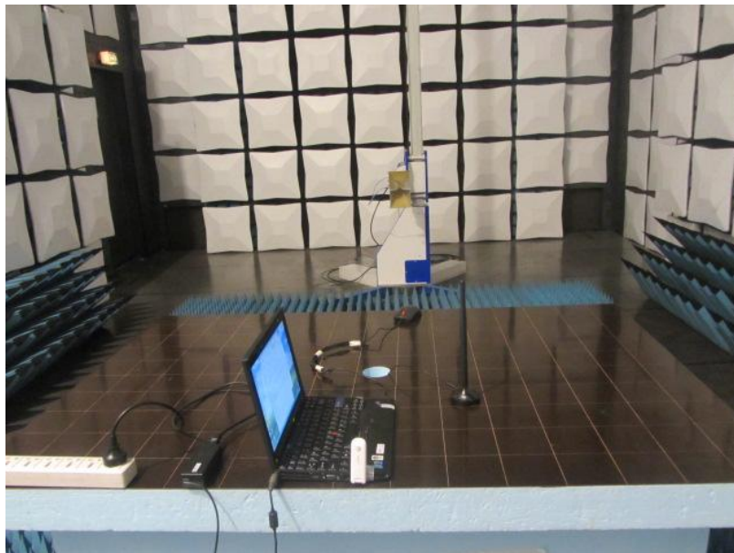
Radiated Emission (1GHz to18GHz)
