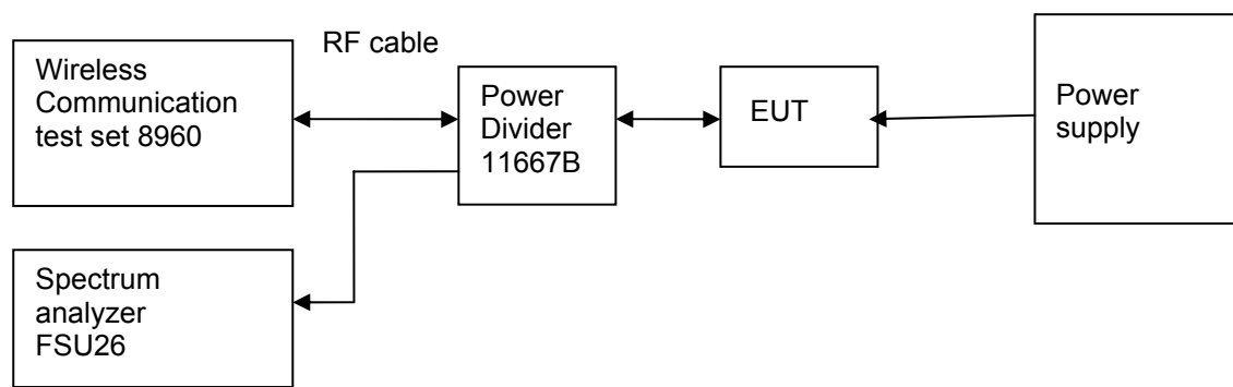
Figure 6. Test Set-up
