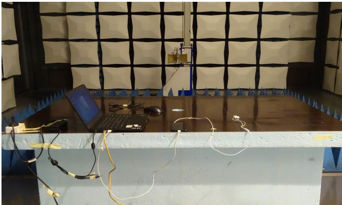
Radiated Disturbance Emissions (1GHz to 18GHz)
