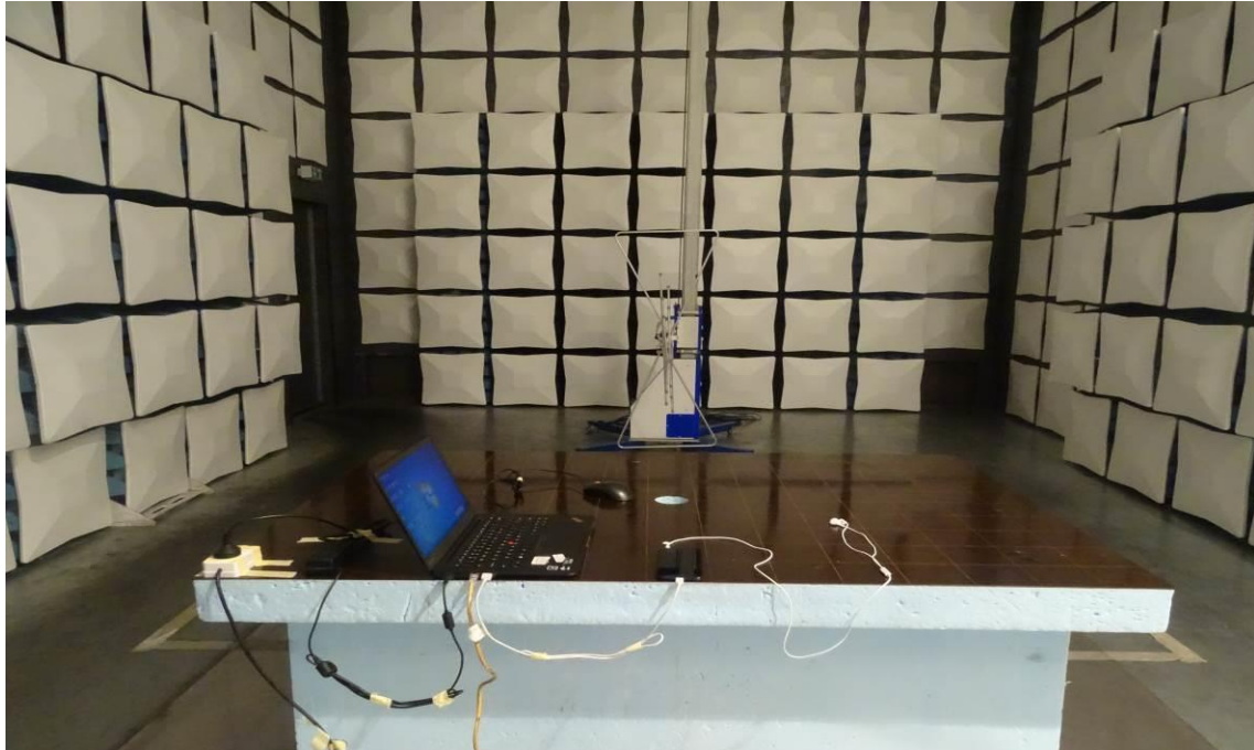
Radiated Disturbance Emissions (below 1GHz)
