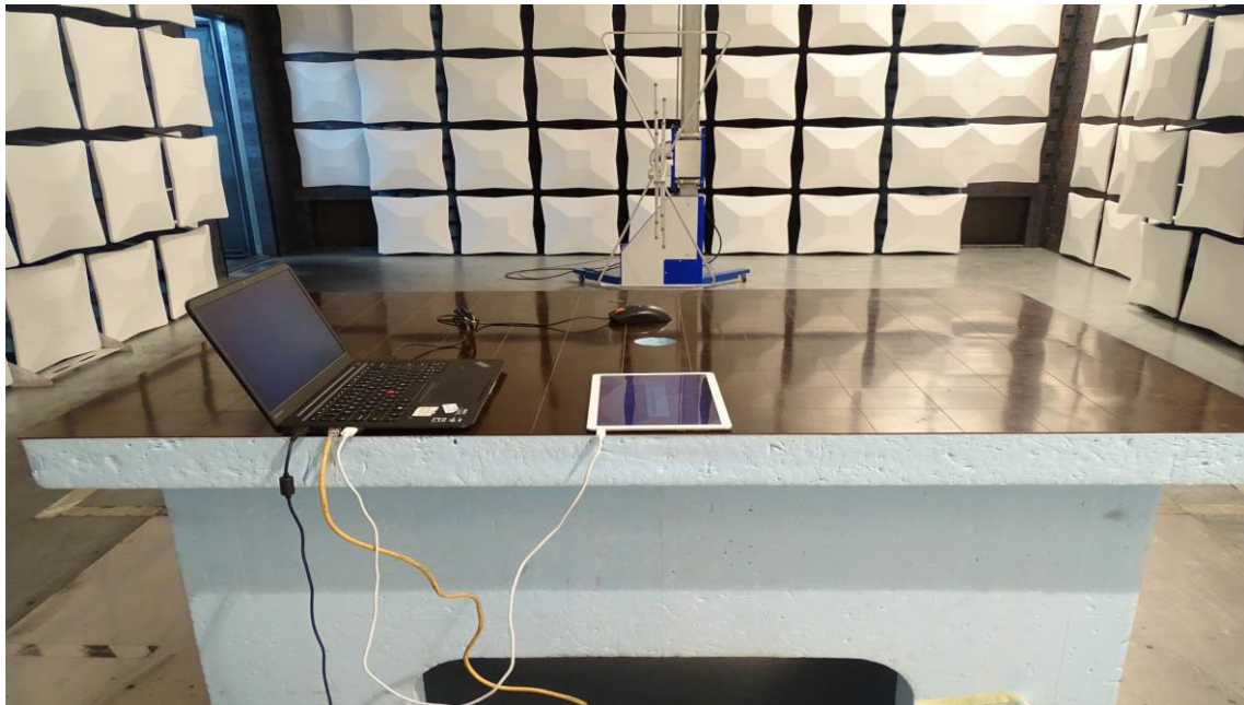
Radiated Disturbance Emissions (below 1GHz)
