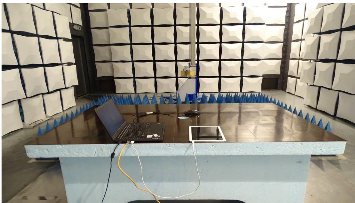
Radiated Disturbance Emissions (1GHz to 18GHz)
