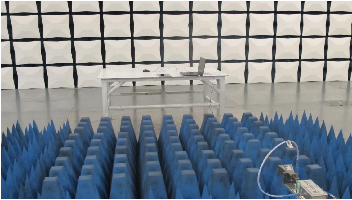
Radiated Disturbance Emissions (18GHz to 26.5GHz)
