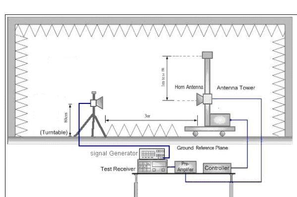
Figure 3. above 1GHz
