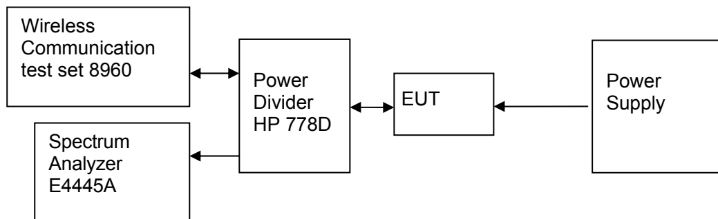
Figure 4. Test Set-up
