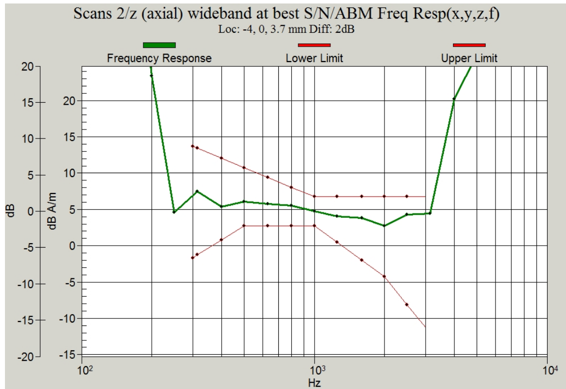
Figure C.5 Frequency Response of CDMA 1880_Channel 600
