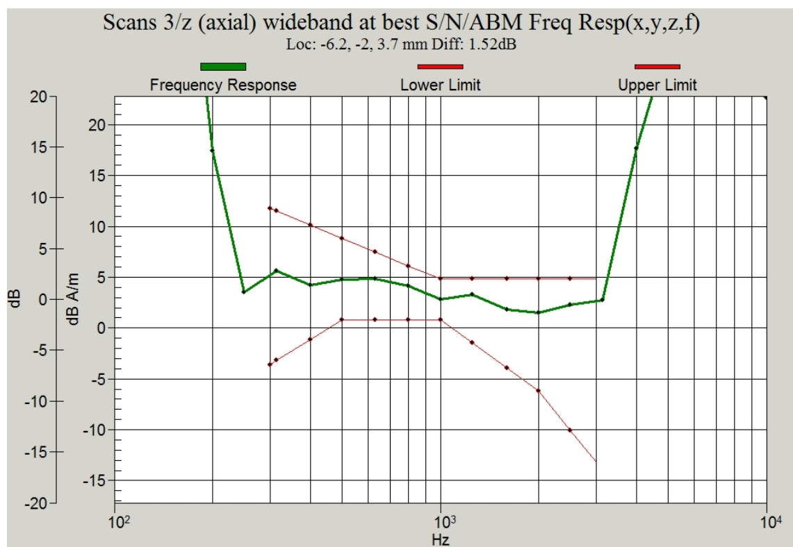
Figure C.6 Frequency Response of CDMA 1880_Channel 25
