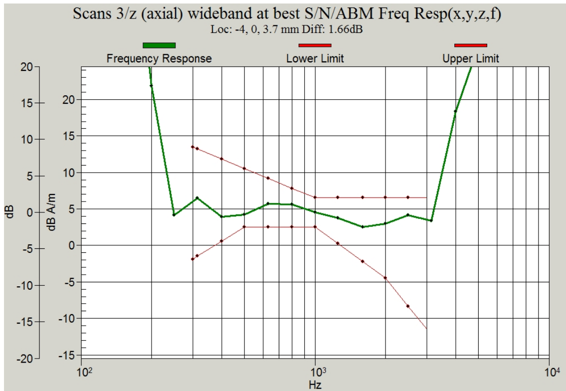
Figure C.9 Frequency Response of CDMA 1700_Channel 25
