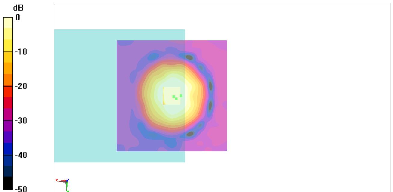
Fig B.21 T-Coil CDMA 1700_Channel 875
