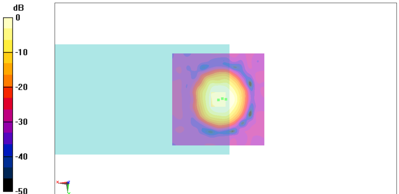
Fig B.15 T-Coil CDMA 1880_Channel 600
