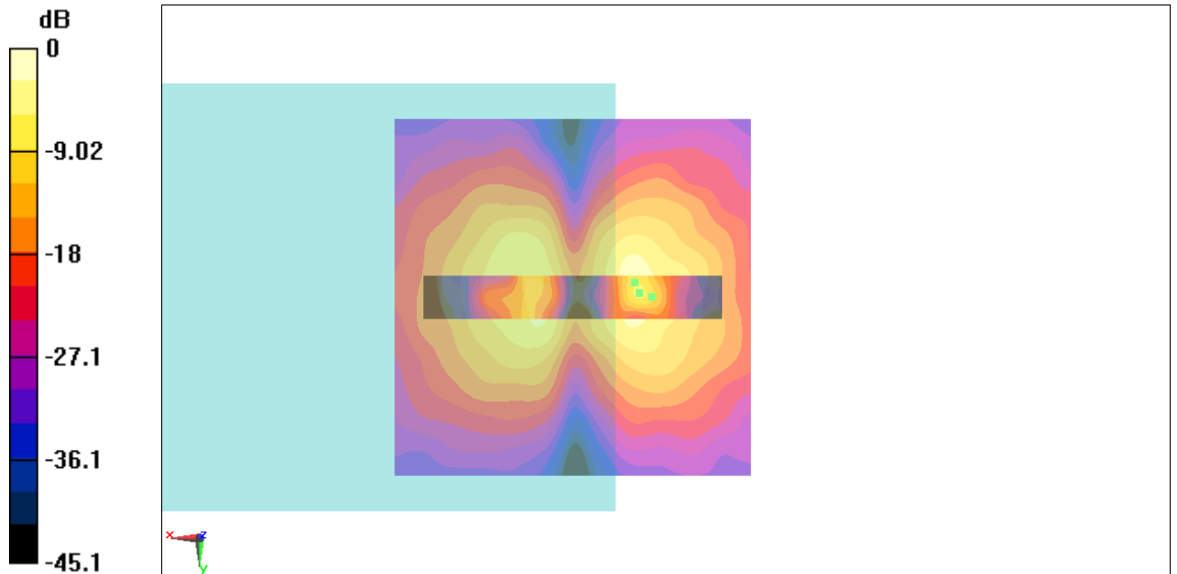
Fig B.19 T-Coil CDMA 1700_Channel 875
