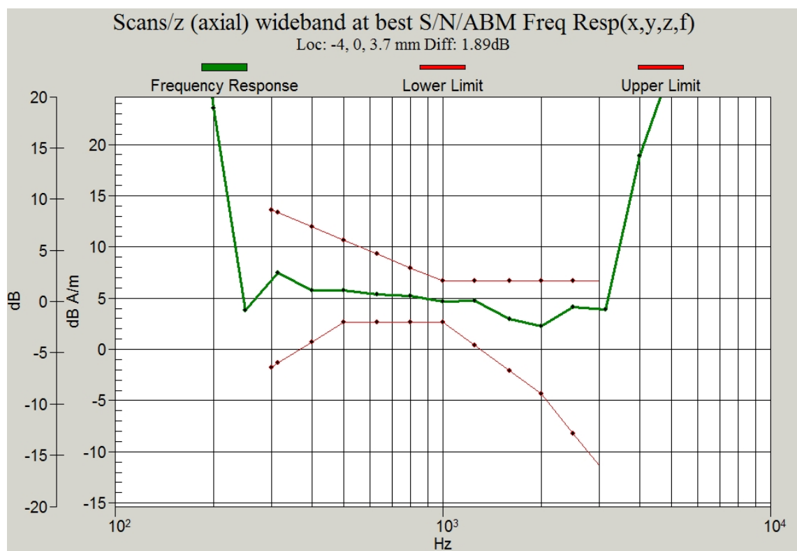
Figure C.4 Frequency Response of CDMA 1880_Channel 1175
