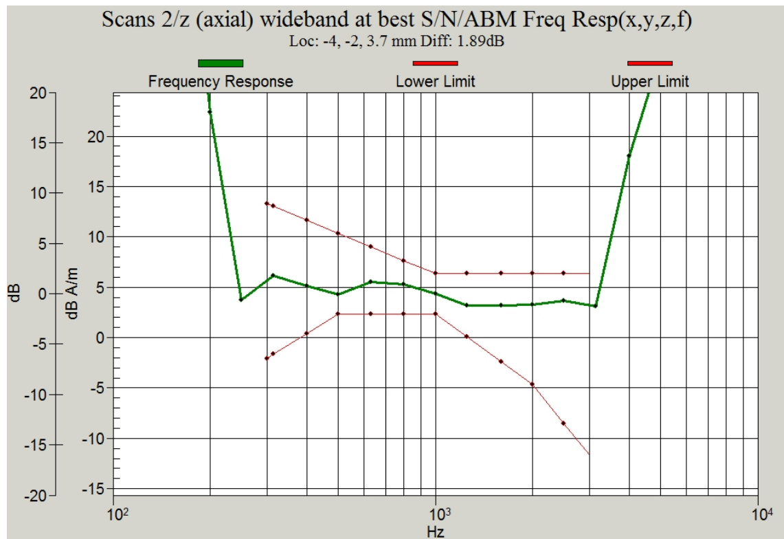
Figure C.2 Frequency Response of CDMA 835_Channel 384
