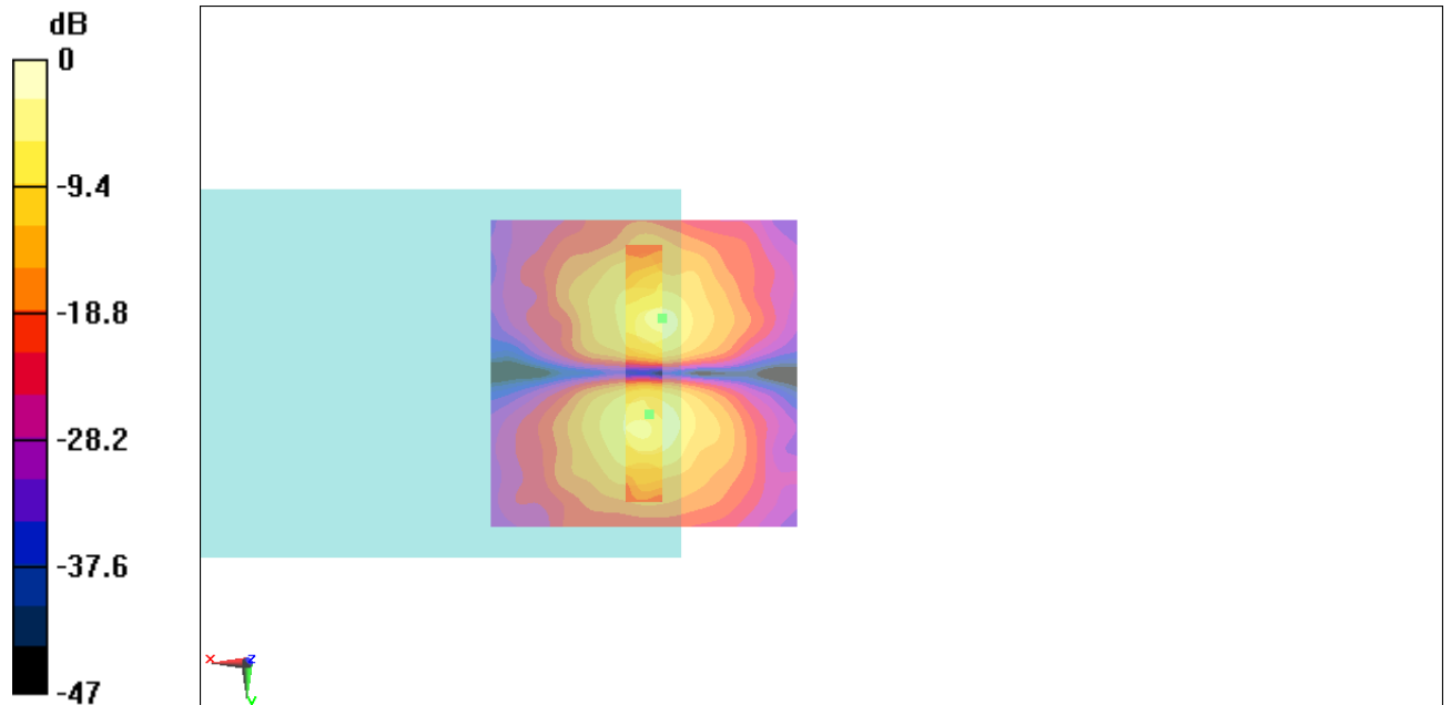
Fig B.8 T-Coil CDMA 835_Channel 1013
