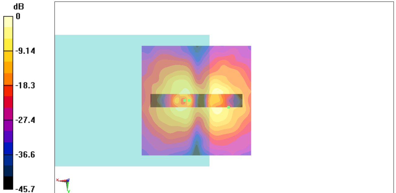
Fig B.10 T-Coil CDMA 1880_Channel 1175
