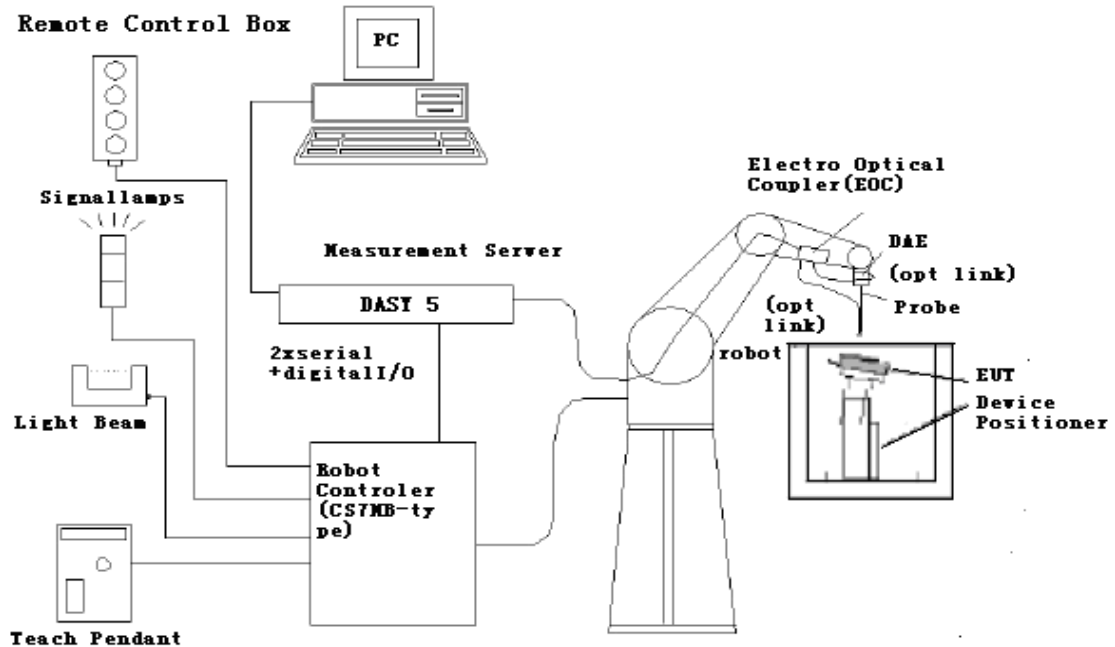
Figure 6.1 HAC Test Measurement Set-up
