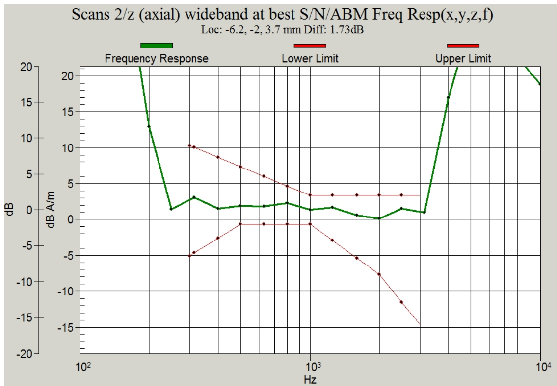
Figure C.8 Frequency Response of CDMA 1700_Channel 450
