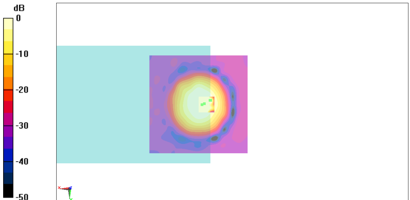
Fig B.24 T-Coil CDMA 1700_Channel 450
