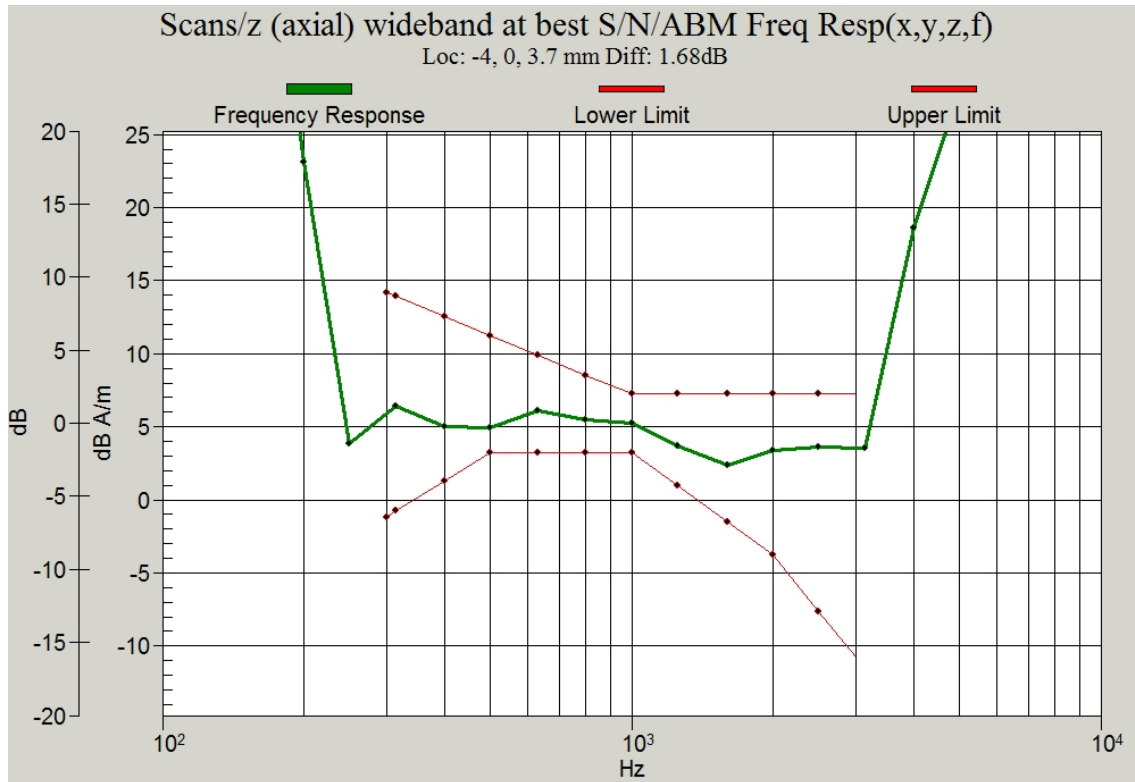
Figure C.7 Frequency Response of CDMA 1700_Channel 875
