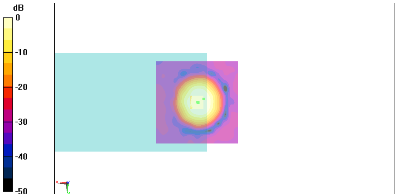
Fig B.9 T-Coil CDMA 835_Channel 1013
