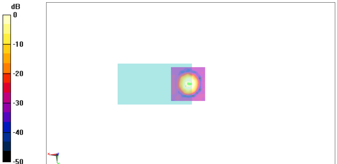
Fig B.12 T-Coil CDMA 1880_Channel 1175
