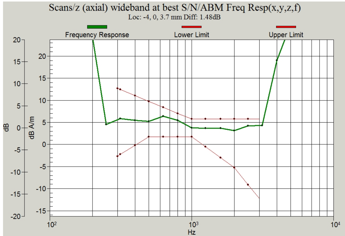
Figure C.1 Frequency Response of CDMA 835_Channel 777
