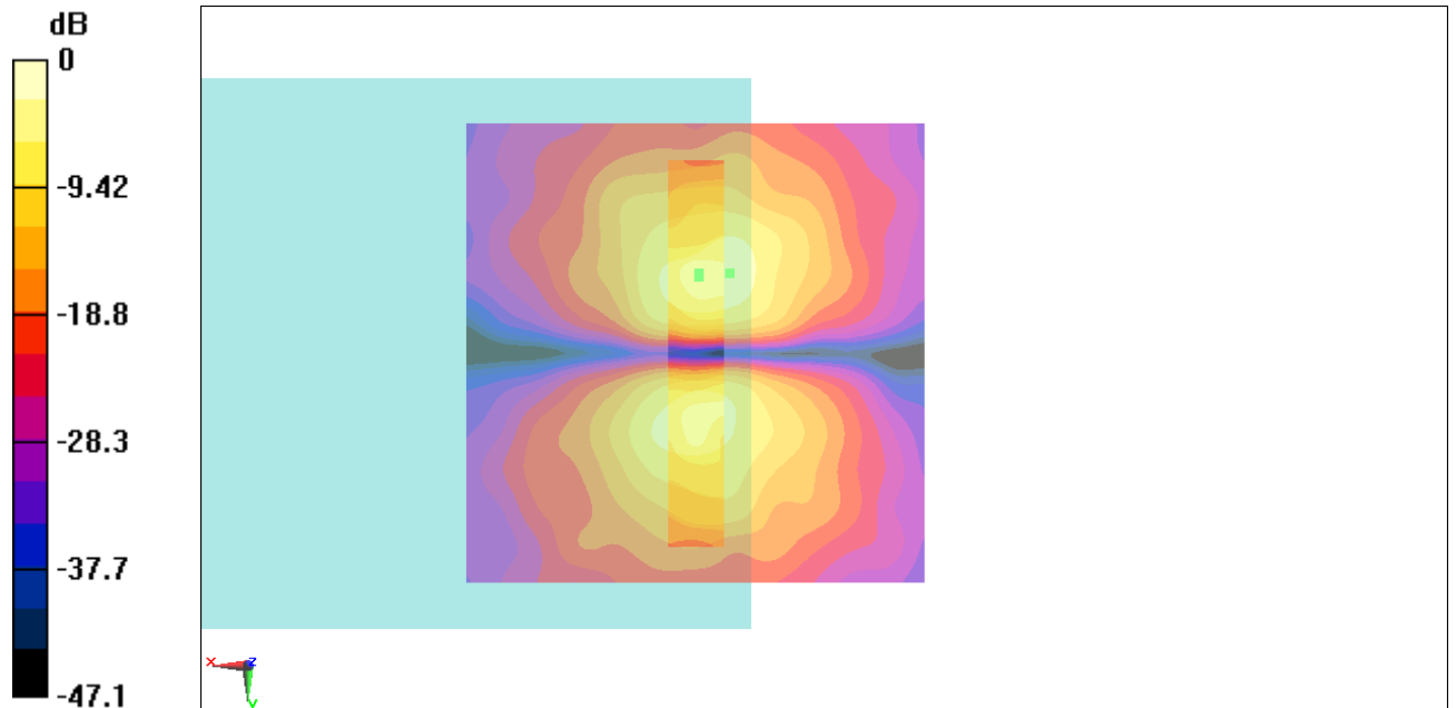
Fig B.14 T-Coil CDMA 1880_Channel 600
