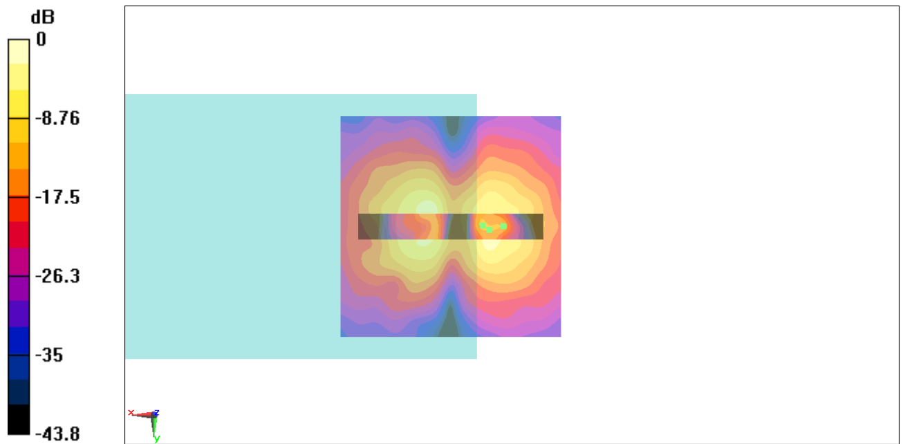
Fig B.1 T-Coil CDMA 835_Channel 777
