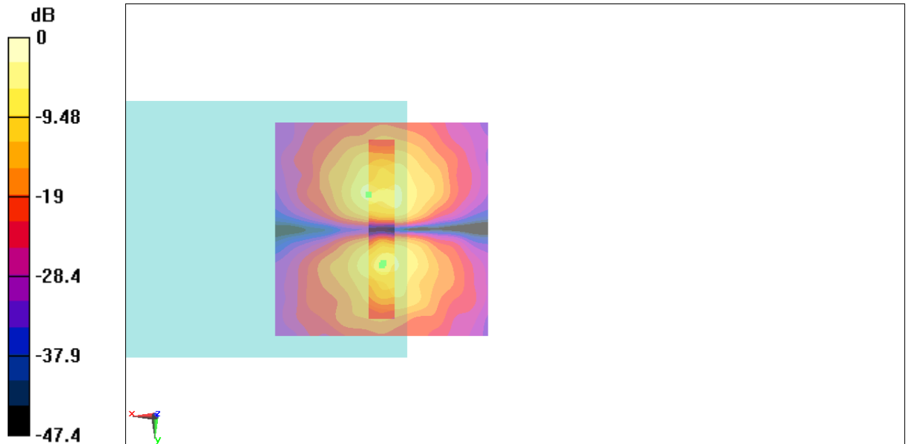
Fig B.20 T-Coil CDMA 1700_Channel 875
