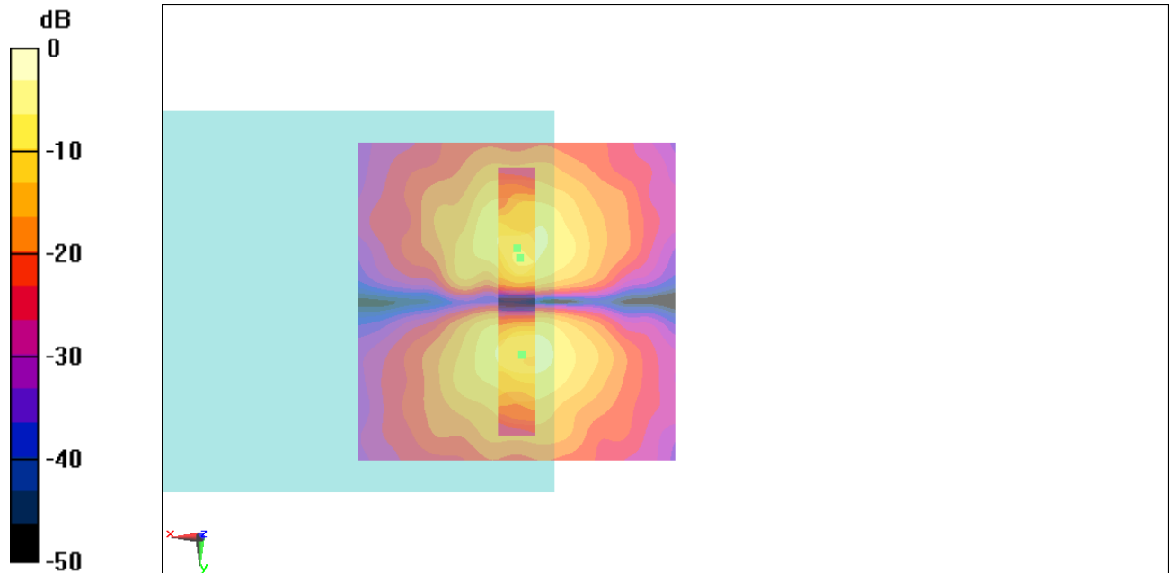
Fig B.26 T-Coil CDMA 1700_Channel 25
