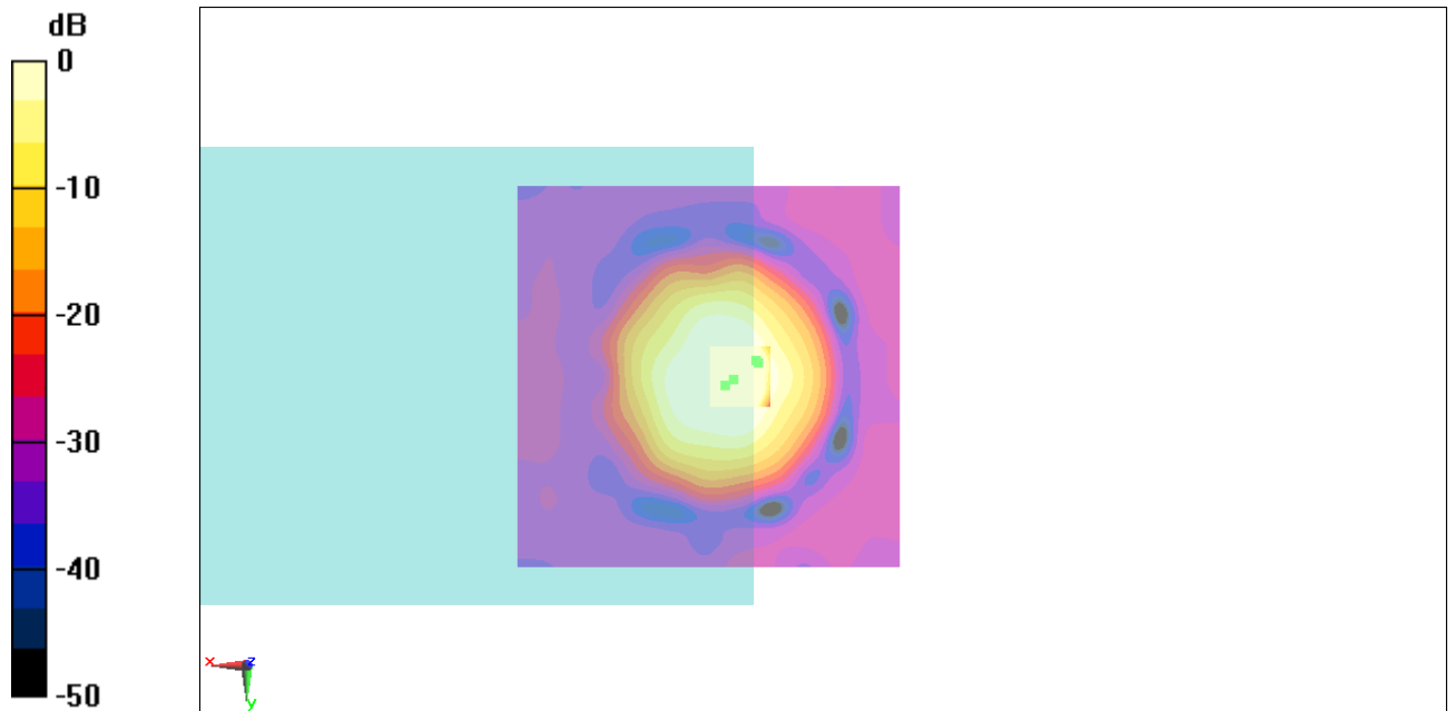
Fig B.18 T-Coil CDMA 1880_Channel 25
