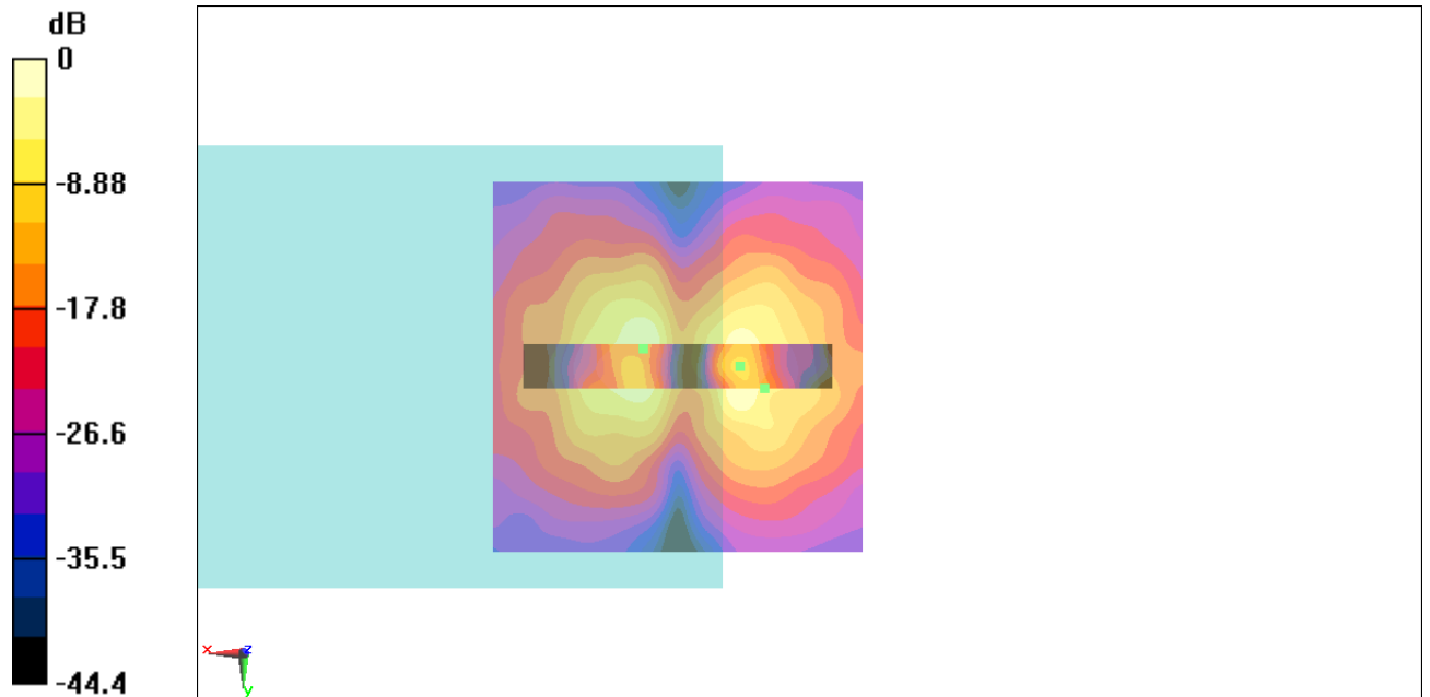
Fig B.7 T-Coil CDMA 835_Channel 1013
