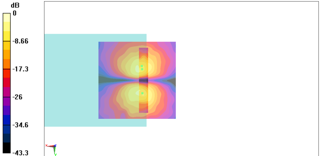
Fig B.17 T-Coil CDMA 1880_Channel 25
