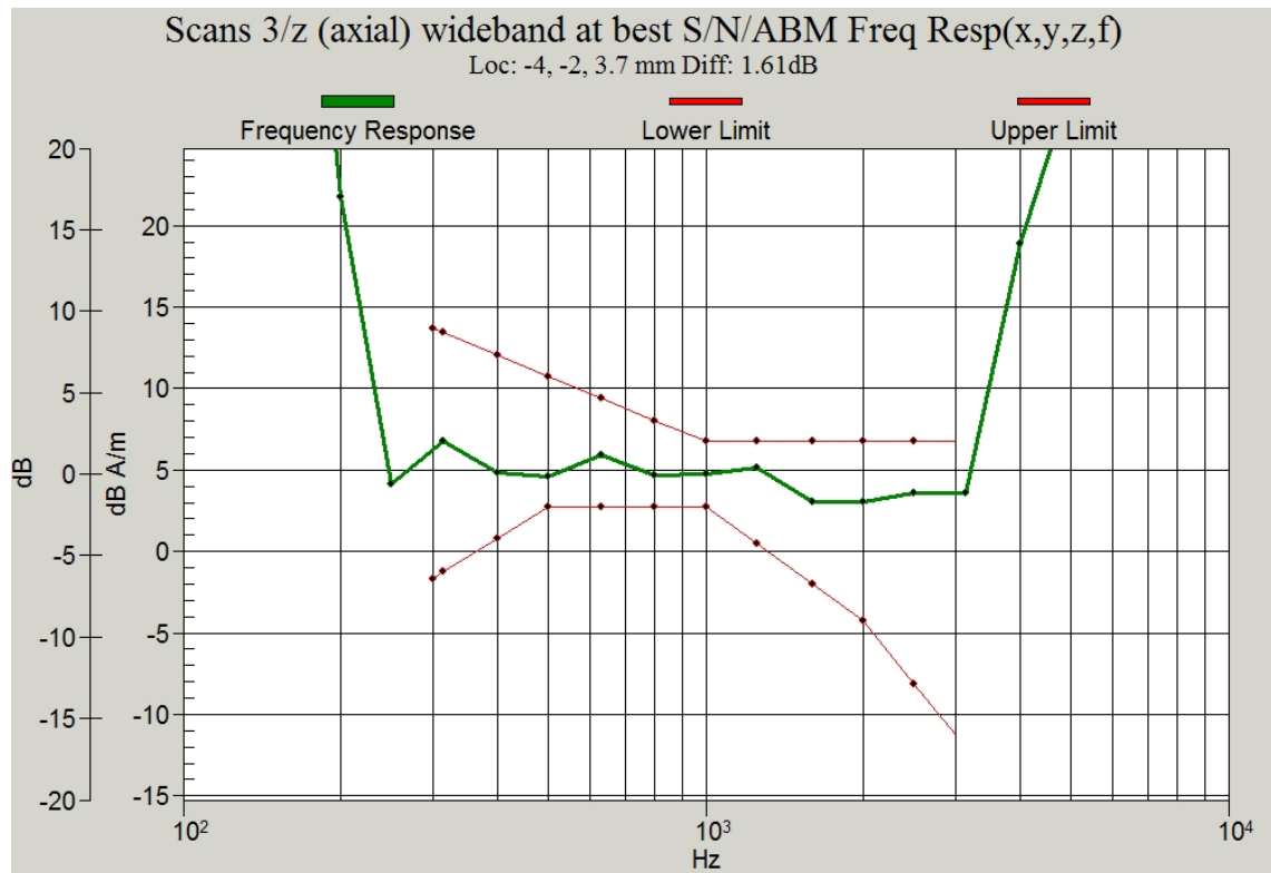
Figure C.3 Frequency Response of CDMA 835_Channel 1013
