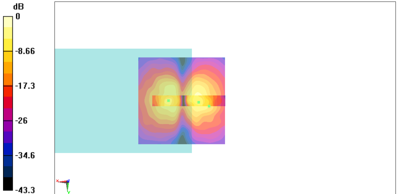
Fig B.22 T-Coil CDMA 1700_Channel 450
