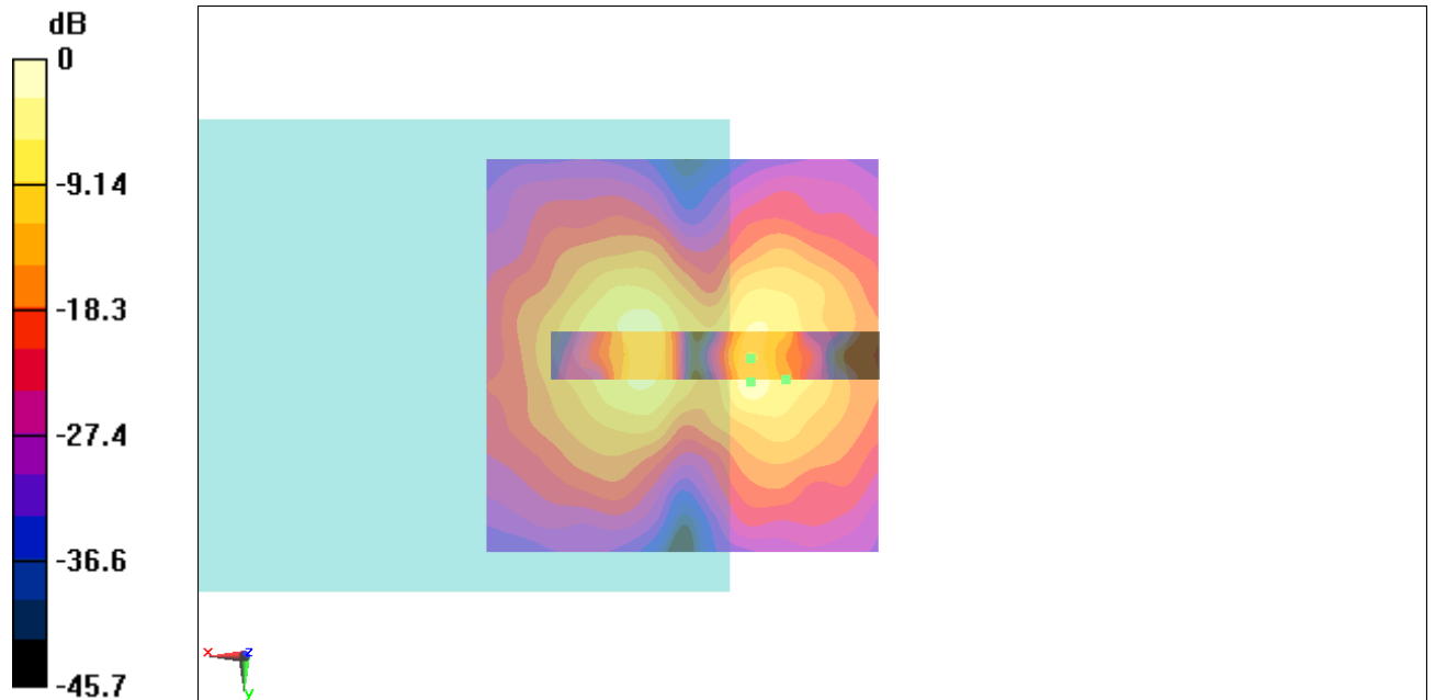
Fig B.16 T-Coil CDMA 1880_Channel 25
