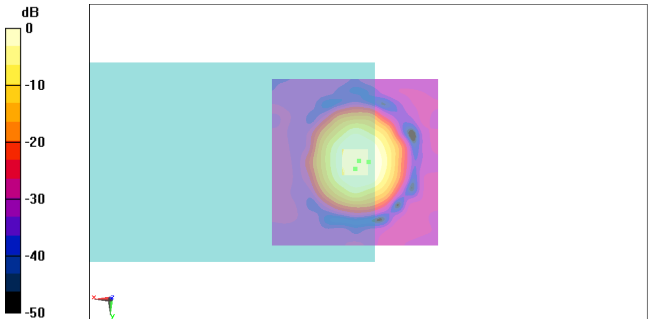
Fig B.3 T-Coil CDMA 835_Channel 777
