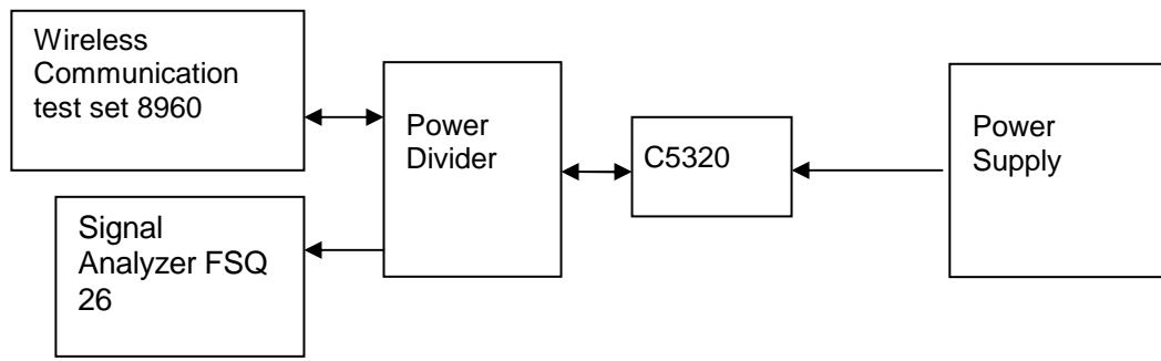
Figure 3. Test Set-up
