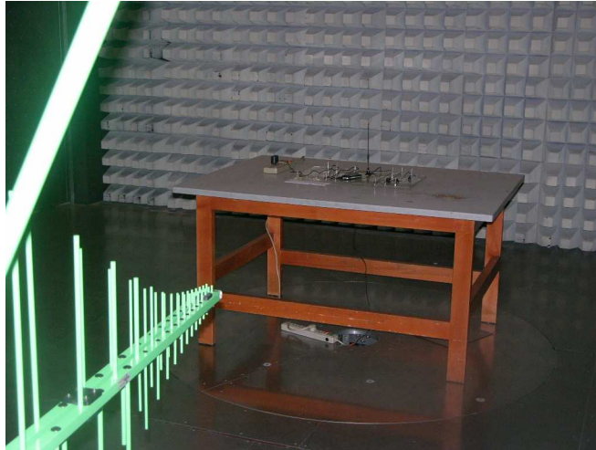
Radiated Disturbance
