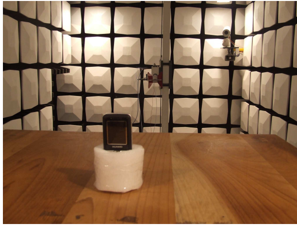
Radiated Spurious Emission (above 2GHz)
