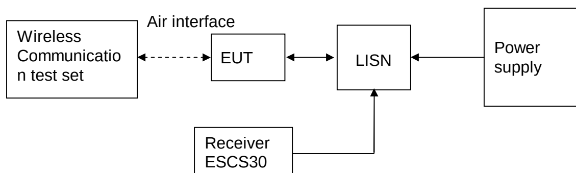
Figure 3. Test Set-up
