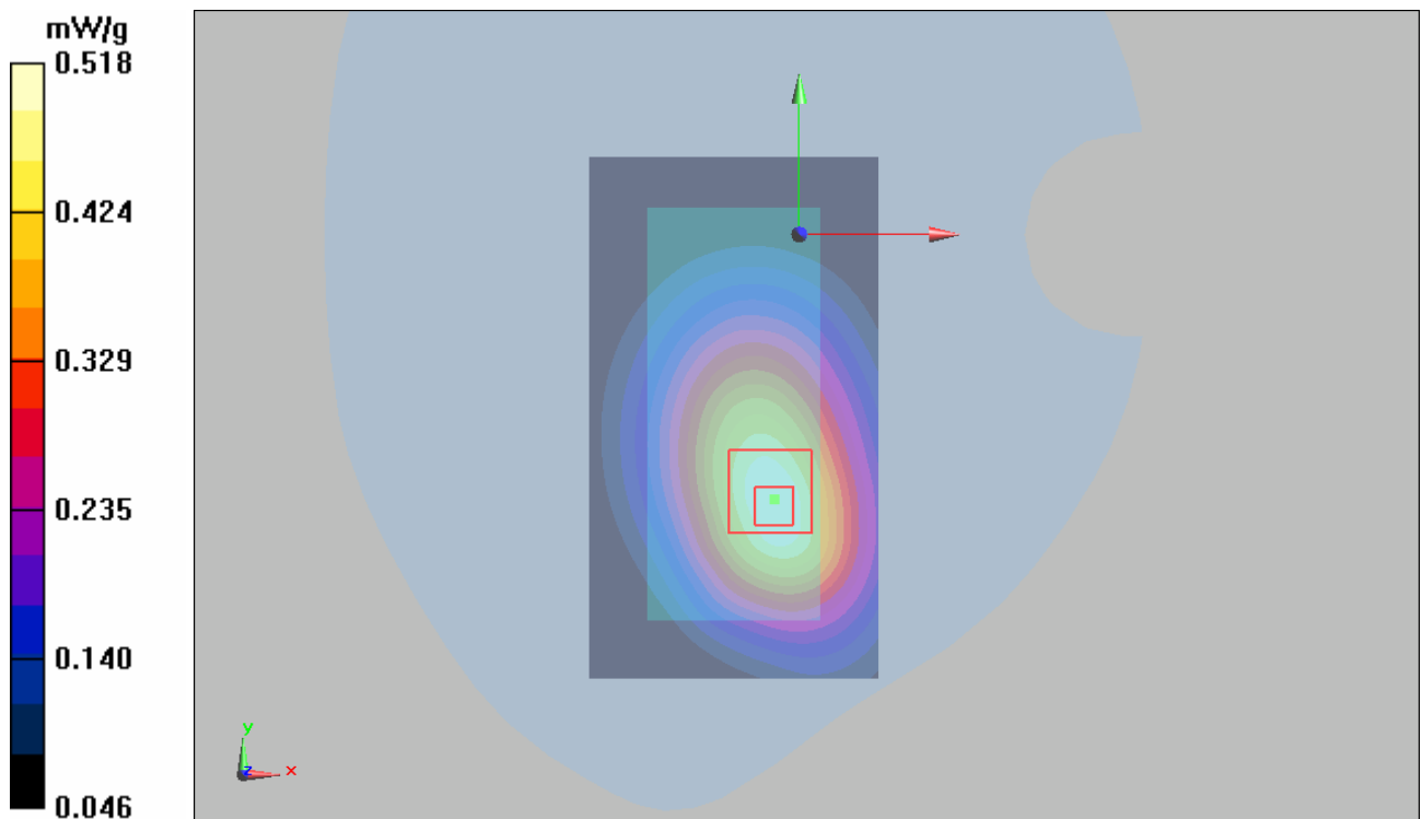
Figure 17 Body, Towards Ground, CDMA Cellular Channel 777
