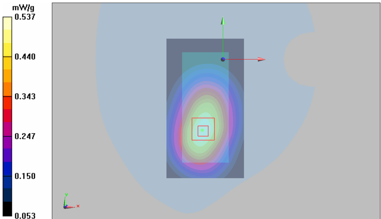
Figure 20 Body, Towards Phantom, CDMA Cellular Channel 384
