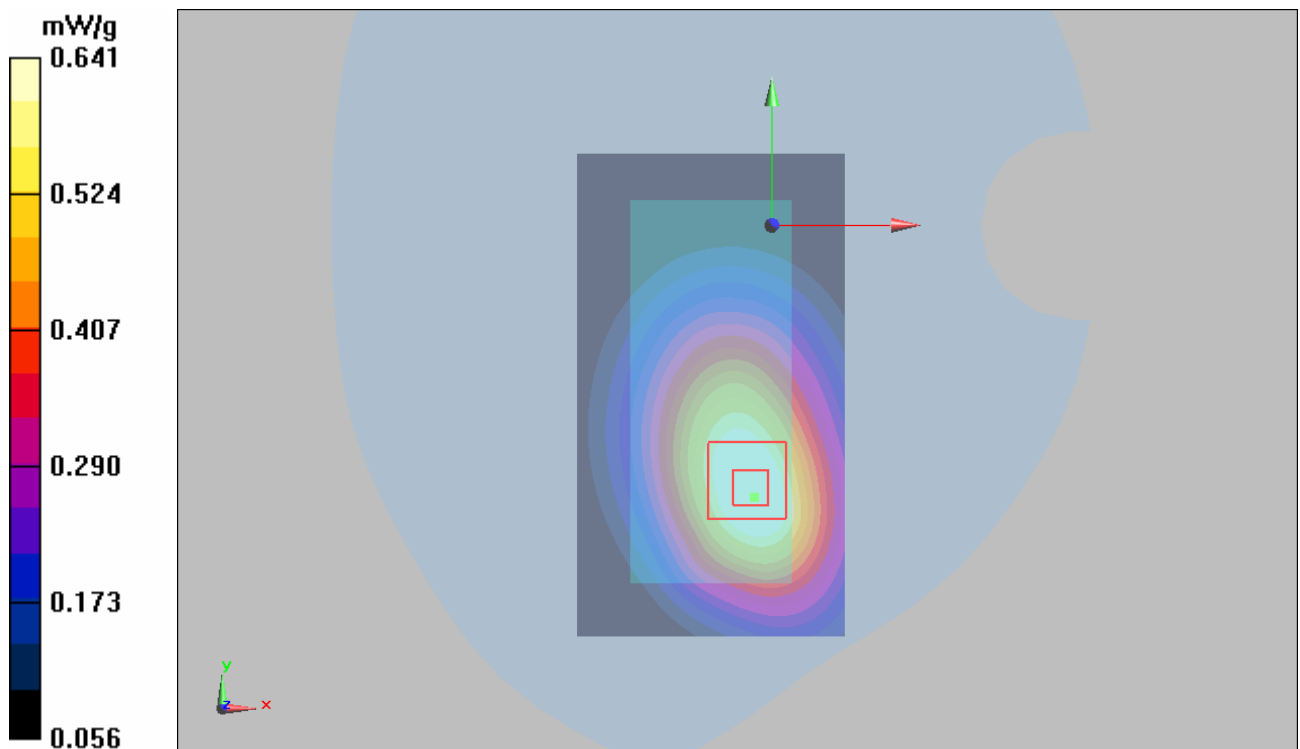
Figure 21 Body with Earphone, Towards Ground, CDMA Cellular Channel 1013
