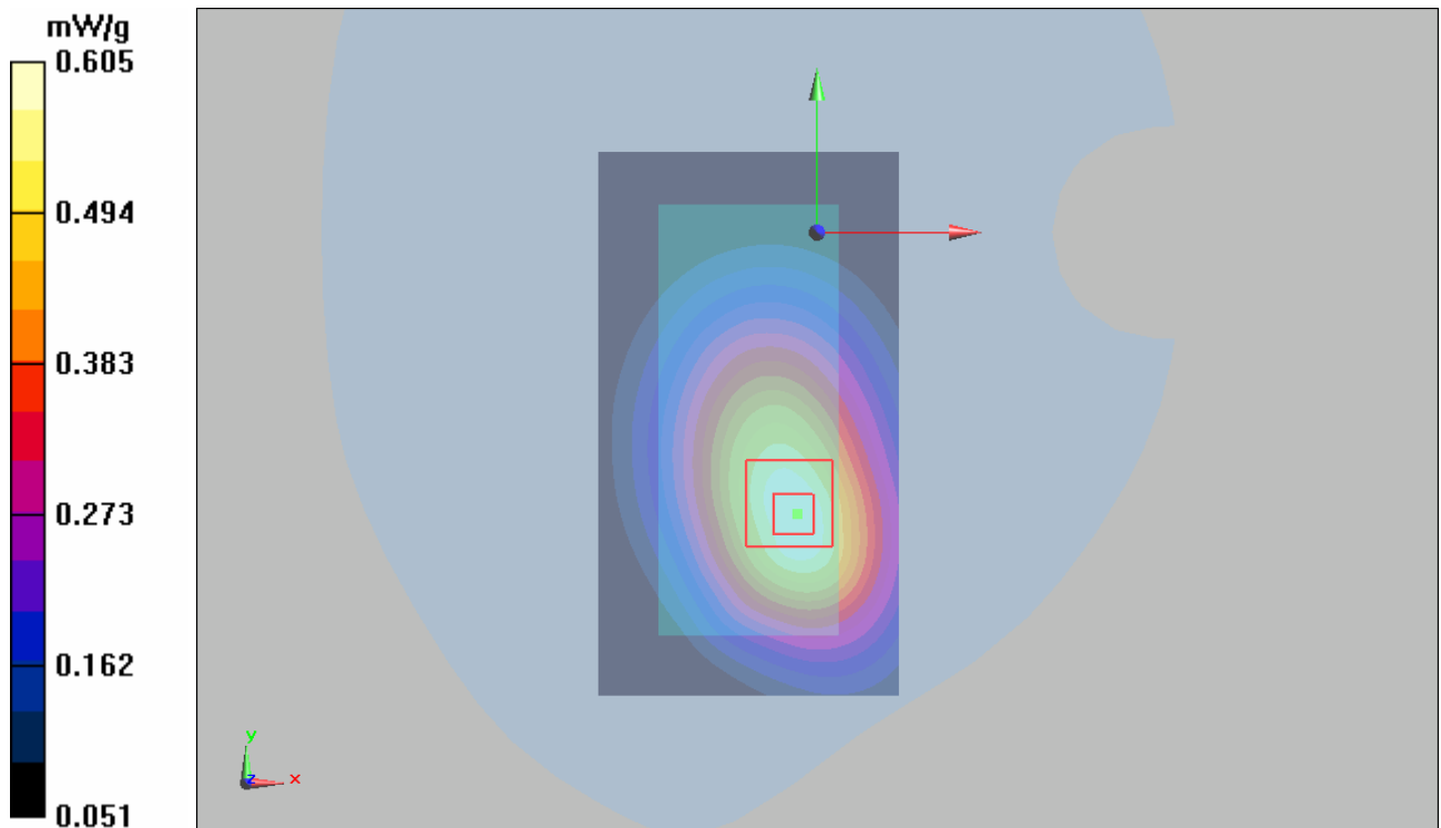
Figure 18 Body, Towards Ground, CDMA Cellular Channel 384
