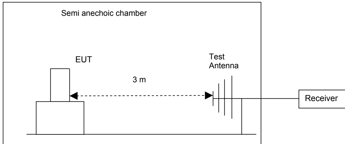
Figure 12. Test set up
