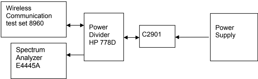
Figure 4. Test Set-up
