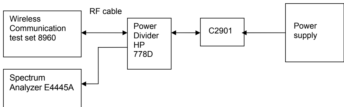
Figure 5. Test Set-up
