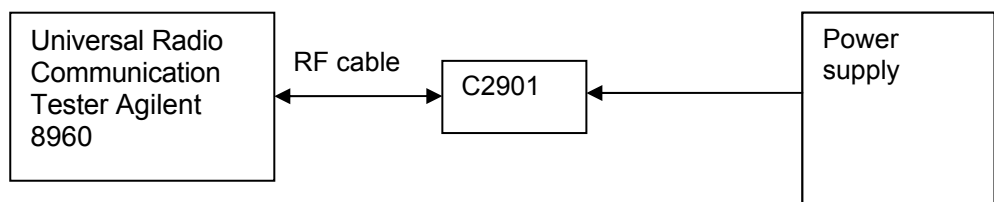
Figure 2. Test Set-up
