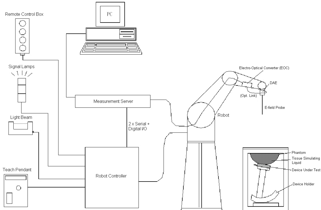
Fig 5.1 SPEAG DASY4 or DASY5 System Configurations
