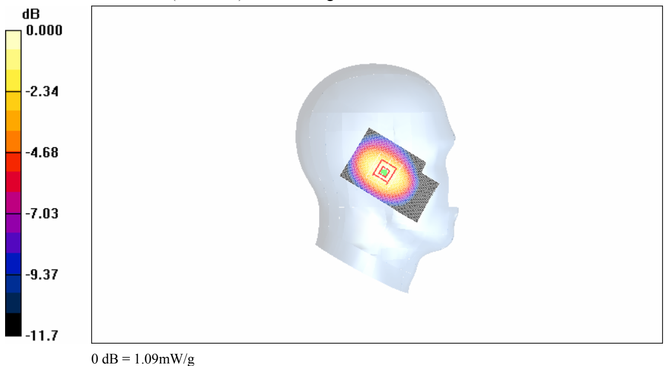
Fig. 1 Left Hand Touch Cheek CDMA 835MHz CH777
