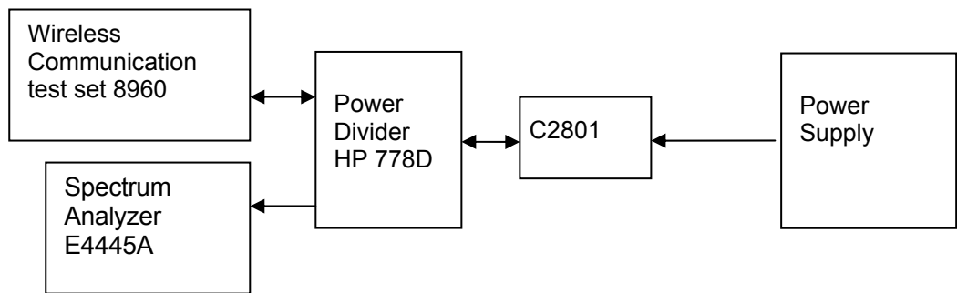
Figure 4. Test Set-up
