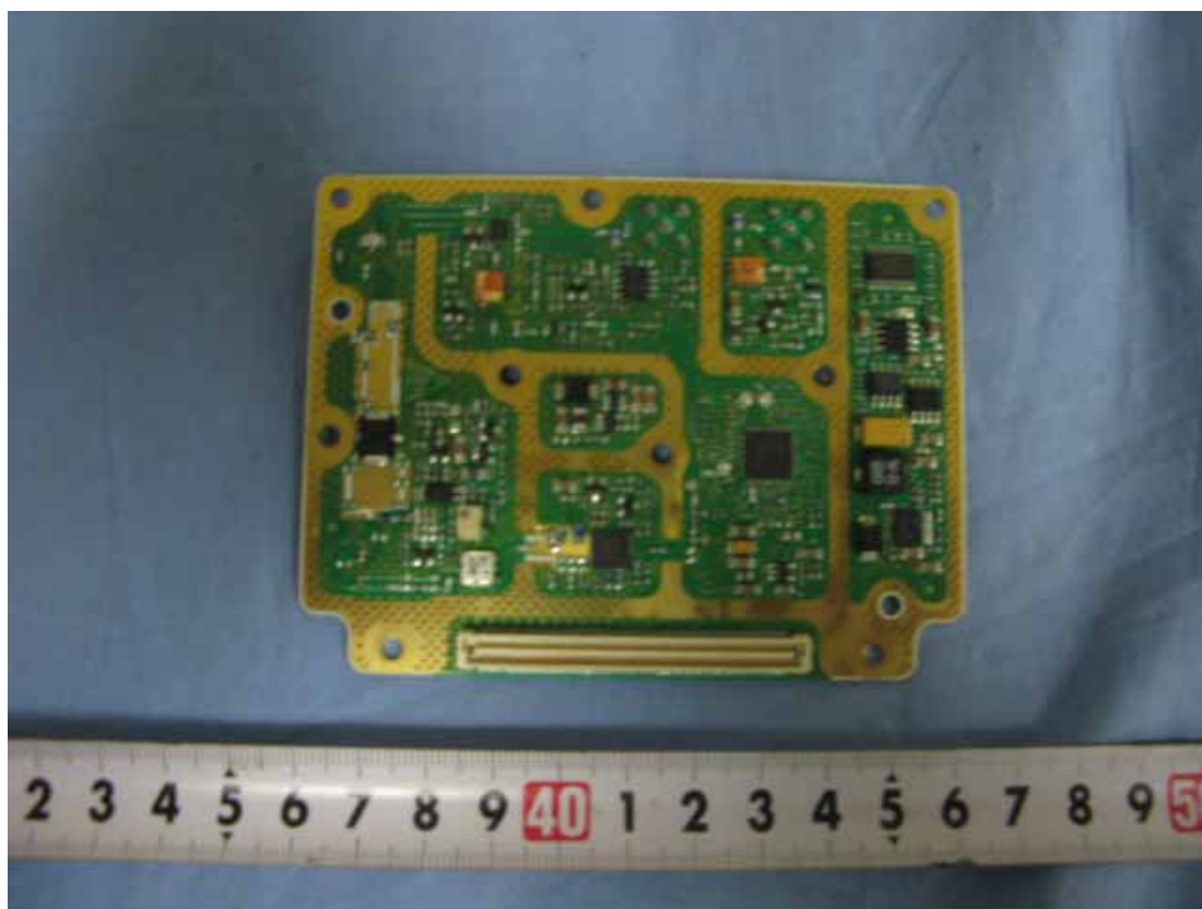
03 View of RF board components side
