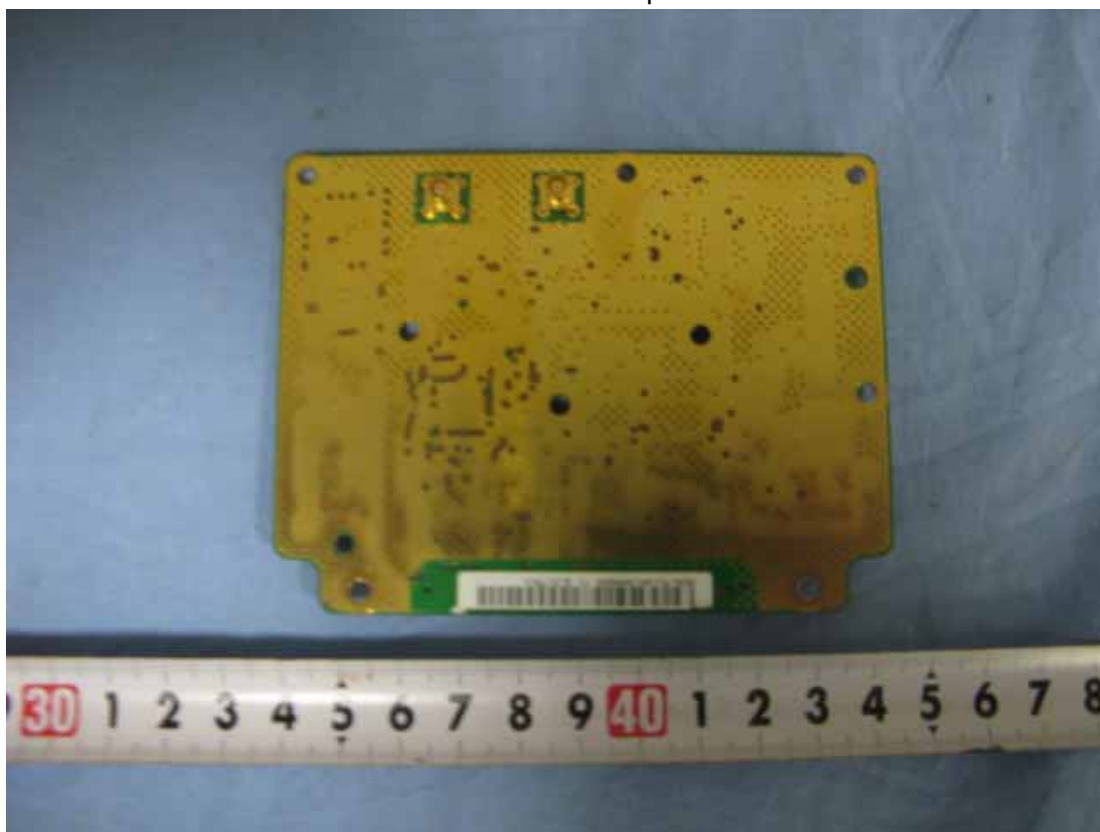
05 View of RF board solder side
