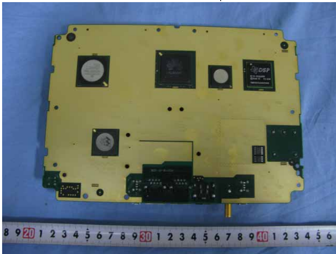
02 View of main board solder side
