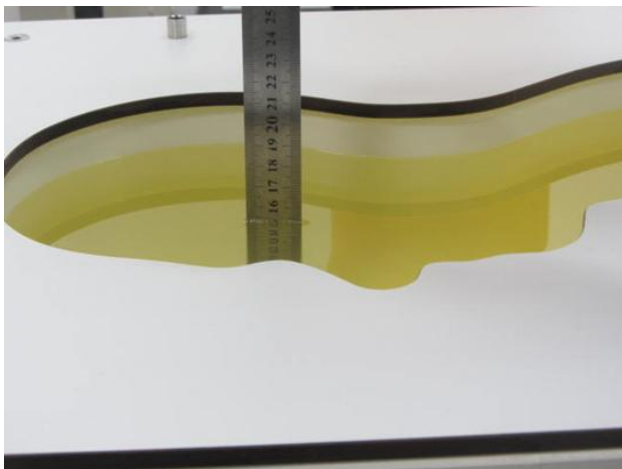
Photo 20: HSL835MHz depth (15.1cm)
