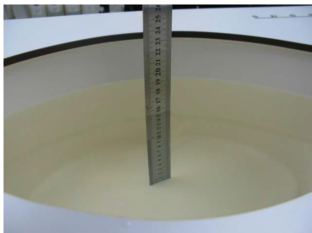
Photo 27: MSL2450MHz depth (15.1cm)
