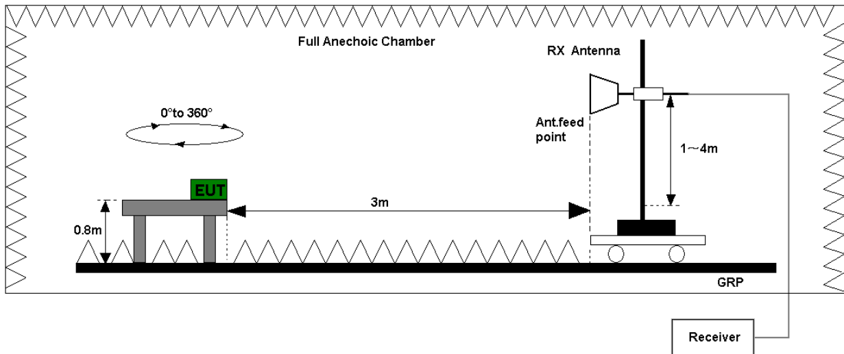
Figure 2. Test set-up of radiated disturbance (above 1GHz) Figure 3.
