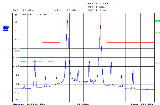
CA_7C 20MHz+10MHz QPSK RB=1#0+1#49 CH- High
