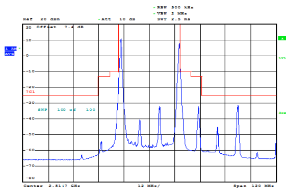
CA_7C 20MHz+10MHz QPSK RB=1#0+1#49 CH- Low
