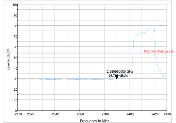
802.11g-Channel 1 Average
