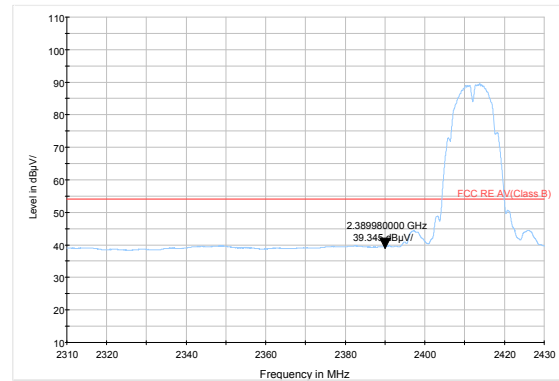
802.11b-Channel 1 Average
