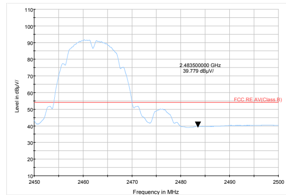
802.11b-Channel 11 Average
