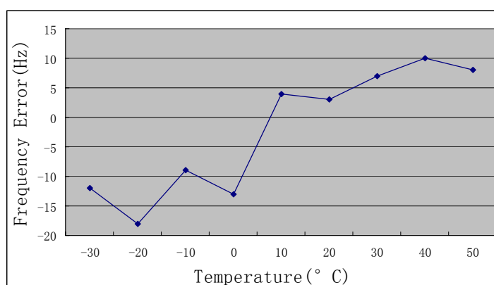
Figure 9. EDGE Mode Test Graph
