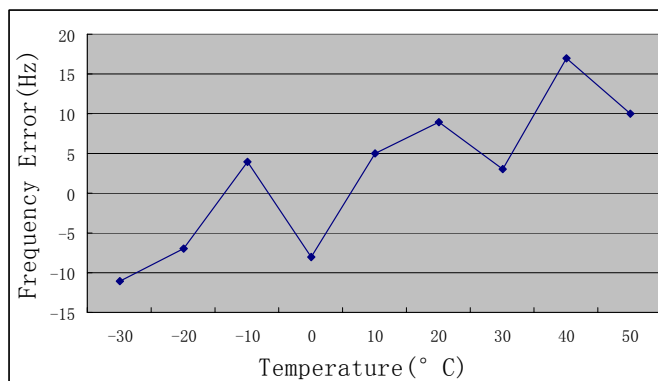
Figure 8. GPRS/GSM Mode Test Graph
