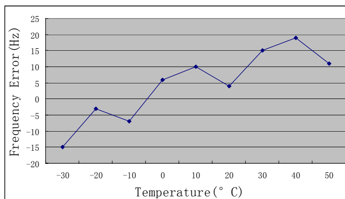
Figure 10. WCDMA Mode Test Graph
