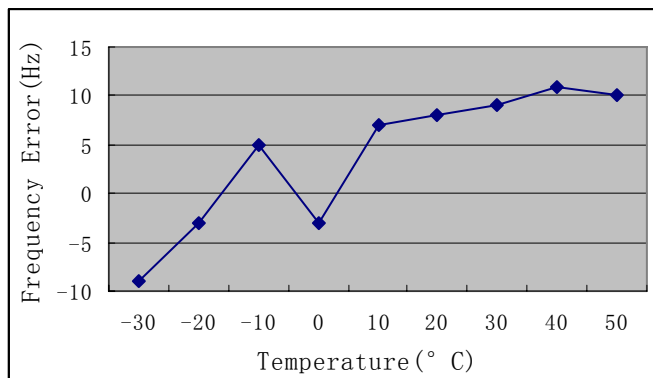
Figure 8. WCDMA Mode Test Graph
