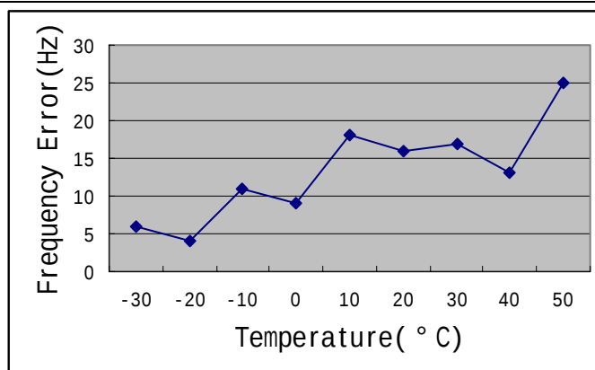
Figure 10. TM3 Test Graph
