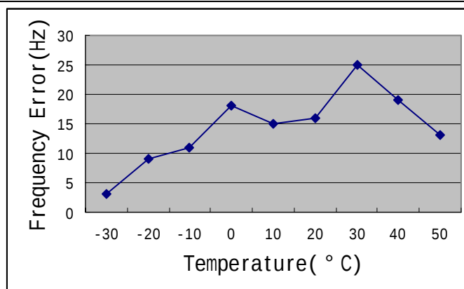
Figure 9. TM2 Test Graph
