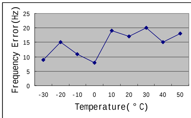
Figure 8. TM1 Test Graph
