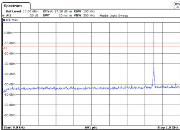
GSM 850 CH-High 9KHz ~ 1GHz
