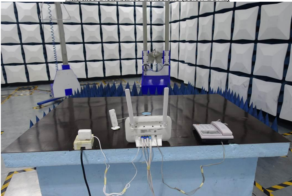
Radiated Disturbance Emissions (1GHz to18GHz)
