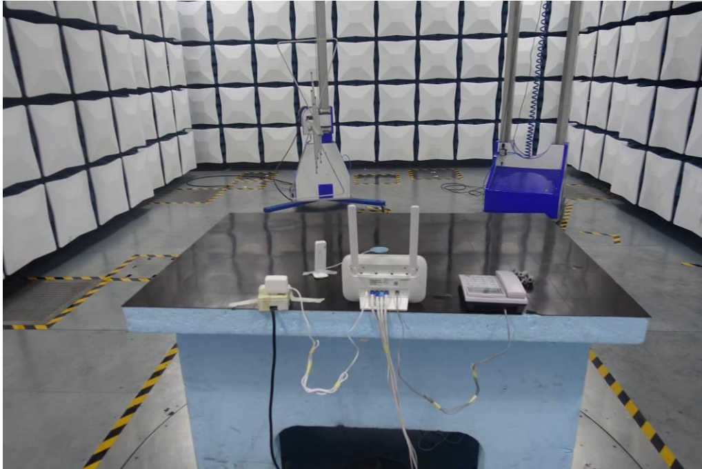
Radiated Disturbance Emissions (below 1GHz)
