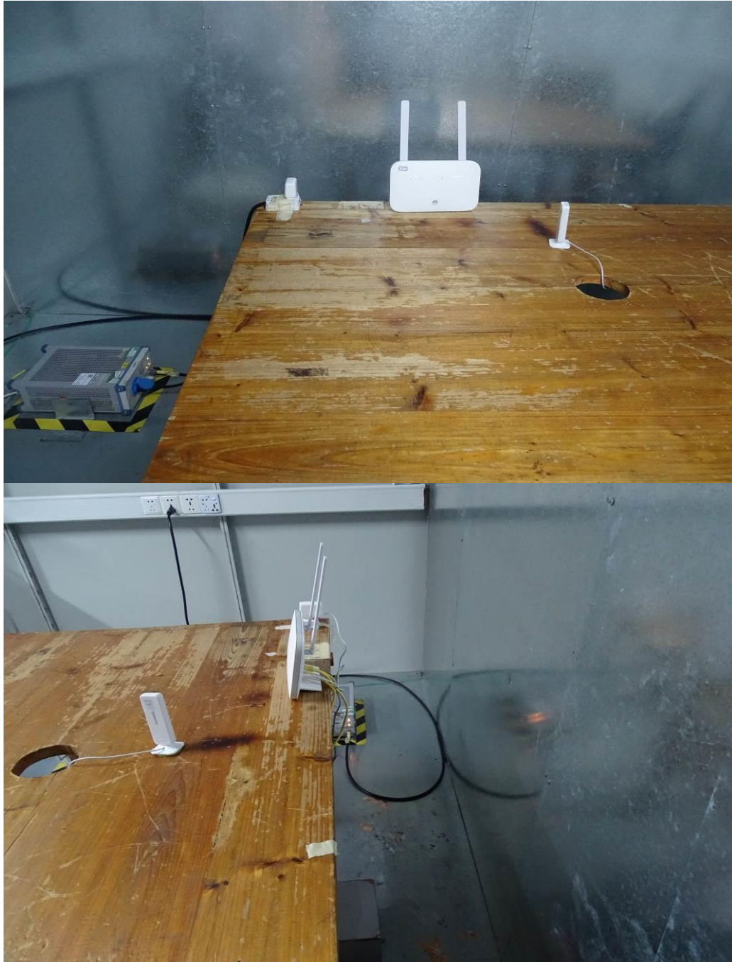
Conducted Emissions with AC Ports
