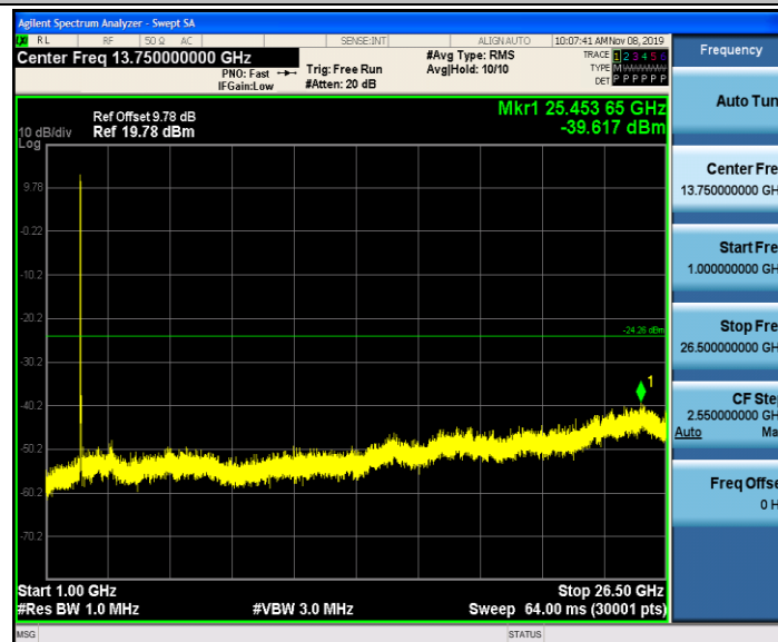
11G-CDD_Ant2_2412_0~Reference
