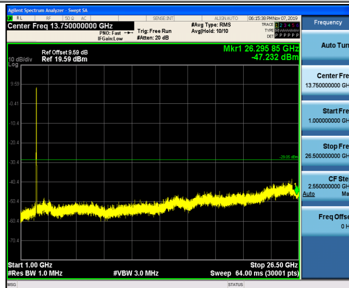
11G-CDD_Ant1_2412_0~Reference
