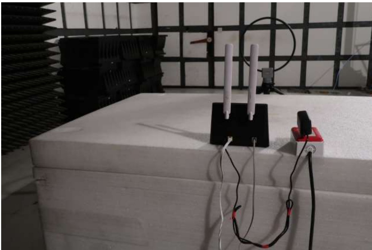
Radiated Spurious Emission (9K-30MHz)
