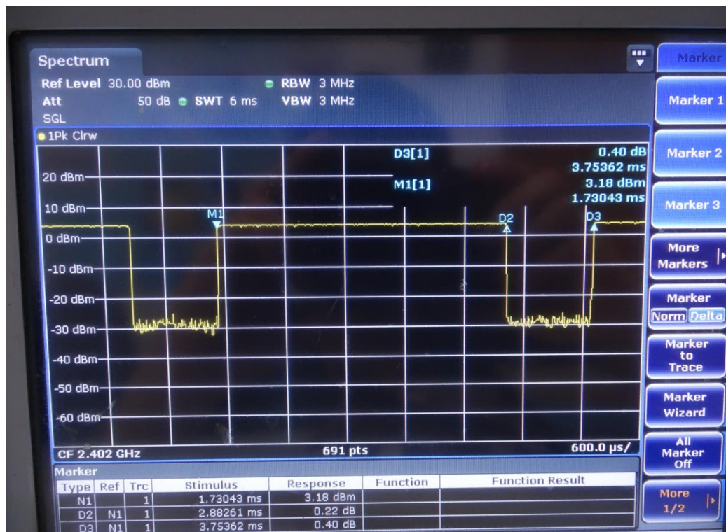
Figure: Bluetooth Transmission Plot
